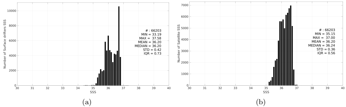
Figure 3: Histograms of SSS from Surface drifters (a) and SMOS SSS L3 v335 - Monthly - 25 km (CATDS-CPDC) (b) considering all match-up pairs per bins of 0.1 over the OTT zone Pi-MEP region and for the full satellite product period.
