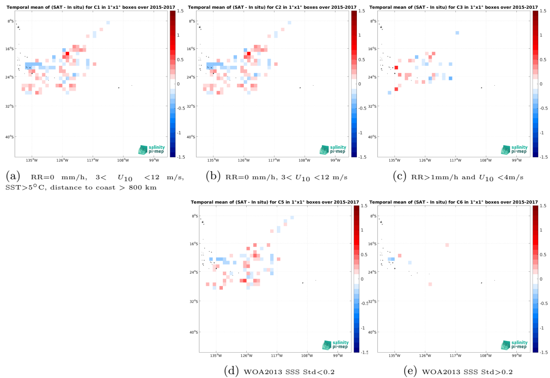
Figure 13: Temporal mean gridded over spatial boxes of size 1^\circ \times 1^\circ of \Delta SSS (SMOS SSS L3 v335 - Monthly - 25 km (CATDS-CPDC) - Surface drifters) for 5 different subdatasets corresponding to:RR=0 mm/h, 3 < U_{10} < 12 m/s, SST >5^\circ C, distance to coast > 800 km (a), RR=0 mm/h, 3 < U_{10} < 12 m/s (b), RR >1 mm/h and U_{10} < 4 m/s (c), WOA2013 SSS Std <0.2 (d), WOA2013 SSS Std >0.2 (e).
