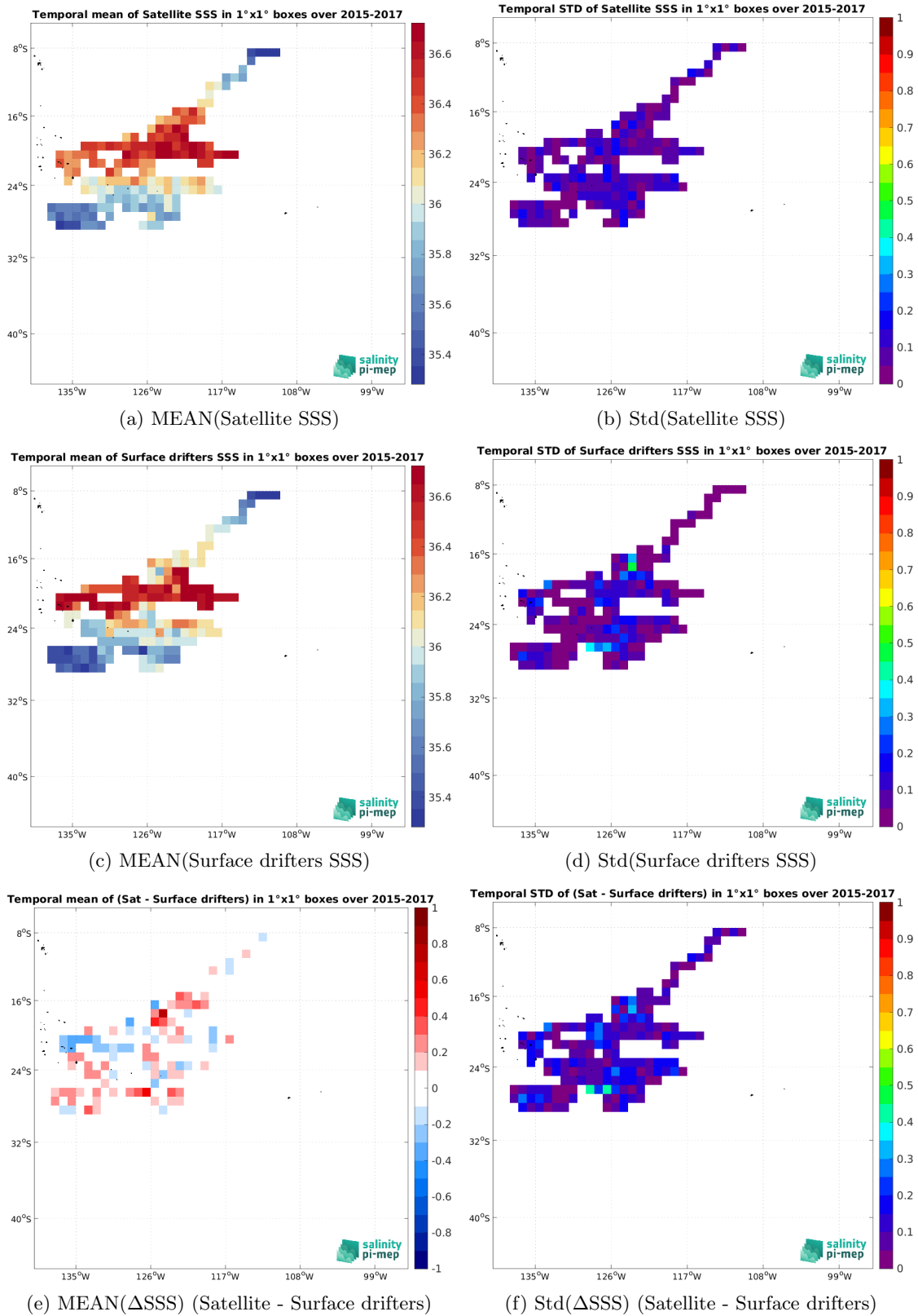
Figure 6: Temporal mean (left) and Std (right) of SSS from SMOS SSS L3 v335 - Monthly - 25 km (CATDS-CPDC) (top), Surface drifters (middle), and of \Delta SSS (Satellite - Surface drifters). Only match-up pairs are used to generate these maps.
