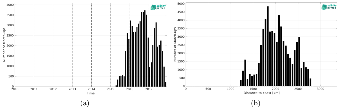
Figure 2: Number of match-ups between Surface drifters and SMOS SSS L3 v335 - Monthly - 25 km (CATDS-CPDC) SSS as a function of time (a) and as function of the distance to coast (b) over the OTT zone Pi-MEP region and for the full satellite product period.
