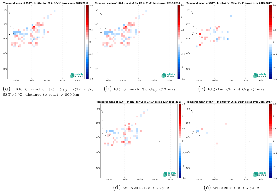
Figure 13: Temporal mean gridded over spatial boxes of size 1^\circ \times 1^\circ of \Delta SSS (SMOS SSS L3 v335 - Monthly - 25 km (CATDS-CPDC) - Surface drifters) for 5 different subdatasets corresponding to:RR=0 mm/h, 3 < U_{10} < 12 m/s, SST >5^\circ C, distance to coast > 800 km (a), RR=0 mm/h, 3 < U_{10} < 12 m/s (b), RR >1 mm/h and U_{10} < 4 m/s (c), WOA2013 SSS Std <0.2 (d), WOA2013 SSS Std >0.2 (e).
