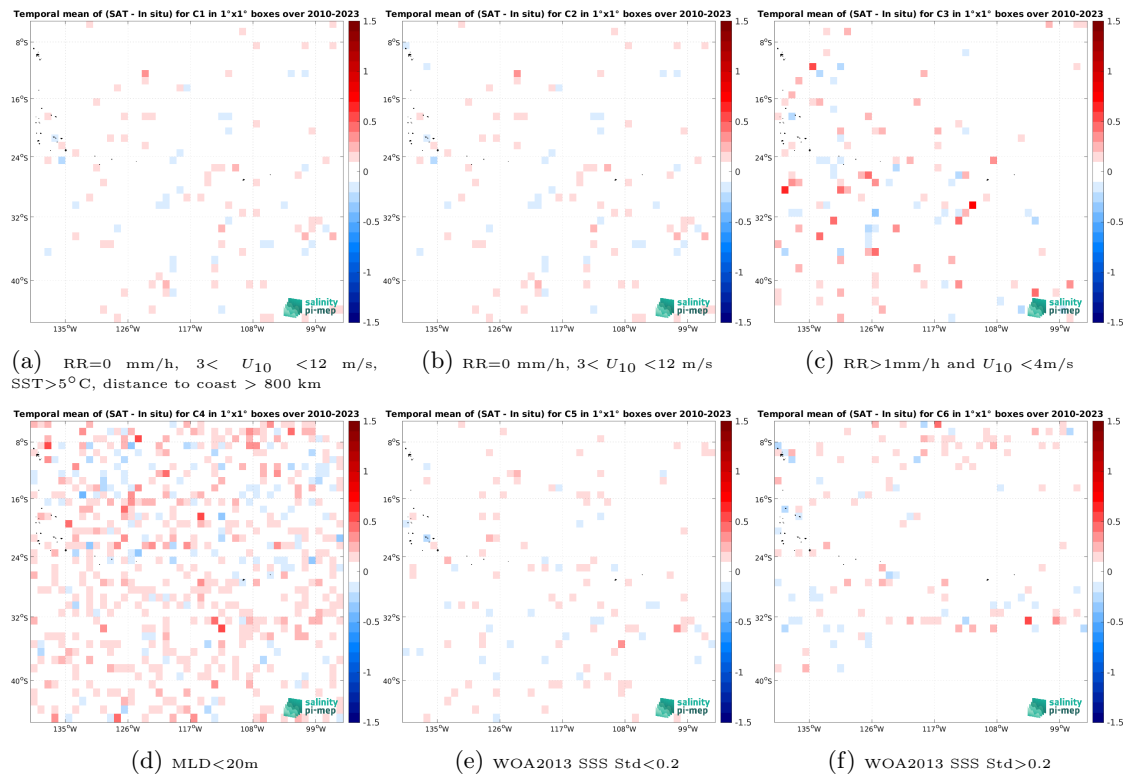
Figure 12: Temporal mean gridded over spatial boxes of size 1^\circ \times 1^\circ of \Delta SSS (SMOS SSS L3 v335 - Monthly - 25 km (CATDS-CPDC) - Argo) for 6 different subdatasets corresponding to:RR=0 mm/h, 3 < U_{10} < 12 m/s, SST >5^\circ C, distance to coast > 800 km (a), RR=0 mm/h, 3 < U_{10} < 12 m/s (b), RR >1 mm/h and U_{10} < 4 m/s (c),MLD <20 m (d),WOA2013 SSS Std <0.2 (e),WOA2013 SSS Std >0.2 (f).
