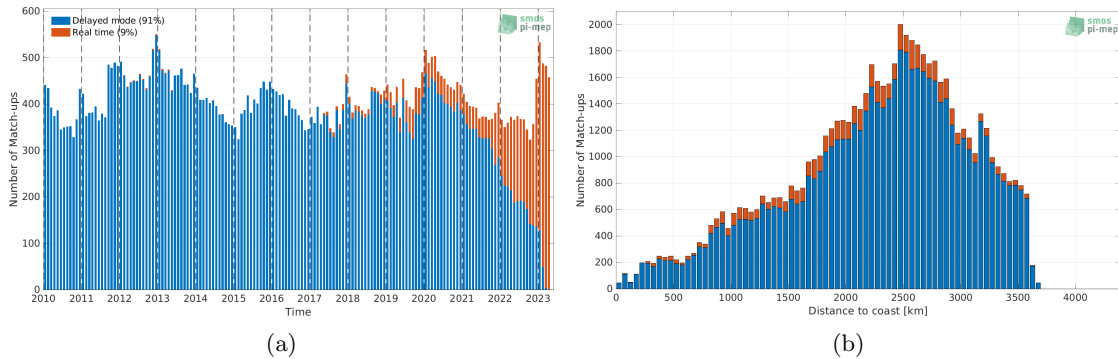
Figure 1: Number of match-ups between Argo and SMOS SSS L3 v335 - Monthly - 25 km (CATDS-CPDC) SSS as a function of time (a) and as function of the distance to coast (b) over the OTT zone Pi-MEP region and for the full satellite product period.
