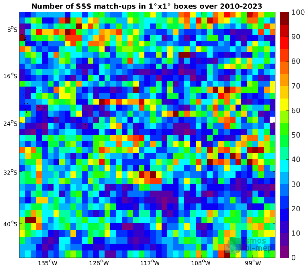
Figure 4: Number of SSS match-ups between Argo SSS and the SMOS SSS L3 v335 - Monthly - 25 km (CATDS-CPDC) SSS product for the OTT zone Pi-MEP region over 1°x1° boxes and for the full satellite product period.
