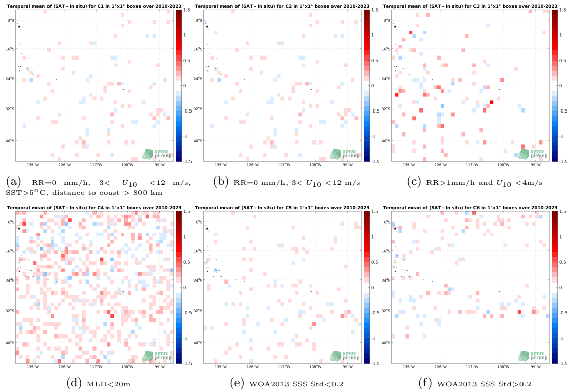
Figure 12: Temporal mean gridded over spatial boxes of size 1^\circ \times 1^\circ of \Delta SSS (SMOS SSS L3 v335 - Monthly - 25 km (CATDS-CPDC) - Argo) for 6 different subdatasets corresponding to:RR=0 mm/h, 3 < U_{10} < 12 m/s, SST >5^\circ C, distance to coast > 800 km (a), RR=0 mm/h, 3 < U_{10} < 12 m/s (b), RR >1 mm/h and U_{10} < 4 m/s (c),MLD <20 m (d),WOA2013 SSS Std <0.2 (e),WOA2013 SSS Std >0.2 (f).
