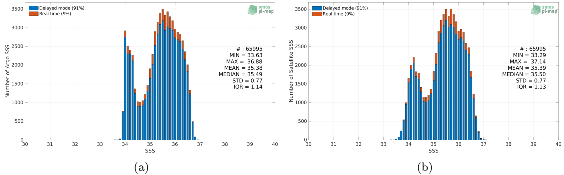
Figure 2: Histograms of SSS from Argo (a) and SMOS SSS L3 v335 - Monthly - 25 km (CATDS-CPDC) (b) considering all match-up pairs per bins of 0.1 over the OTT zone Pi-MEP region and for the full satellite product period.
