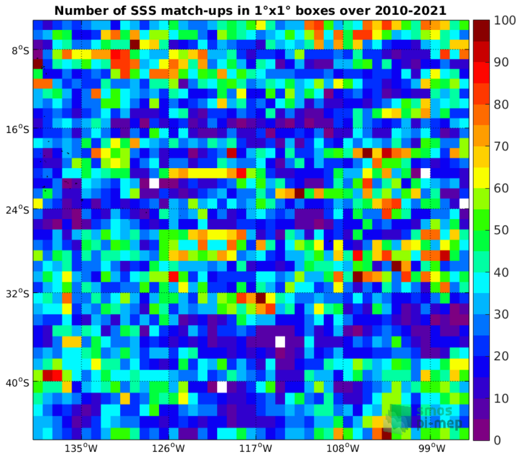
Figure 4: Number of SSS match-ups between Argo SSS and the SMOS SSS L3 v335 - Monthly - 25 km (CATDS-CPDC) SSS product for the OTT zone Pi-MEP region over 1^\circ \times 1^\circ boxes and for the full satellite product period.
