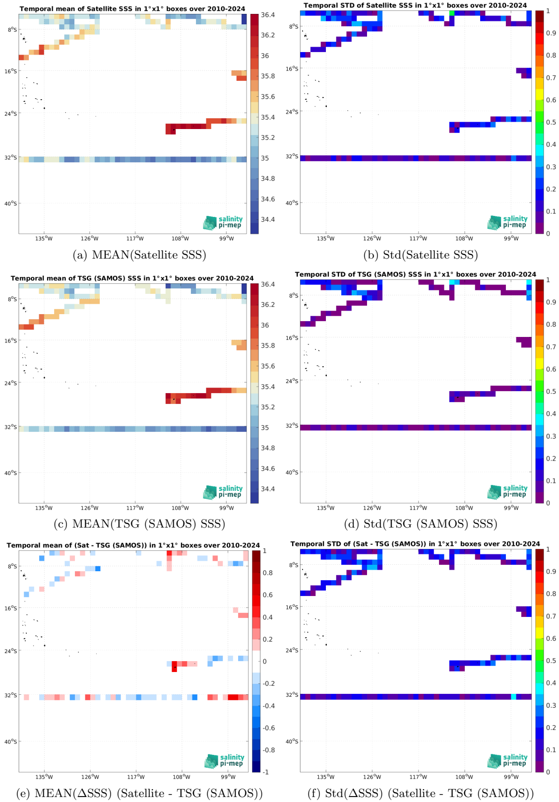
Figure 7: Temporal mean (left) and Std (right) of SSS from SMOS SSS L3 v335 - 10 Days - 25 km (CATDS-CPDC) (top), TSG (SAMOS) (middle), and of \Delta SSS (Satellite - TSG (SAMOS)). Only match-up pairs are used to generate these maps.
