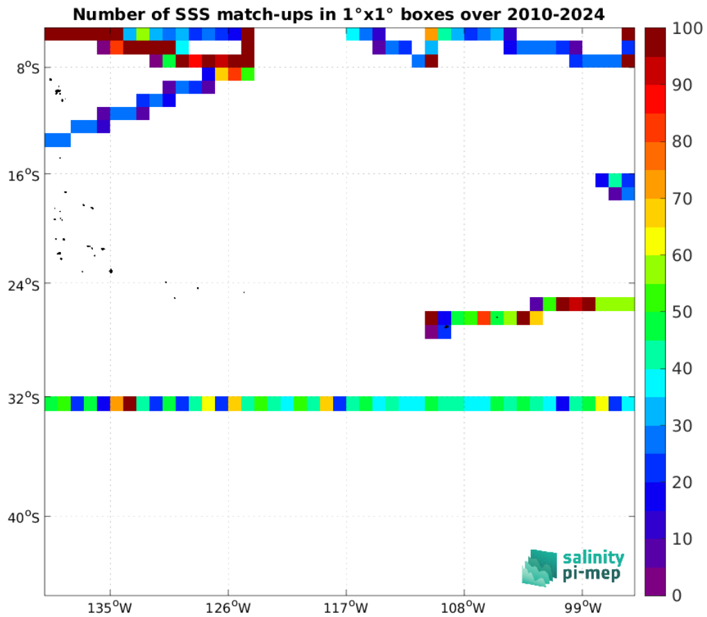
Figure 5: Number of SSS match-ups between TSG (SAMOS) SSS and the SMOS SSS L3 v335 - 10 Days - 25 km (CATDS-CPDC) SSS product for the OTT zone Pi-MEP region over 1^\circ \times 1^\circ boxes and for the full satellite product period.
