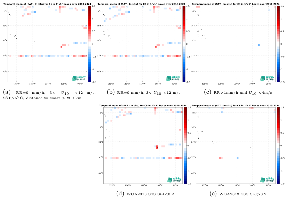
Figure 14: Temporal mean gridded over spatial boxes of size 1^\circ \times 1^\circ of \Delta SSS (SMOS SSS L3 v335 - 10 Days - 25 km (CATDS-CPDC) - TSG (SAMOS)) for 5 different subdatasets corresponding to: RR=0 mm/h, 3 < U_{10} < 12 m/s, SST > 5^\circ C , distance to coast > 800 km (a), RR=0 mm/h, 3 < U_{10} < 12 m/s (b), RR > 1 mm/h and U_{10} < 4 m/s (c), WOA2013 SSS Std < 0.2 (d), WOA2013 SSS Std > 0.2 (e).
