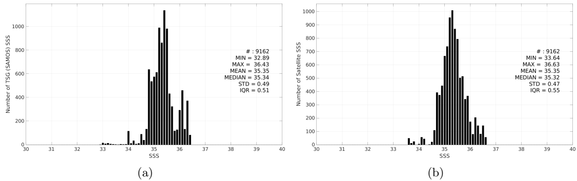
Figure 3: Histograms of SSS from TSG (SAMOS) (a) and SMOS SSS L3 v335 - 10 Days - 25 km (CATDS-CPDC) (b) considering all match-up pairs per bins of 0.1 over the OTT zone Pi-MEP region and for the full satellite product period.
