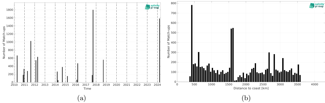
Figure 2: Number of match-ups between TSG (SAMOS) and SMOS SSS L3 v335 - 10 Days - 25 km (CATDS-CPDC) SSS as a function of time (a) and as function of the distance to coast (b) over the OTT zone Pi-MEP region and for the full satellite product period.
