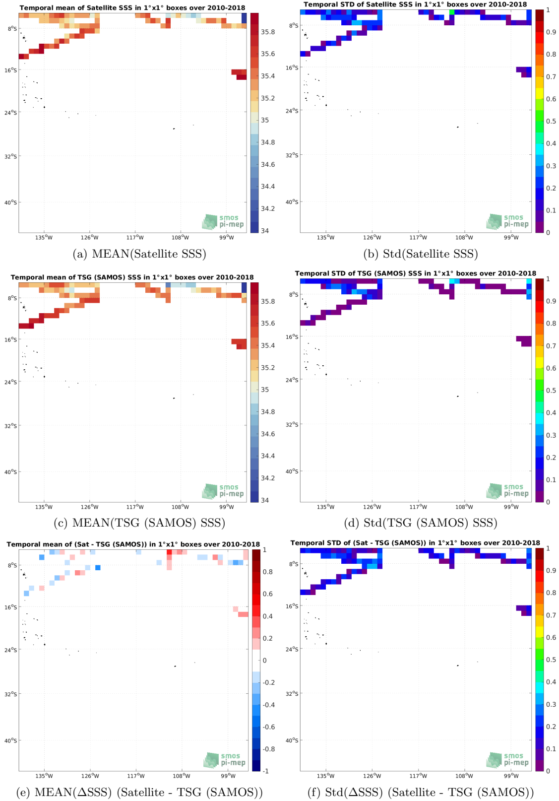
Figure 6: Temporal mean (left) and Std (right), of SSS from SMOS SSS L3 v335 - 10 Days - 25 km (CATDS-CPDC) (top), TSG (SAMOS) (middle), and of \Delta SSS (Satellite - TSG (SAMOS)). Only match-up pairs are used to generate these maps.
