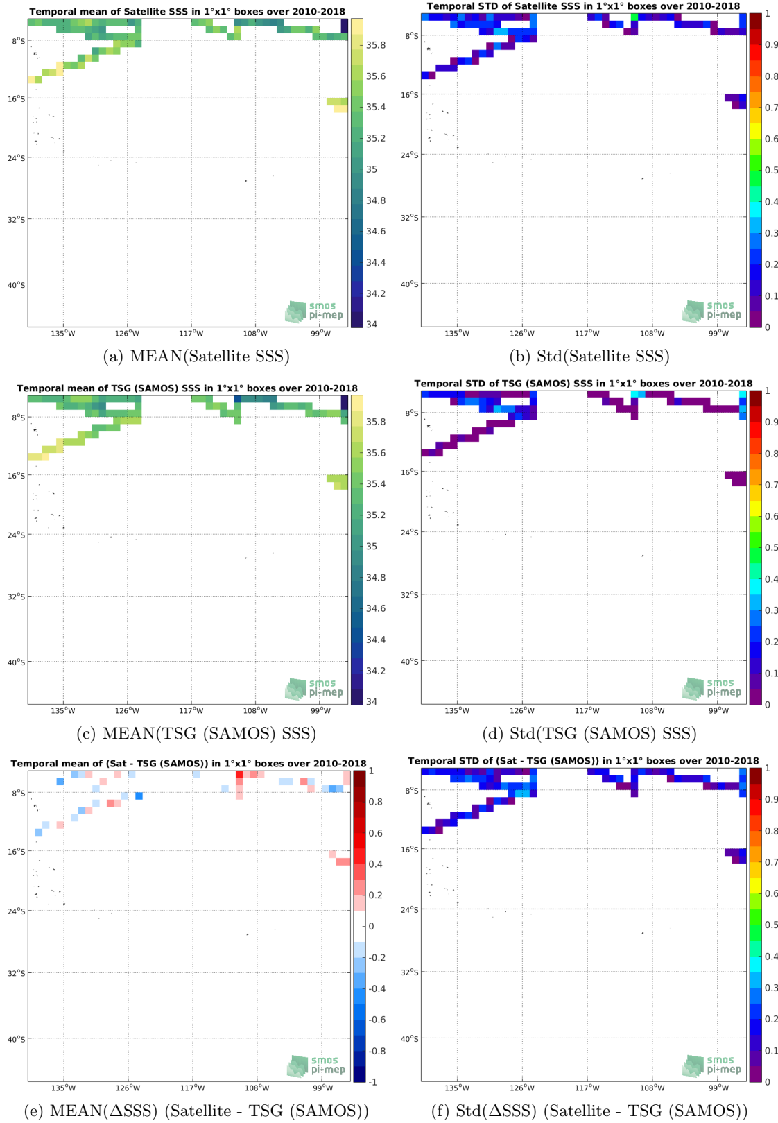
Figure 6: Temporal mean (left) and Std (right) of SSS from SMOS SSS L3 v335 - 10 Days - 25 km (CATDS-CPDC) (top), TSG (SAMOS) (middle), and of \Delta SSS (Satellite - TSG (SAMOS)). Only match-up pairs are used to generate these maps.
