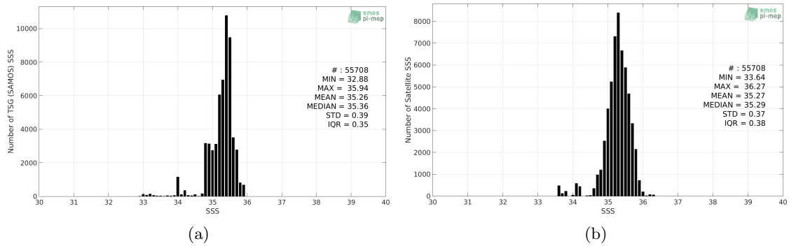
Figure 2: Histograms of SSS from TSG (SAMOS) (a) and SMOS SSS L3 v335 - 10 Days - 25 km (CATDS-CPDC) (b) considering all match-up pairs per bins of 0.1 over the OTT zone Pi-MEP region and for the full satellite product period.
