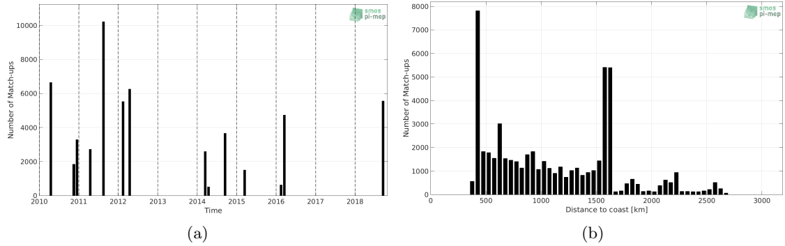
Figure 1: Number of match-ups between TSG (SAMOS) and SMOS SSS L3 v335 - 10 Days - 25 km (CATDS-CPDC) SSS as a function of time (a) and as function of the distance to coast (b) over the OTT zone Pi-MEP region and for the full satellite product period.
