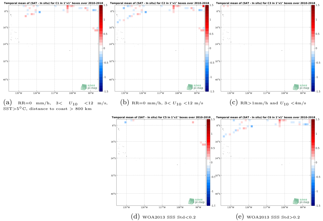
Figure 12: Temporal mean gridded over spatial boxes of size 1^\circ \times 1^\circ of \Delta SSS (SMOS SSS L3 v335 - 10 Days - 25 km (CATDS-CPDC) - TSG (SAMOS)) for 5 different subdatasets corresponding to: RR=0 mm/h, 3 < U_{10} < 12 m/s, SST > 5^\circ C , distance to coast > 800 km (a), RR=0 mm/h, 3 < U_{10} < 12 m/s (b), RR > 1 mm/h and U_{10} < 4 m/s (c), WOA2013 SSS Std < 0.2 (d), WOA2013 SSS Std > 0.2 (e).
