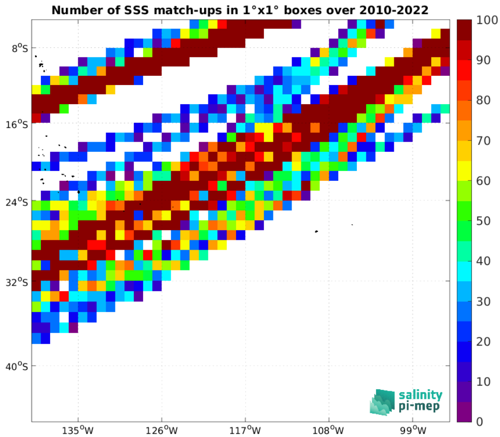
Figure 5: Number of SSS match-ups between TSG (LEGOS-DM) SSS and the SMOS SSS L3 v335 - 10 Days - 25 km (CATDS-CPDC) SSS product for the OTT zone Pi-MEP region over 1°x1° boxes and for the full satellite product period.
