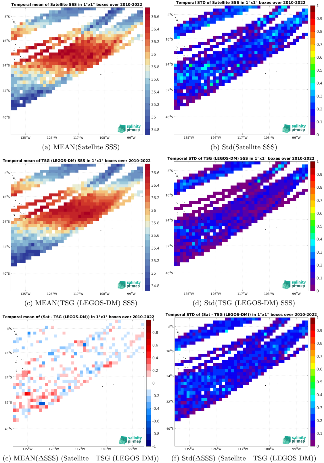
(e) MEAN( \Delta SSS) (Satellite - TSG (LEGOS-DM)) (f) Std( \Delta SSS) (Satellite - TSG (LEGOS-DM)) Figure 7: Temporal mean (left) and Std (right) of SSS from SMOS SSS L3 v335 - 10 Days - 25 km (CATDS-CPDC) (top), TSG (LEGOS-DM) (middle), and of \Delta SSS (Satellite - TSG (LEGOS-DM)). Only match-up pairs are used to generate these maps.
