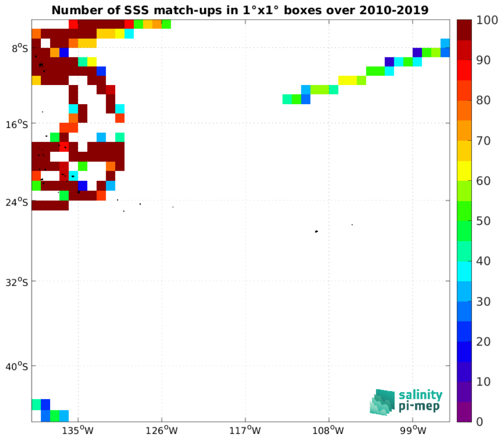
Figure 5: Number of SSS match-ups between TSG (GOSUD-Research-vessel) SSS and the SMOS SSS L3 v335 - 10 Days - 25 km (CATDS-CPDC) SSS product for the OTT zone Pi-MEP region over 1^\circ \times 1^\circ boxes and for the full satellite product period.
