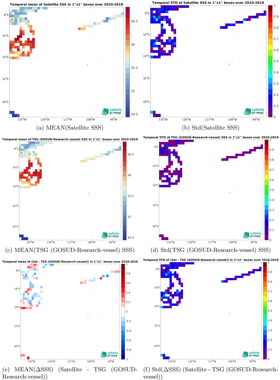
Figure 7: Temporal mean (left) and Std (right) of SSS from SMOS SSS L3 v335 - 10 Days - 25 km (CATDS-CPDC) (top), TSG (GOSUD-Research-vessel) (middle), and of \Delta SSS (Satellite - TSG (GOSUD-Research-vessel)). Only match-up pairs are used to generate these maps.
