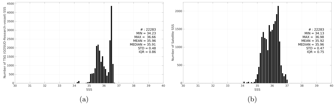
Figure 3: Histograms of SSS from TSG (GOSUD-Research-vessel) (a) and SMOS SSS L3 v335 - 10 Days - 25 km (CATDS-CPDC) (b) considering all match-up pairs per bins of 0.1 over the OTT zone Pi-MEP region and for the full satellite product period.
