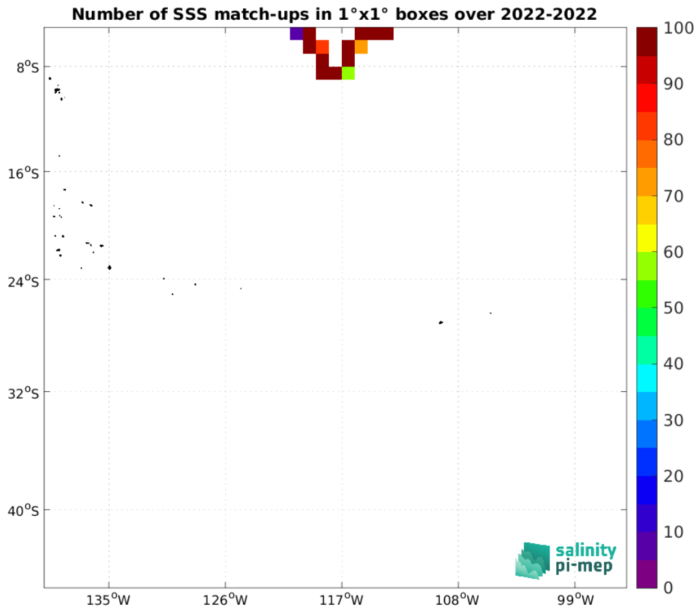
Figure 4: Number of SSS match-ups between Saildrone SSS and the SMOS SSS L3 v335 - 10 Days - 25 km (CATDS-CPDC) SSS product for the OTT zone Pi-MEP region over 1°x1° boxes and for the full satellite product period.
