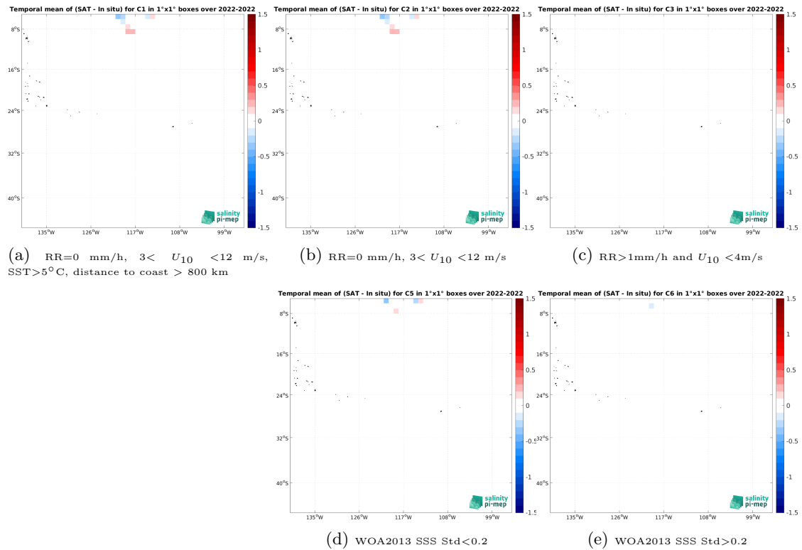
Figure 12: Temporal mean gridded over spatial boxes of size 1^\circ \times 1^\circ of \Delta SSS (SMOS SSS L3 v335 - 10 Days - 25 km (CATDS-CPDC) - Saildrone) for 5 different subdatasets corresponding to: RR=0 mm/h, 3 < U_{10} < 12 m/s, SST > 5^\circ C , distance to coast > 800 km (a), RR=0 mm/h, 3 < U_{10} < 12 m/s (b), RR > 1 mm/h and U_{10} < 4 m/s (c), WOA2013 SSS Std < 0.2 (d), WOA2013 SSS Std > 0.2 (e).
