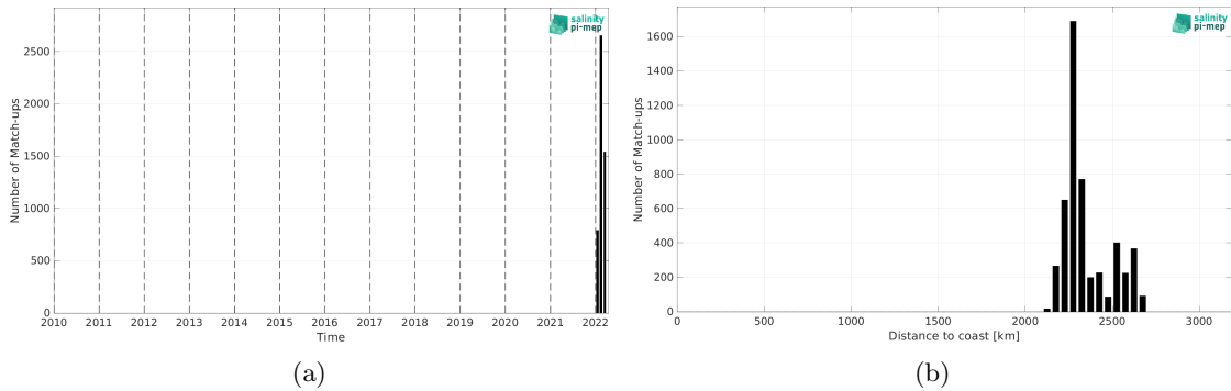
Figure 1: Number of match-ups between Saildrone and SMOS SSS L3 v335 - 10 Days - 25 km (CATDS-CPDC) SSS as a function of time (a) and as function of the distance to coast (b) over the OTT zone Pi-MEP region and for the full satellite product period.
