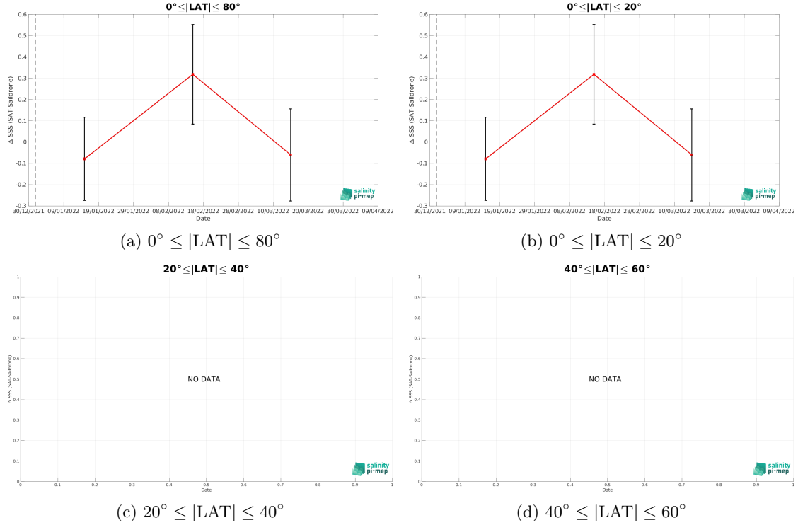
Figure 10: Monthly median (red curves) of \Delta\text{SSS} (Satellite - Saldrone) and \pm 1 Std (black vertical thick bars) as function of time for all the collected Pi-MEP match-up pairs estimated over the OTT zone Pi-MEP region and for the full satellite product period are shown for different latitude bands: (a) 80°S-80°N, (b) 20°S-20°N, (c) 40°S-20°S and 20°N-40°N and (d) 60°S-40°S and 40°N-60°N.
