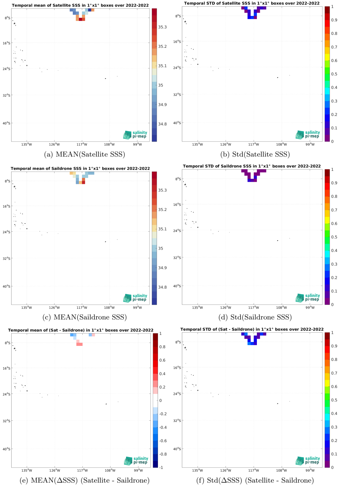
Figure 6: Temporal mean (left) and Std (right) of SSS from SMOS SSS L3 v335 - 10 Days - 25 km (CATDS-CPDC) (top), Saildrone (middle), and of \Delta SSS (Satellite - Saildrone). Only match-up pairs are used to generate these maps.
