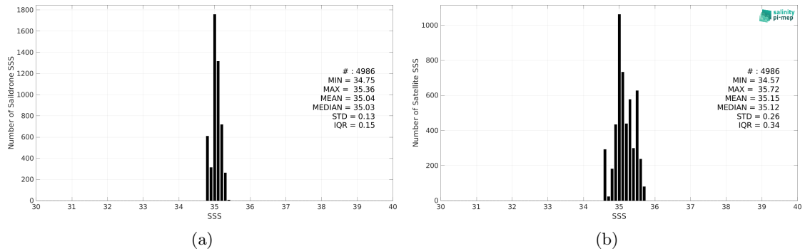
Figure 2: Histograms of SSS from Sailldrone (a) and SMOS SSS L3 v335 - 10 Days - 25 km (CATDS-CPDC) (b) considering all match-up pairs per bins of 0.1 over the OTT zone Pi-MEP region and for the full satellite product period.
