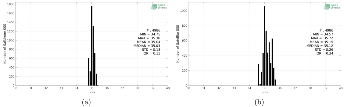
Figure 2: Histograms of SSS from Saildrone (a) and SMOS SSS L3 v335 - 10 Days - 25 km (CATDS-CPDC) (b) considering all match-up pairs per bins of 0.1 over the OTT zone Pi-MEP region and for the full satellite product period.
