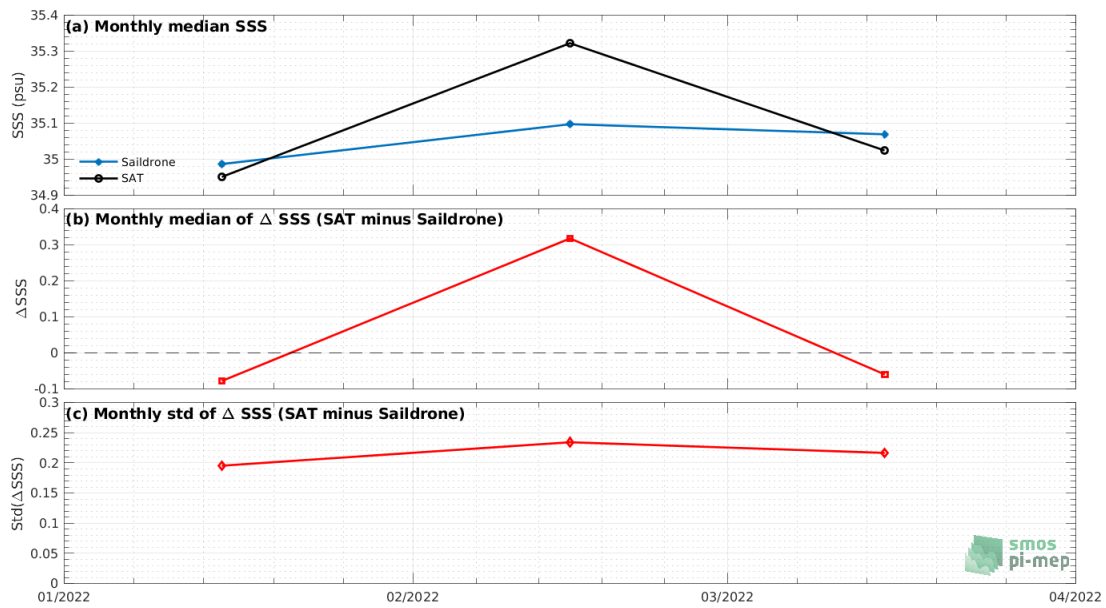
Figure 7: Time series of the monthly median SSS (top), median of \Delta SSS (Satellite - Sailldrone) and Std of \Delta SSS (Satellite - Sailldrone) over the OTT zone Pi-MEP region considering all match-ups collected by the Pi-MEP.
