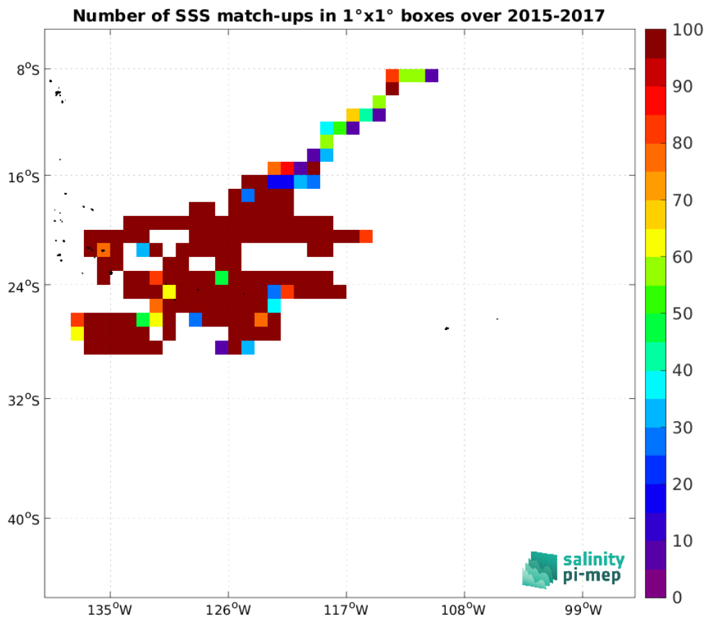
Figure 3: Number of SSS match-ups between Surface drifters SSS and the SMOS SSS L3 v335 - 10 Days - 25 km (CATDS-CPDC) SSS product for the OTT zone Pi-MEP region over 1°x1° boxes and for the full satellite product period.
