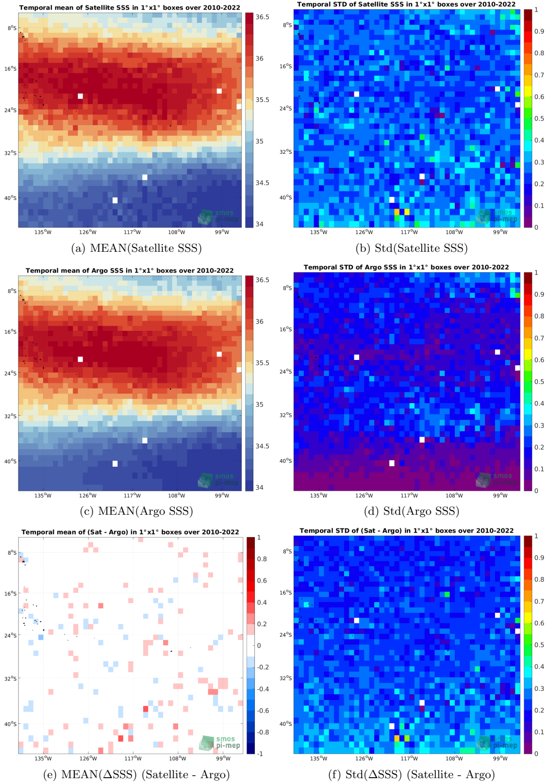
Figure 6: Temporal mean (left) and Std (right), of SSS from SMOS SSS L3 v335 - 10 Days - 25 km (CATDS-CPDC) (top), Argo (middle), and of \Delta SSS (Satellite - Argo). Only match-up pairs are used to generate these maps.
