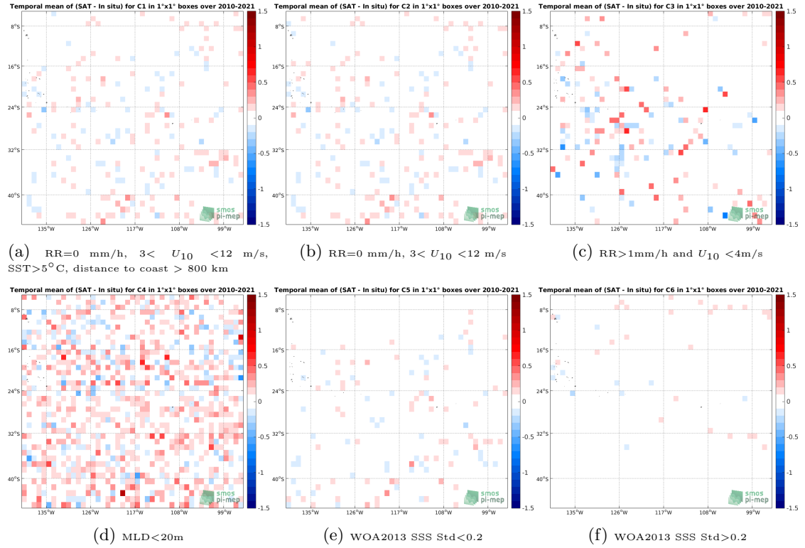
Figure 12: Temporal mean gridded over spatial boxes of size 1^\circ \times 1^\circ of \Delta SSS (SMOS SSS L3 v335 - 10 Days - 25 km (CATDS-CPDC) - Argo) for 6 different subdatasets corresponding to: RR=0 mm/h, 3 < U_{10} < 12 m/s, SST > 5^\circ C , distance to coast > 800 km (a), RR=0 mm/h, 3 < U_{10} < 12 m/s (b), RR > 1 mm/h and U_{10} < 4 m/s (c), MLD < 20 m (d), WOA2013 SSS Std < 0.2 (e), WOA2013 SSS Std > 0.2 (f).
