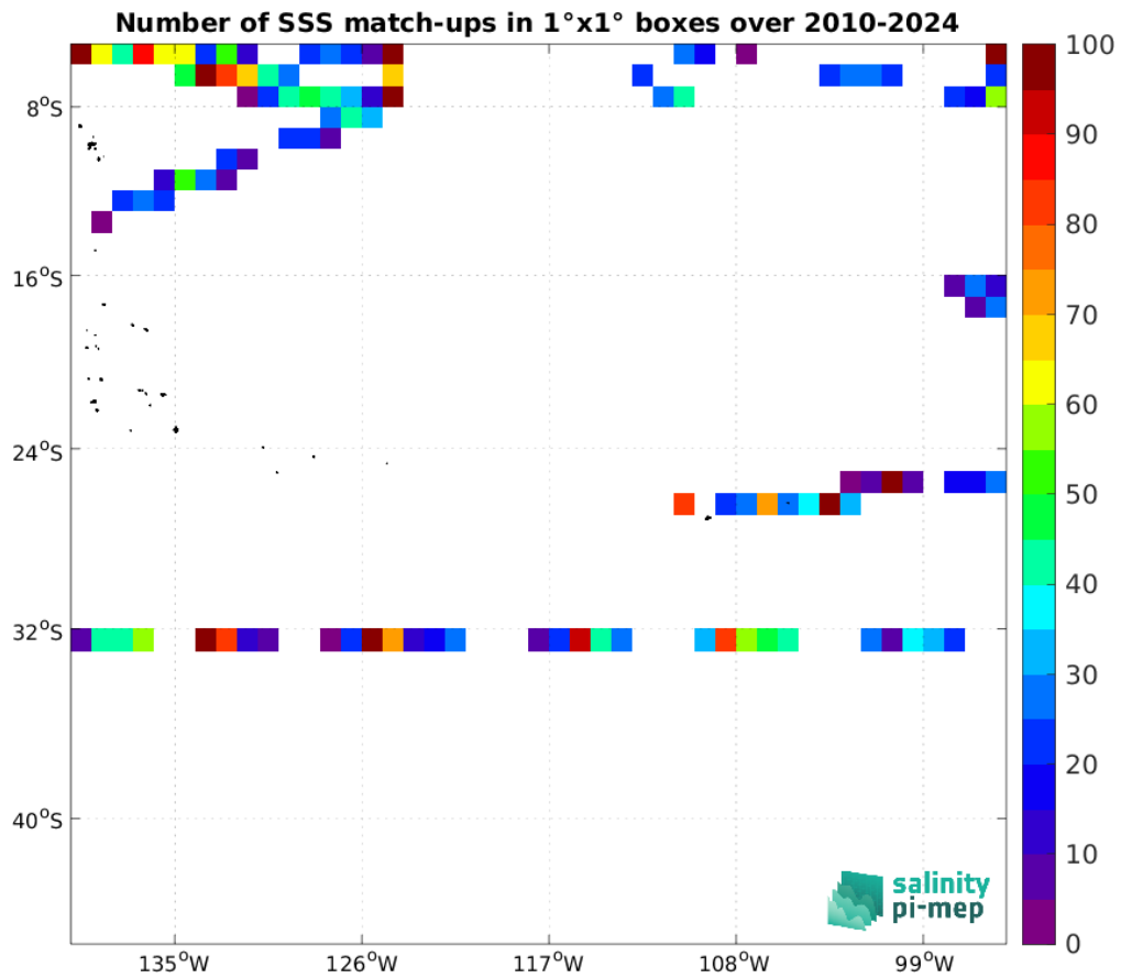
Figure 5: Number of SSS match-ups between TSG (SAMOS) SSS and the SMOS SSS L2Q v333 - 0.25 Deg (CATDS-CPDC) SSS product for the OTT zone Pi-MEP region over 1°x1° boxes and for the full satellite product period.
