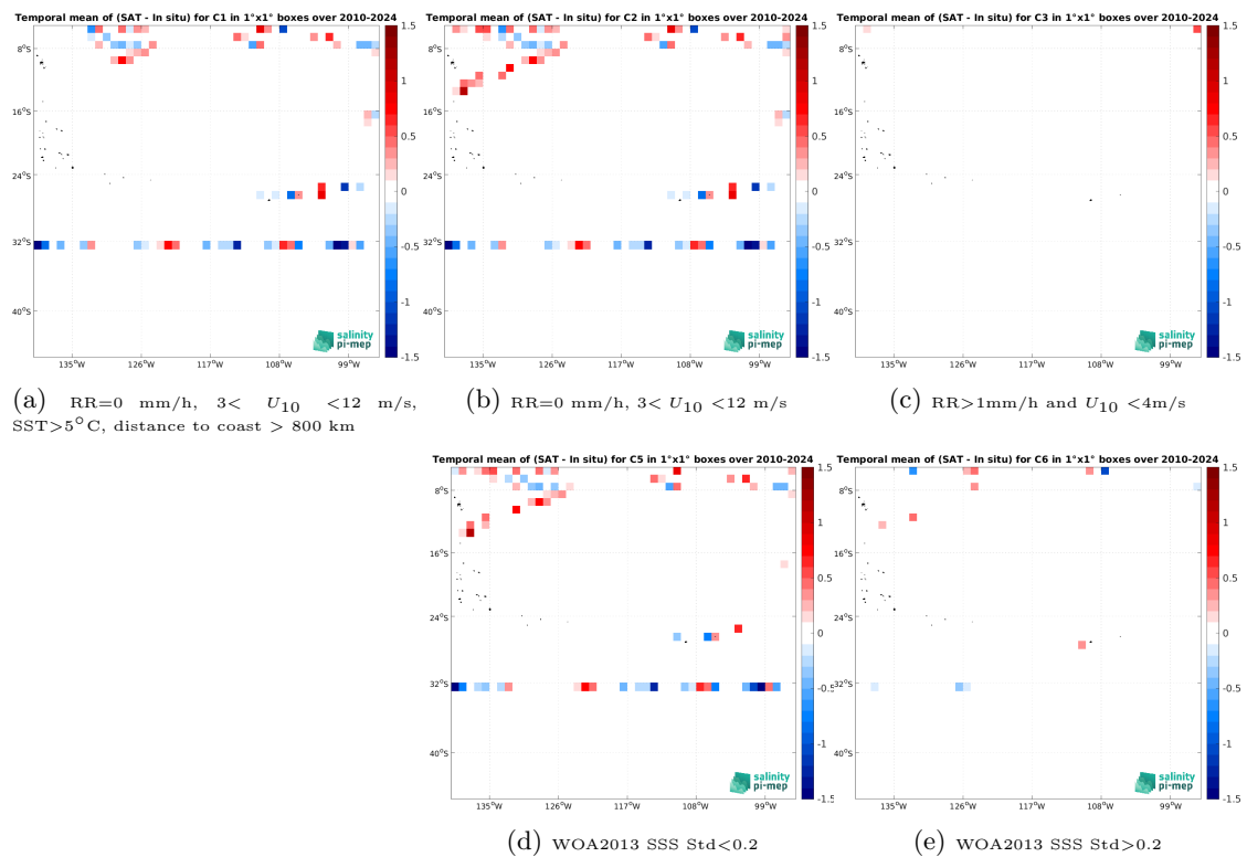
Figure 14: Temporal mean gridded over spatial boxes of size 1^\circ \times 1^\circ of \Delta SSS (SMOS SSS L2Q v333 - 0.25 Deg (CATDS-CPDC) - TSG (SAMOS)) for 5 different subdatasets corresponding to: RR=0 mm/h, 3 < U_{10} < 12 m/s, SST > 5^\circ C , distance to coast > 800 km (a), RR=0 mm/h, 3 < U_{10} < 12 m/s (b), RR > 1 mm/h and U_{10} < 4 m/s (c), WOA2013 SSS Std < 0.2 (d), WOA2013 SSS Std > 0.2 (e).
