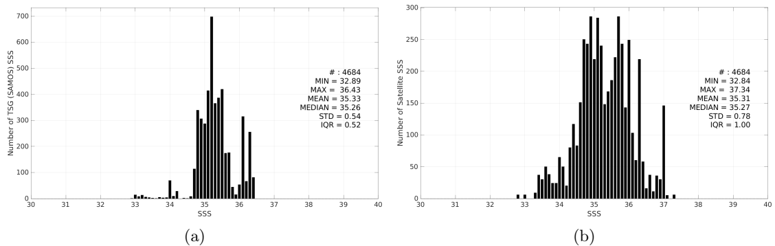
Figure 3: Histograms of SSS from TSG (SAMOS) (a) and SMOS SSS L2Q v333 - 0.25 Deg (CATDS-CPDC) (b) considering all match-up pairs per bins of 0.1 over the OTT zone Pi-MEP region and for the full satellite product period.
