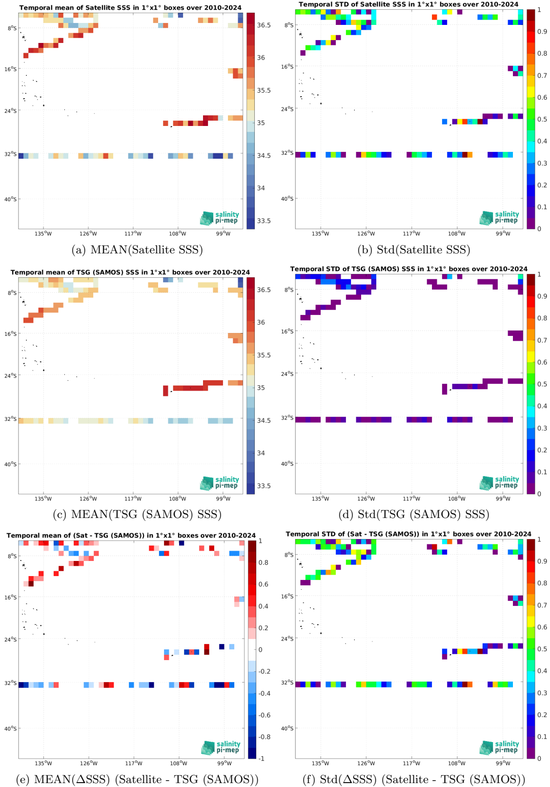
Figure 7: Temporal mean (left) and Std (right) of SSS from SMOS SSS L2Q v333 - 0.25 Deg (CATDS-CPDC) (top), TSG (SAMOS) (middle), and of \Delta SSS (Satellite - TSG (SAMOS)). Only match-up pairs are used to generate these maps.
