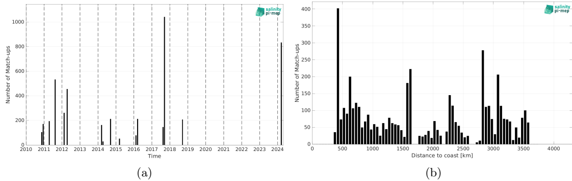
Figure 2: Number of match-ups between TSG (SAMOS) and SMOS SSS L2Q v333 - 0.25 Deg (CATDS-CPDC) SSS as a function of time (a) and as function of the distance to coast (b) over the OTT zone Pi-MEP region and for the full satellite product period.
