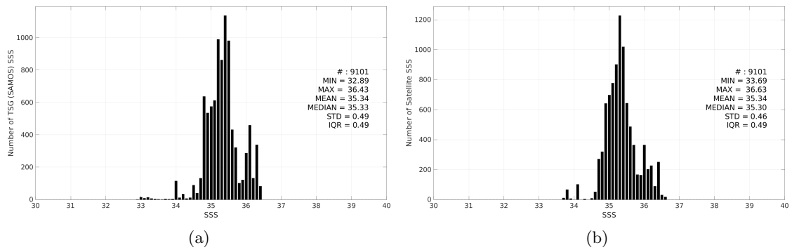
Figure 3: Histograms of SSS from TSG (SAMOS) (a) and SMOS SSS L3 v332 - 9 Days (CATDS-CPDC) (b) considering all match-up pairs per bins of 0.1 over the OTT zone Pi-MEP region and for the full satellite product period.
