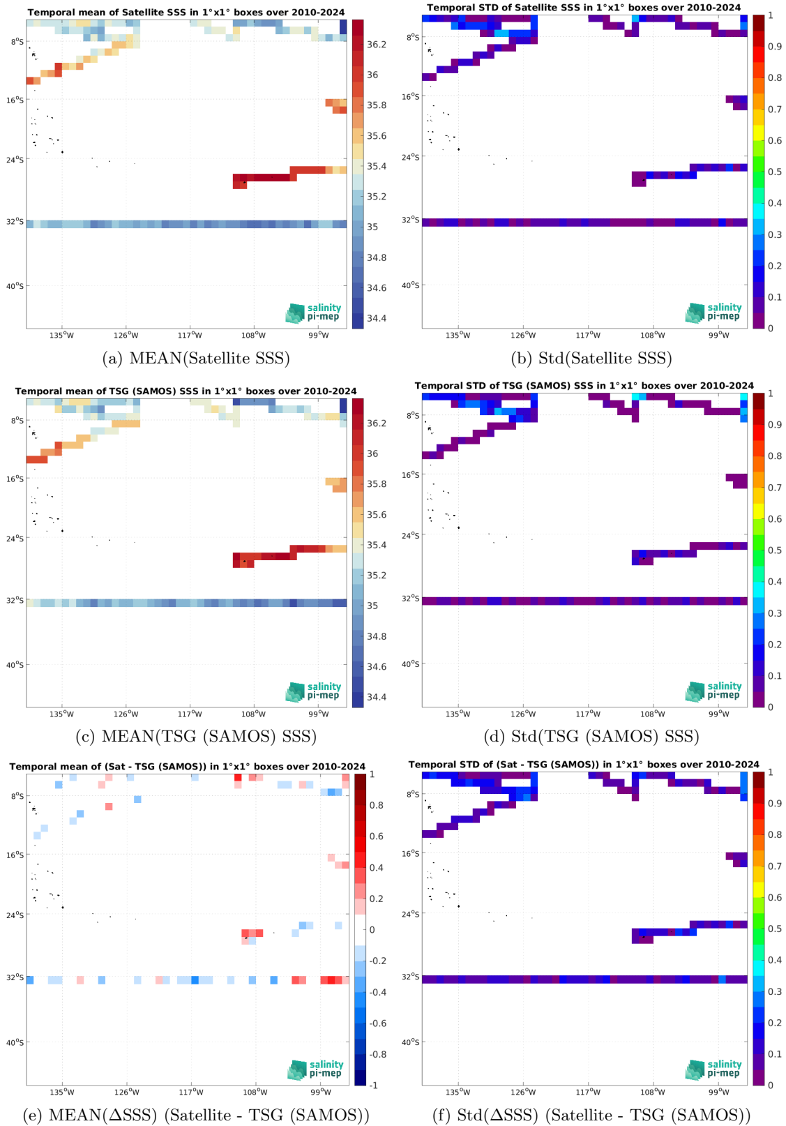
Figure 7: Temporal mean (left) and Std (right) of SSS from SMOS SSS L3 v332 - 9 Days (CATDS-CPDC) (top), TSG (SAMOS) (middle), and of \Delta SSS (Satellite - TSG (SAMOS)). Only match-up pairs are used to generate these maps.
