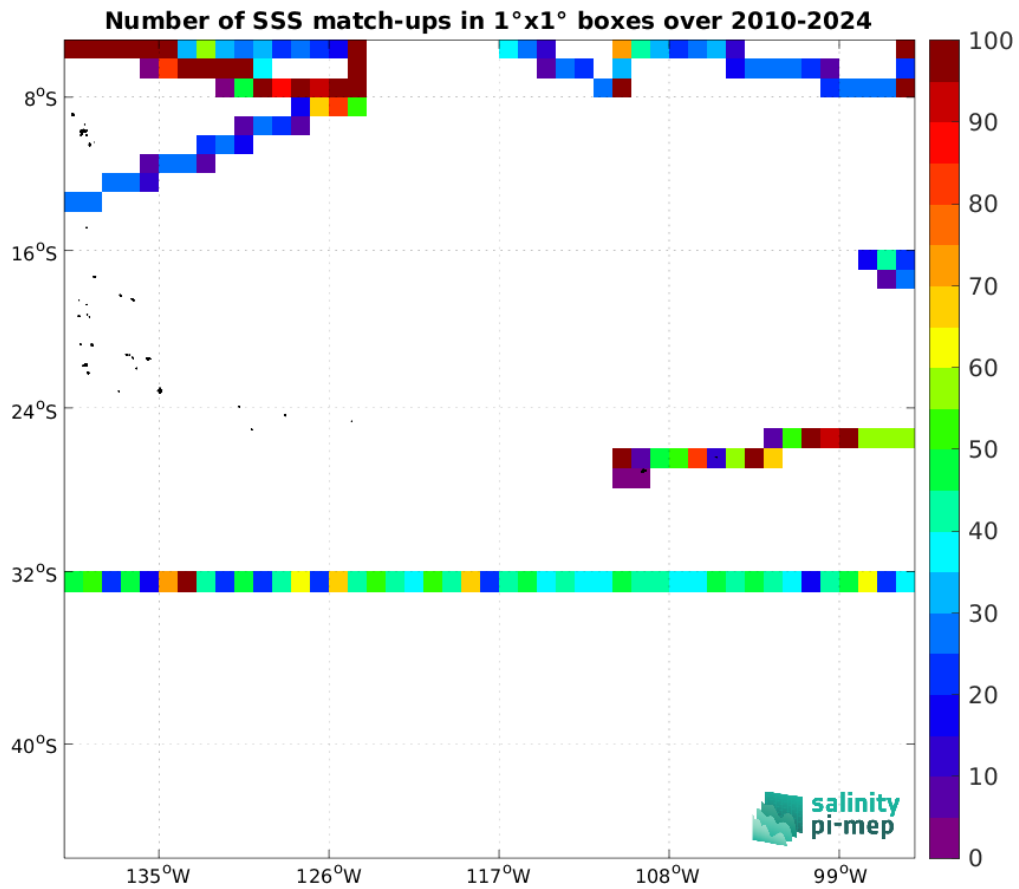
Figure 5: Number of SSS match-ups between TSG (SAMOS) SSS and the SMOS SSS L3 v332 - 9 Days (CATDS-CPDC) SSS product for the OTT zone Pi-MEP region over 1^\circ \times 1^\circ boxes and for the full satellite product period.
