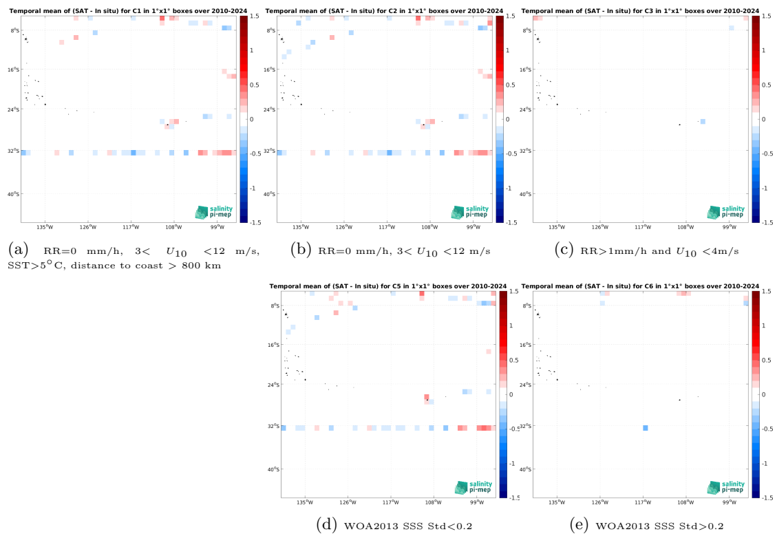
Figure 14: Temporal mean gridded over spatial boxes of size 1^\circ \times 1^\circ of \Delta SSS (SMOS SSS L3 v332 - 9 Days (CATDS-CPDC) - TSG (SAMOS)) for 5 different subdatasets corresponding to:RR=0 mm/h, 3 < U_{10} < 12 m/s, SST >5^\circ\text{C} , distance to coast > 800 km (a), RR=0 mm/h, 3 < U_{10} < 12 m/s (b), RR >1 mm/h and U_{10} < 4 m/s (c), WOA2013 SSS Std <0.2 (d), WOA2013 SSS Std >0.2 (e).
