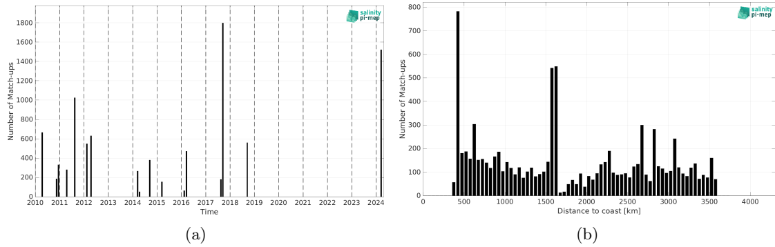
Figure 2: Number of match-ups between TSG (SAMOS) and SMOS SSS L3 v332 - 9 Days (CATDS-CPDC) SSS as a function of time (a) and as function of the distance to coast (b) over the OTT zone Pi-MEP region and for the full satellite product period.
