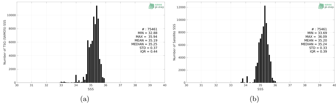
Figure 2: Histograms of SSS from TSG (SAMOS) (a) and SMOS SSS L3 v332 - 9 Days (CATDS-CPDC) (b) considering all match-up pairs per bins of 0.1 over the OTT zone Pi-MEP region and for the full satellite product period.
