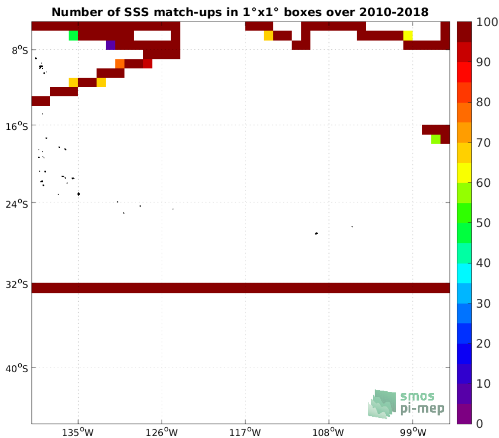
Figure 4: Number of SSS match-ups between TSG (SAMOS) SSS and the SMOS SSS L3 v332 - 9 Days (CATDS-CPDC) SSS product for the OTT zone Pi-MEP region over 1^\circ \times 1^\circ boxes and for the full satellite product period.
