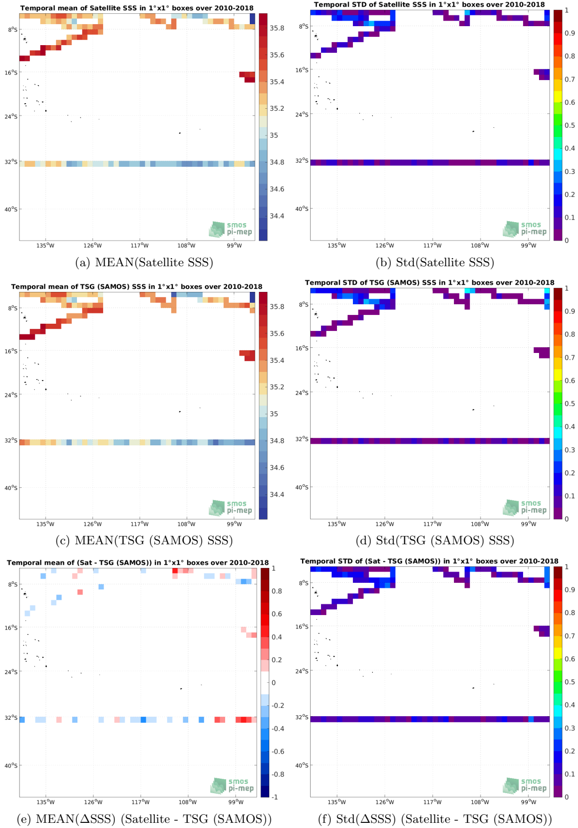
Figure 6: Temporal mean (left) and Std (right) of SSS from SMOS SSS L3 v332 - 9 Days (CATDS-CPDC) (top), TSG (SAMOS) (middle), and of \Delta SSS (Satellite - TSG (SAMOS)). Only match-up pairs are used to generate these maps.
