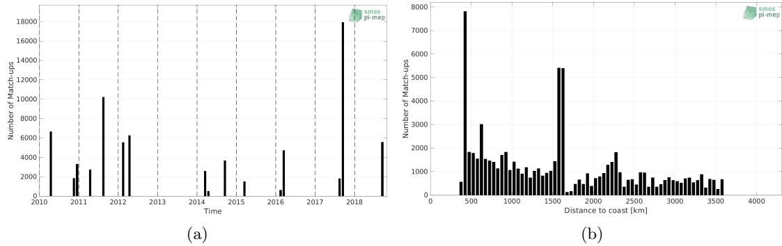
Figure 1: Number of match-ups between TSG (SAMOS) and SMOS SSS L3 v332 - 9 Days (CATDS-CPDC) SSS as a function of time (a) and as function of the distance to coast (b) over the OTT zone Pi-MEP region and for the full satellite product period.
