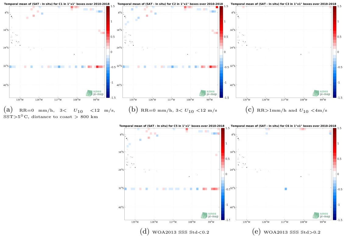
Figure 12: Temporal mean gridded over spatial boxes of size 1^\circ \times 1^\circ of \Delta SSS (SMOS SSS L3 v332 - 9 Days (CATDS-CPDC) - TSG (SAMOS)) for 5 different subdatasets corresponding to:RR=0 mm/h, 3 < U_{10} < 12 m/s, SST >5^\circ C, distance to coast > 800 km (a), RR=0 mm/h, 3 < U_{10} < 12 m/s (b), RR >1 mm/h and U_{10} < 4 m/s (c), WOA2013 SSS Std <0.2 (d), WOA2013 SSS Std >0.2 (e).
