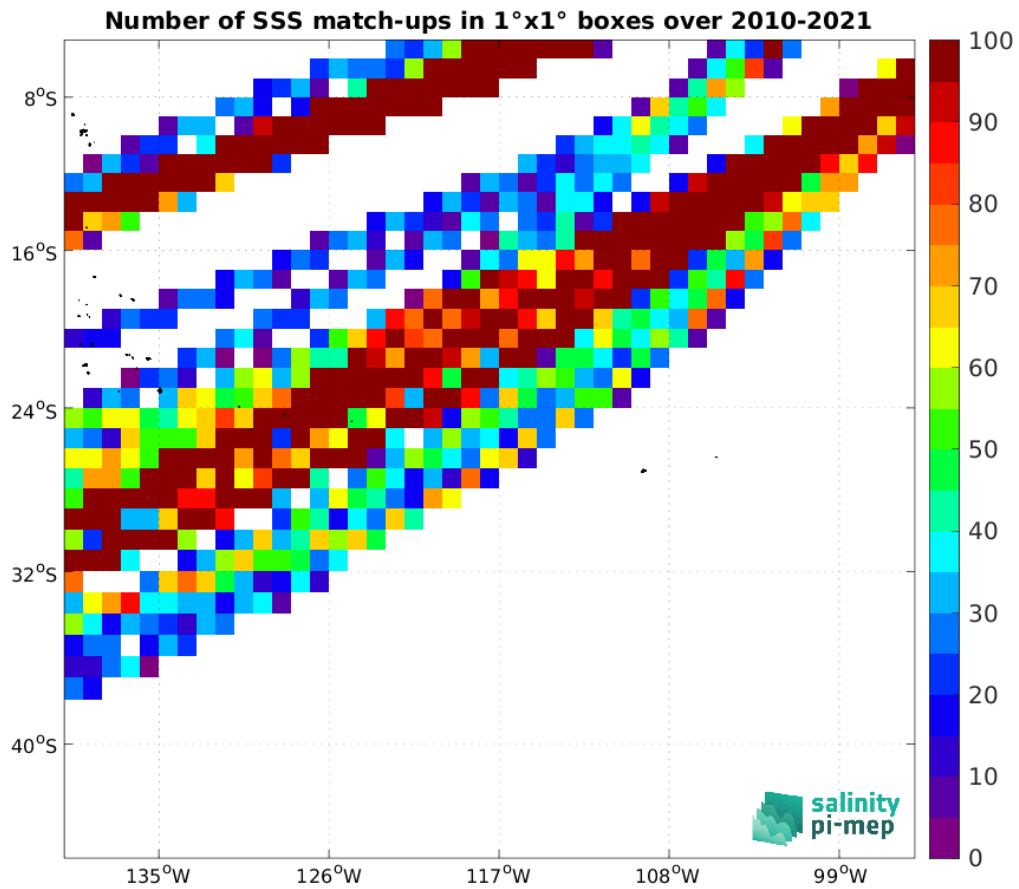
Figure 4: Number of SSS match-ups between TSG (LEGOS-DM) SSS and the SMOS SSS L3 v332 - 9 Days (CATDS-CPDC) SSS product for the OTT zone Pi-MEP region over 1^\circ \times 1^\circ boxes and for the full satellite product period.
