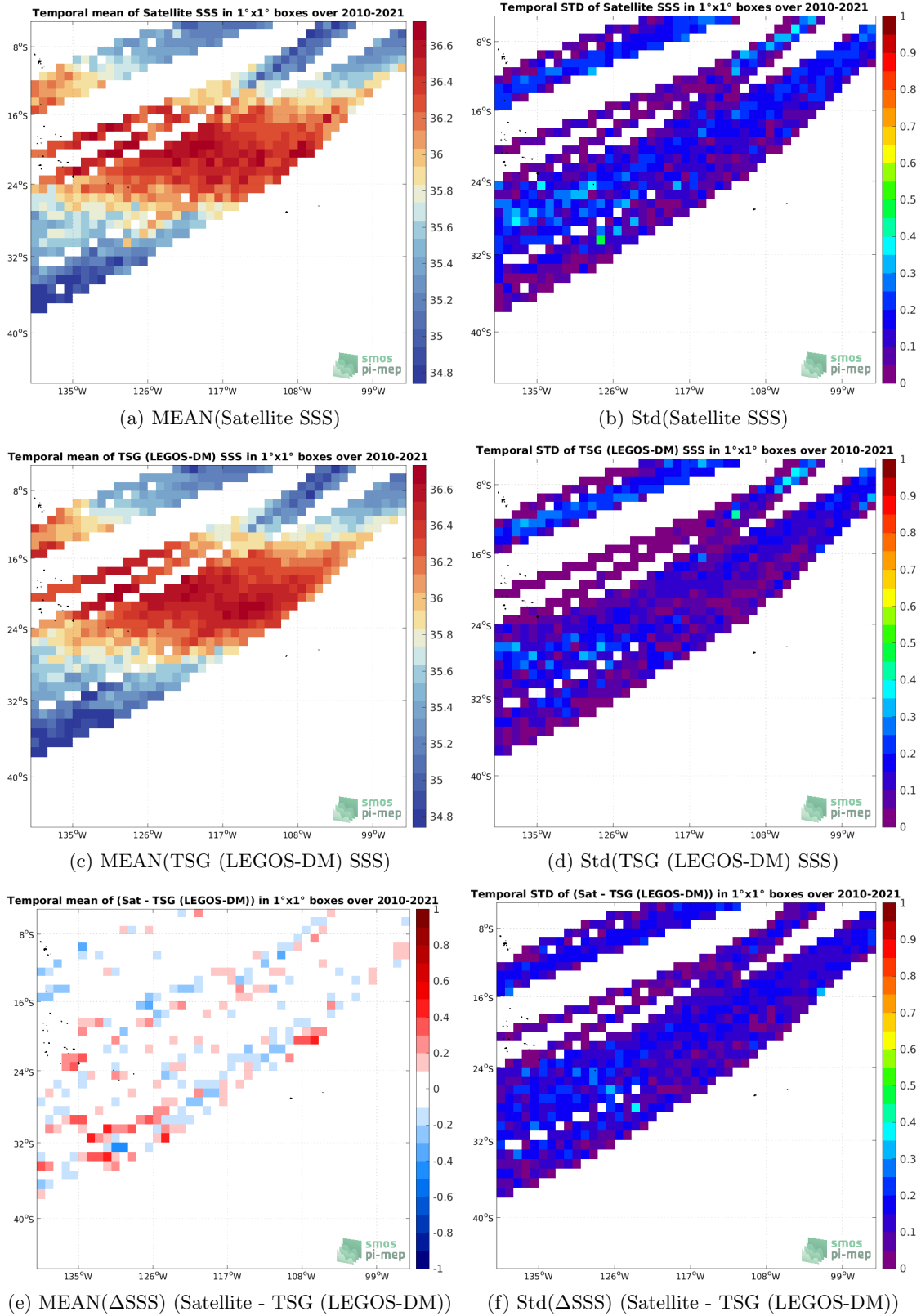
Figure 6: Temporal mean (left) and Std (right) of SSS from SMOS SSS L3 v332 - 9 Days (CATDS-CPDC) (top), TSG (LEGOS-DM) (middle), and of \Delta SSS (Satellite - TSG (LEGOS-DM)). Only match-up pairs are used to generate these maps.
