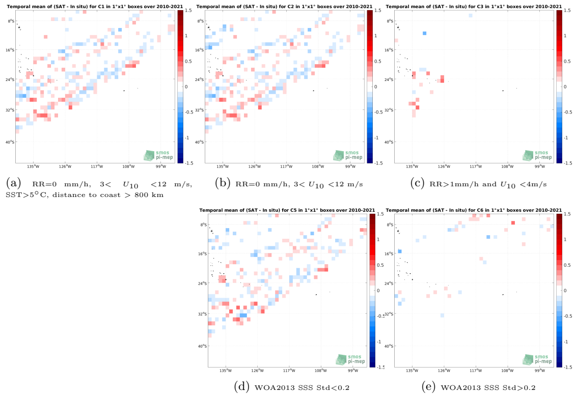
Figure 12: Temporal mean gridded over spatial boxes of size 1^\circ \times 1^\circ of \Delta SSS (SMOS SSS L3 v332 - 9 Days (CATDS-CPDC) - TSG (LEGOS-DM)) for 5 different subdatasets corresponding to:RR=0 mm/h, 3 < U_{10} < 12 m/s, SST > 5^\circ\text{C} , distance to coast > 800 km (a), RR=0 mm/h, 3 < U_{10} < 12 m/s (b), RR > 1 mm/h and U_{10} < 4 m/s (c), WOA2013 SSS Std < 0.2 (d), WOA2013 SSS Std > 0.2 (e).
