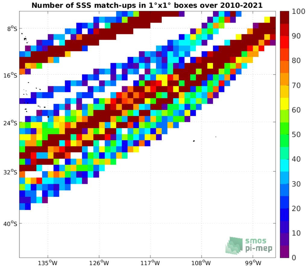
Figure 4: Number of SSS match-ups between TSG (LEGOS-DM) SSS and the SMOS SSS L3 v332 - 9 Days (CATDS-CPDC) SSS product for the OTT zone Pi-MEP region over 1°x1° boxes and for the full satellite product period.
