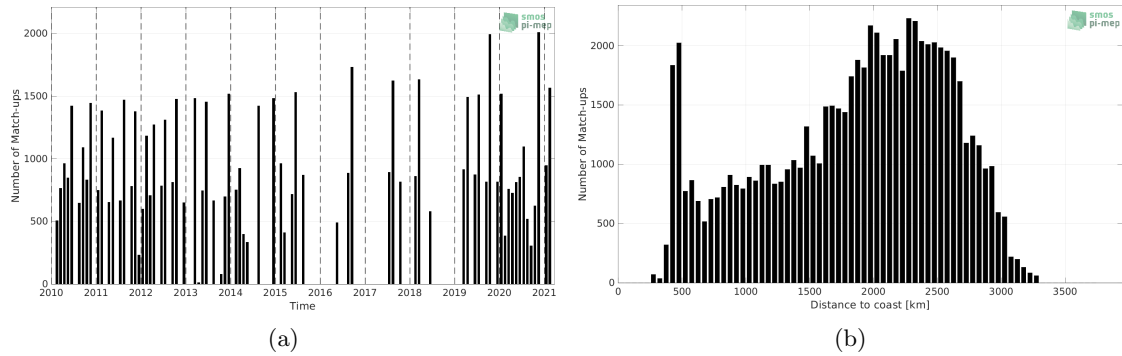
Figure 1: Number of match-ups between TSG (LEGOS-DM) and SMOS SSS L3 v332 - 9 Days (CATDS-CPDC) SSS as a function of time (a) and as function of the distance to coast (b) over the OTT zone Pi-MEP region and for the full satellite product period.
