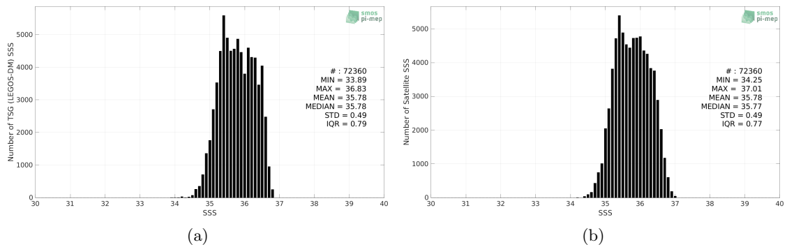
Figure 2: Histograms of SSS from TSG (LEGOS-DM) (a) and SMOS SSS L3 v332 - 9 Days (CATDS-CPDC) (b) considering all match-up pairs per bins of 0.1 over the OTT zone Pi-MEP region and for the full satellite product period.
