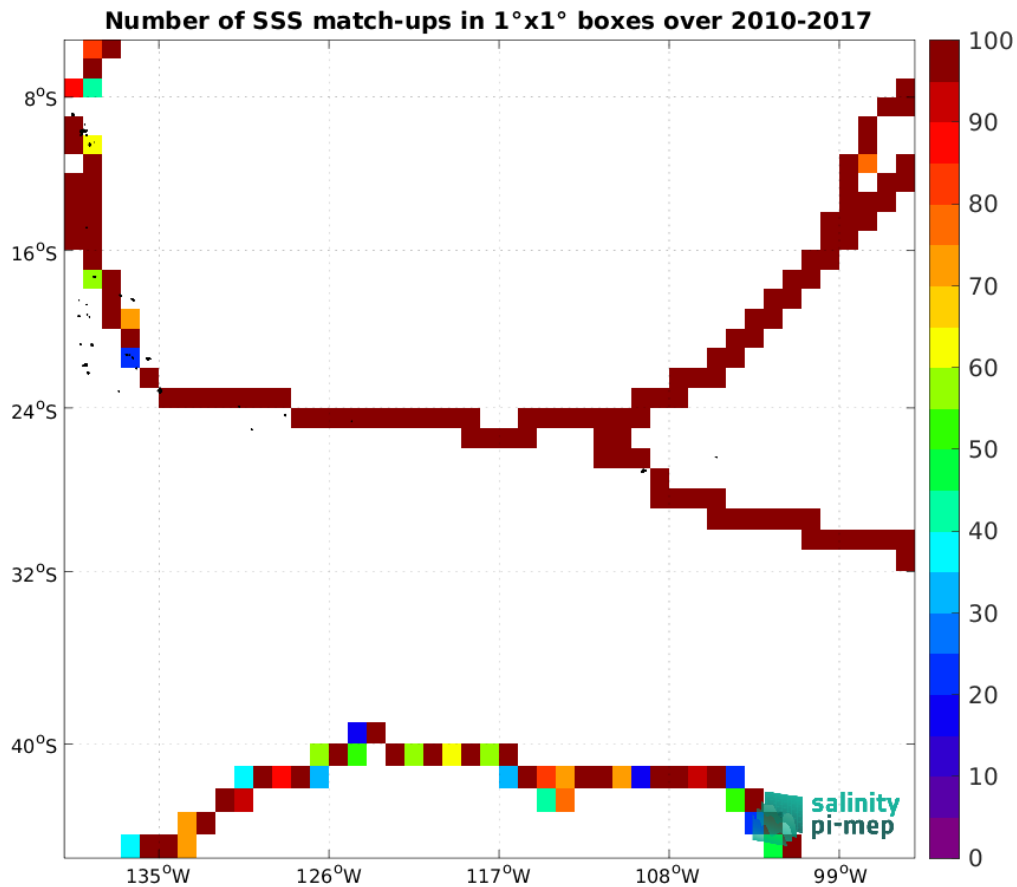
Figure 5: Number of SSS match-ups between TSG (GOSUD-Sailing-ship) SSS and the SMOS SSS L3 v332 - 9 Days (CATDS-CPDC) SSS product for the OTT zone Pi-MEP region over 1^\circ \times 1^\circ boxes and for the full satellite product period.
