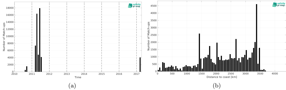
Figure 2: Number of match-ups between TSG (GOSUD-Sailing-ship) and SMOS SSS L3 v332 - 9 Days (CATDS-CPDC) SSS as a function of time (a) and as function of the distance to coast (b) over the OTT zone Pi-MEP region and for the full satellite product period.
