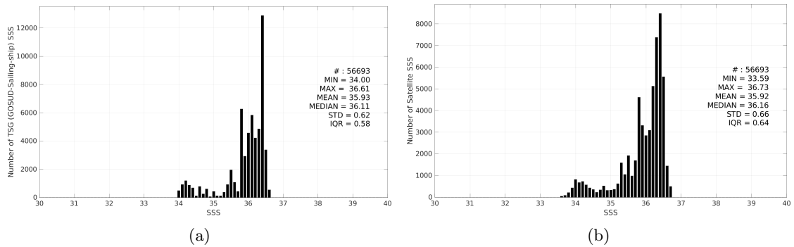
Figure 3: Histograms of SSS from TSG (GOSUD-Sailing-ship) (a) and SMOS SSS L3 v332 - 9 Days (CATDS-CPDC) (b) considering all match-up pairs per bins of 0.1 over the OTT zone Pi-MEP region and for the full satellite product period.
