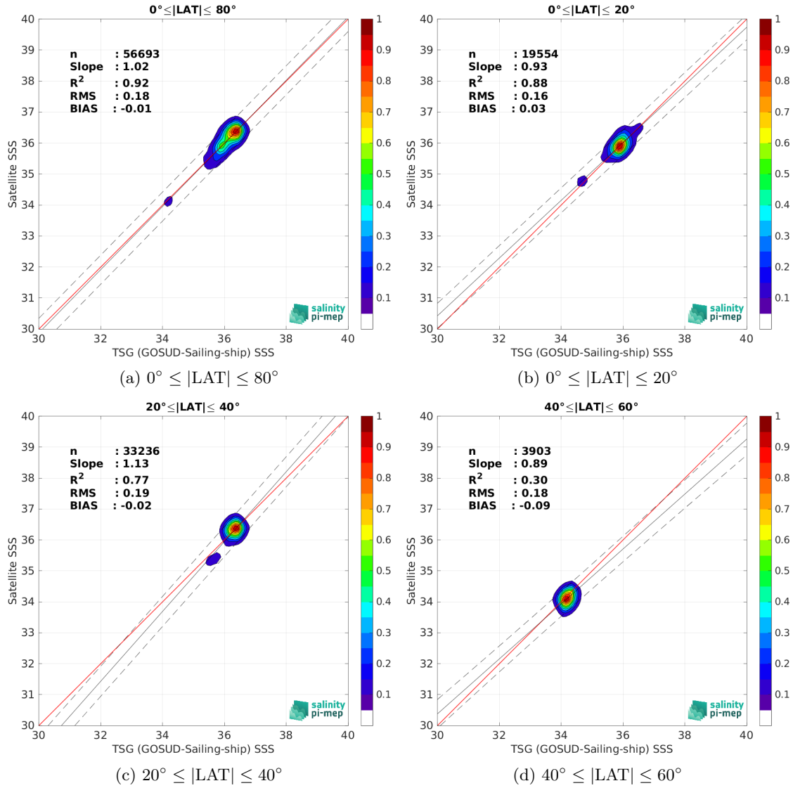
Figure 10: Contour maps of the concentration of SMOS SSS L3 v332 - 9 Days (CATDS-CPDC) SSS (y-axis) versus TSG (GOSUD-Sailing-ship) SSS (x-axis) at match-up pairs for different latitude bands. For each plot, the red line shows x=y . The black thin and dashed lines indicate a linear fit through the data cloud and the \pm 95\% confidence levels, respectively. The number match-up pairs n , the slope and R^2 coefficient of the linear fit, the root mean square (RMS) and the mean bias between satellite and in situ data are indicated for each latitude band in each plots.
