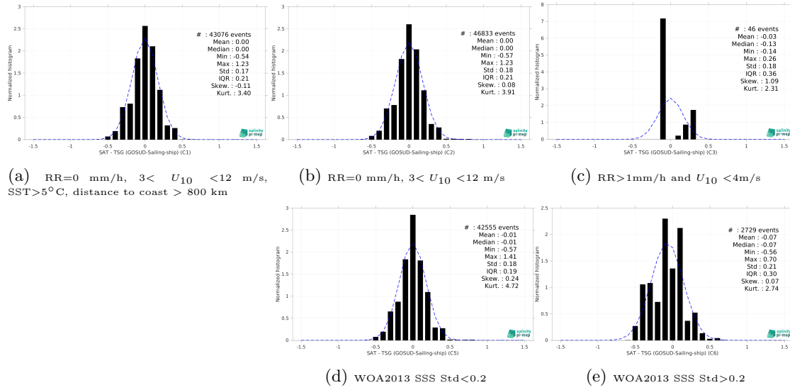
Figure 15: Normalized histogram of \Delta\text{SSS} (SMOS SSS L3 v332 - 9 Days (CATDS-CPDC) - TSG (GOSUD-Sailing-ship)) for 5 different subdatasets corresponding to: RR=0 mm/h, 3 < U_{10} < 12 m/s, SST>5°C, distance to coast > 800 km (a), RR=0 mm/h, 3 < U_{10} < 12 m/s (b), RR>1mm/h and U_{10} < 4 m/s (c), WOA2013 SSS Std<0.2 (d), WOA2013 SSS Std>0.2 (e).
