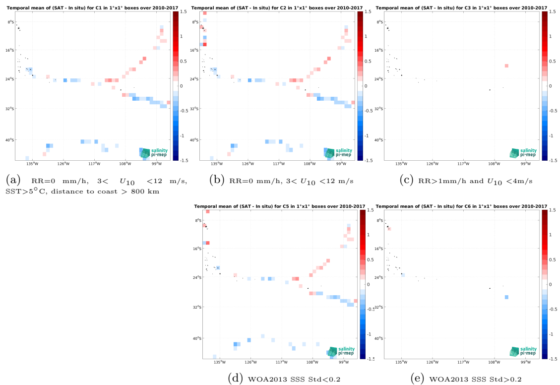
Figure 14: Temporal mean gridded over spatial boxes of size 1^\circ \times 1^\circ of \Delta SSS (SMOS SSS L3 v332 - 9 Days (CATDS-CPDC) - TSG (GOSUD-Sailing-ship)) for 5 different subdatasets corresponding to:RR=0 mm/h, 3 < U_{10} < 12 m/s, SST >5^\circ C, distance to coast > 800 km (a), RR=0 mm/h, 3 < U_{10} < 12 m/s (b), RR >1 mm/h and U_{10} < 4 m/s (c), WOA2013 SSS Std <0.2 (d), WOA2013 SSS Std >0.2 (e).
