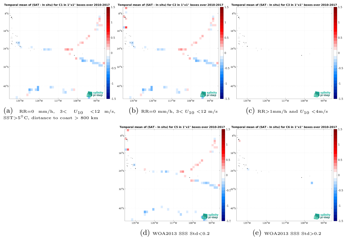
Figure 12: Temporal mean gridded over spatial boxes of size 1^\circ \times 1^\circ of \Delta SSS (SMOS SSS L3 v332 - 9 Days (CATDS-CPDC) - TSG (GOSUD-Sailing-ship)) for 5 different subdatasets corresponding to:RR=0 mm/h, 3 < U_{10} < 12 m/s, SST>5°C, distance to coast > 800 km (a), RR=0 mm/h, 3 < U_{10} < 12 m/s (b), RR>1mm/h and U_{10} < 4 m/s (c), WOA2013 SSS Std<0.2 (d), WOA2013 SSS Std>0.2 (e).
