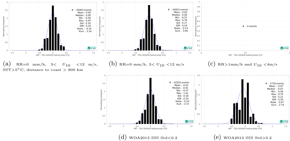
Figure 13: Normalized histogram of \Delta\text{SSS} (SMOS SSS L3 v332 - 9 Days (CATDS-CPDC) - TSG (GOSUD-Sailing-ship)) for 5 different subdatasets corresponding to: RR=0 mm/h, 3 < U_{10} < 12 m/s, SST >5^{\circ}\text{C} , distance to coast > 800 km (a), RR=0 mm/h, 3 < U_{10} < 12 m/s (b), RR >1 mm/h and U_{10} < 4 m/s (c), WOA2013 SSS Std <0.2 (d), WOA2013 SSS Std >0.2 (e).
