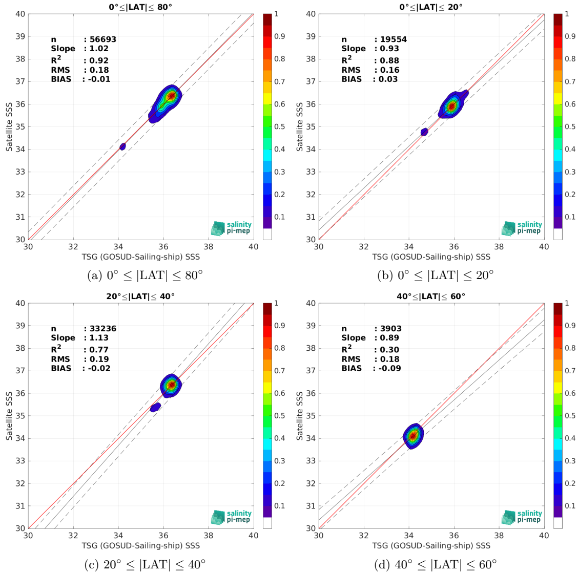
Figure 9: Contour maps of the concentration of SMOS SSS L3 v332 - 9 Days (CATDS-CPDC) SSS (y-axis) versus TSG (GOSUD-Sailing-ship) SSS (x-axis) at match-up pairs for different latitude bands. For each plot, the red line shows x=y . The black thin and dashed lines indicate a linear fit through the data cloud and the \pm 95\% confidence levels, respectively. The number match-up pairs n , the slope and R^2 coefficient of the linear fit, the root mean square (RMS) and the mean bias between satellite and in situ data are indicated for each latitude band in each plots.
