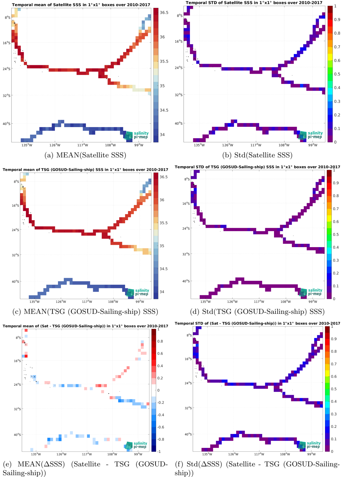
Figure 6: Temporal mean (left) and Std (right) of SSS from SMOS SSS L3 v332 - 9 Days (CATDS-CPDC) (top), TSG (GOSUD-Sailing-ship) (middle), and of \Delta SSS (Satellite - TSG (GOSUD-Sailing-ship)). Only match-up pairs are used to generate these maps.
