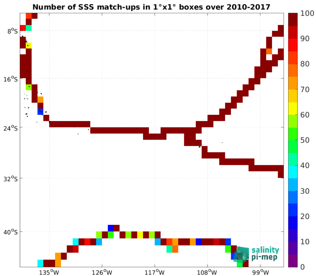
Figure 4: Number of SSS match-ups between TSG (GOSUD-Sailing-ship) SSS and the SMOS SSS L3 v332 - 9 Days (CATDS-CPDC) SSS product for the OTT zone Pi-MEP region over 1^\circ \times 1^\circ boxes and for the full satellite product period.
