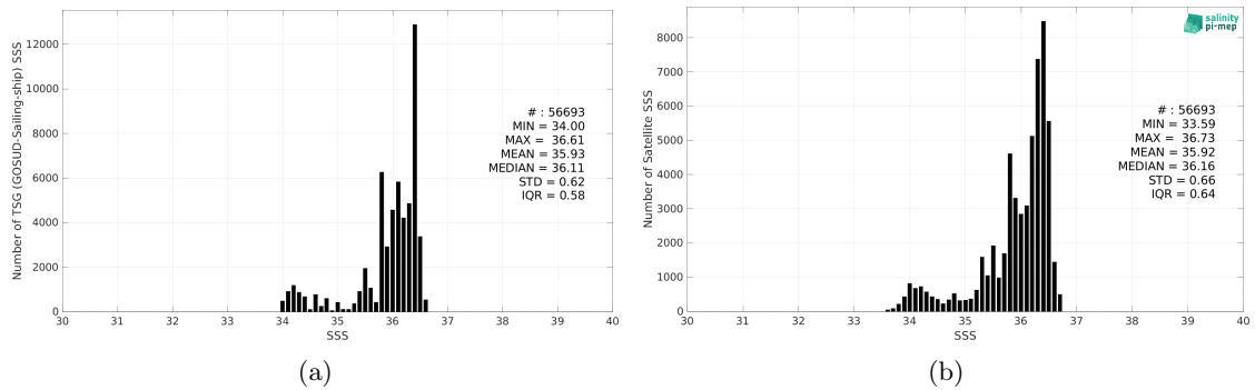
Figure 2: Histograms of SSS from TSG (GOSUD-Sailing-ship) (a) and SMOS SSS L3 v332 - 9 Days (CATDS-CPDC) (b) considering all match-up pairs per bins of 0.1 over the OTT zone Pi-MEP region and for the full satellite product period.
