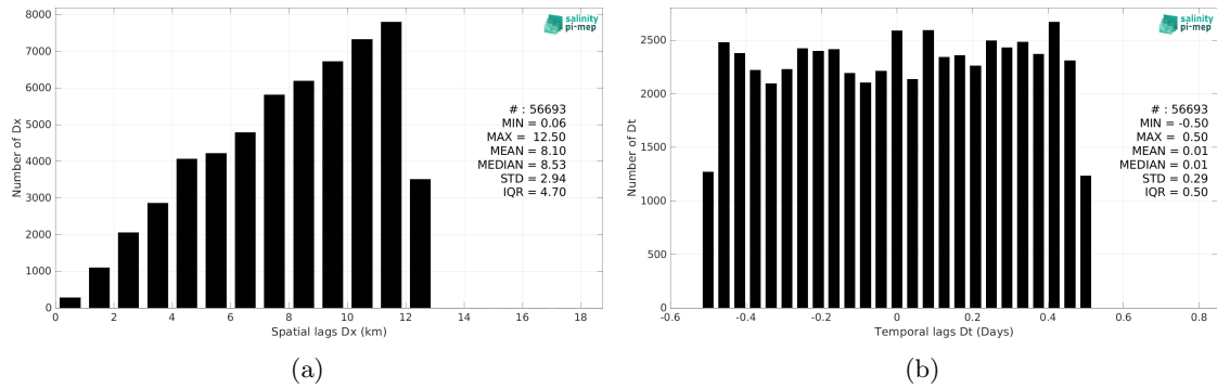
Figure 5: Histograms of the spatial (a) and temporal (b) lags between the location/time of the TSG (GOSUD-Sailing-ship) measurement and the date of the corresponding SMOS SSS L3 v332 - 9 Days (CATDS-CPDC) SSS pixel.
