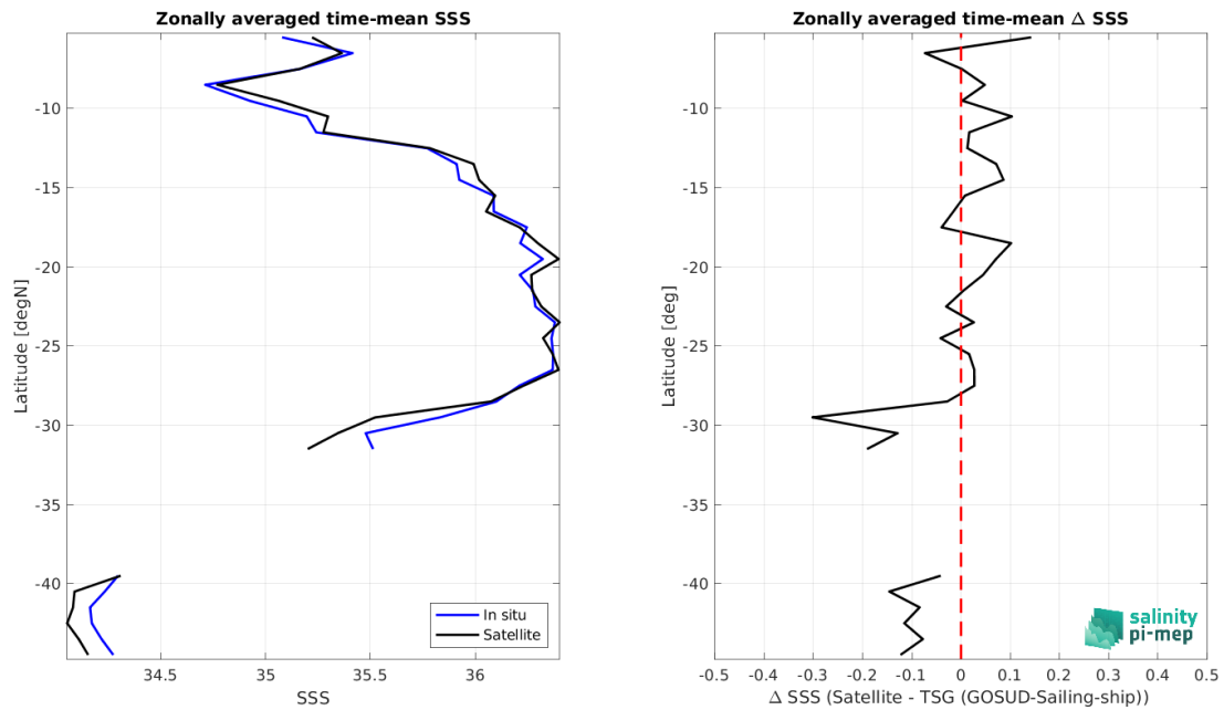
Figure 8: Left panel: Zonal mean SSS from SMOS SSS L3 v332 - 9 Days (CATDS-CPDC) satellite product (black) and from TSG (GOSUD-Sailing-ship) (blue). Right panel: Zonal mean of \Delta SSS (Satellite - TSG (GOSUD-Sailing-ship)) for all the collected Pi-MEP match-up pairs estimated over the full satellite product period.
