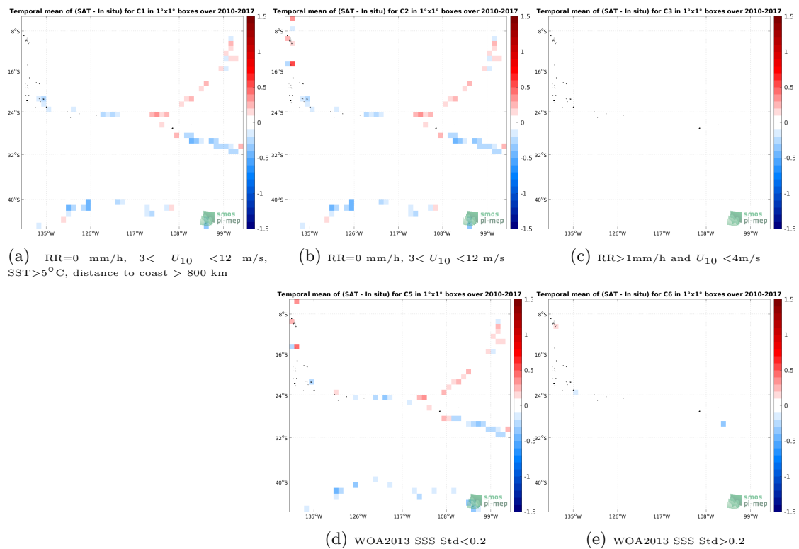
Figure 12: Temporal mean gridded over spatial boxes of size 1^\circ \times 1^\circ of \Delta SSS (SMOS SSS L3 v332 - 9 Days (CATDS-CPDC) - TSG (GOSUD-Sailing-ship)) for 5 different subdatasets corresponding to:RR=0 mm/h, 3 < U_{10} < 12 m/s, SST>5°C, distance to coast > 800 km (a), RR=0 mm/h, 3 < U_{10} < 12 m/s (b), RR>1mm/h and U_{10} < 4 m/s (c), WOA2013 SSS Std<0.2 (d), WOA2013 SSS Std>0.2 (e).
