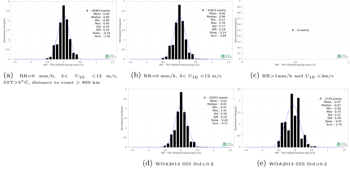
Figure 13: Normalized histogram of \Delta SSS (SMOS SSS L3 v332 - 9 Days (CATDS-CPDC) - TSG (GOSUD-Sailing-ship)) for 5 different subdatasets corresponding to: RR=0 mm/h, 3 < U_{10} < 12 m/s, SST > 5°C, distance to coast > 800 km (a), RR=0 mm/h, 3 < U_{10} < 12 m/s (b), RR > 1mm/h and U_{10} < 4 m/s (c), WOA2013 SSS Std < 0.2 (d), WOA2013 SSS Std > 0.2 (e).
