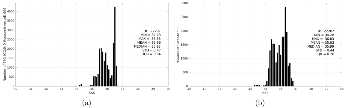
Figure 3: Histograms of SSS from TSG (GOSUD-Research-vessel) (a) and SMOS SSS L3 v332 - 9 Days (CATDS-CPDC) (b) considering all match-up pairs per bins of 0.1 over the OTT zone Pi-MEP region and for the full satellite product period.
