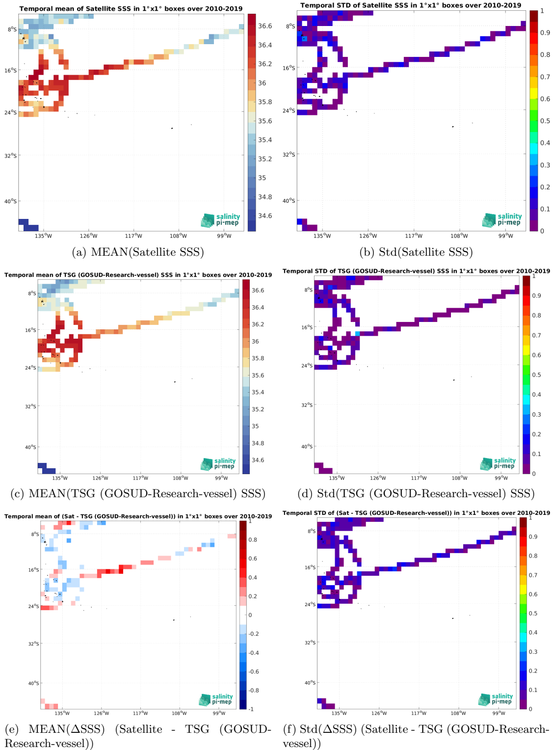
Figure 7: Temporal mean (left) and Std (right) of SSS from SMOS SSS L3 v332 - 9 Days (CATDS-CPDC) (top), TSG (GOSUD-Research-vessel) (middle), and of \Delta SSS (Satellite - TSG (GOSUD-Research-vessel)). Only match-up pairs are used to generate these maps.
