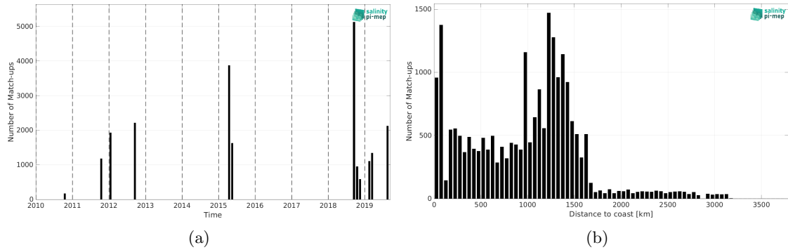
Figure 2: Number of match-ups between TSG (GOSUD-Research-vessel) and SMOS SSS L3 v332 - 9 Days (CATDS-CPDC) SSS as a function of time (a) and as function of the distance to coast (b) over the OTT zone Pi-MEP region and for the full satellite product period.
