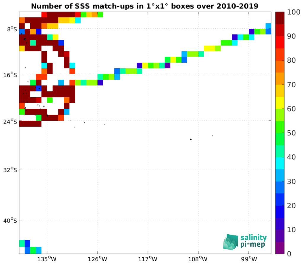
Figure 5: Number of SSS match-ups between TSG (GOSUD-Research-vessel) SSS and the SMOS SSS L3 v332 - 9 Days (CATDS-CPDC) SSS product for the OTT zone Pi-MEP region over 1^\circ \times 1^\circ boxes and for the full satellite product period.
