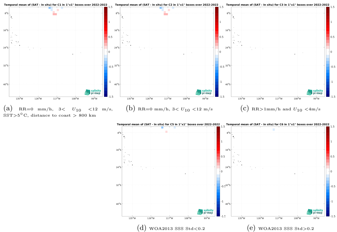
Figure 14: Temporal mean gridded over spatial boxes of size 1^\circ \times 1^\circ of \Delta SSS (SMOS SSS L3 v332 - 9 Days (CATDS-CPDC) - Sairdrone) for 5 different subdatasets corresponding to:RR=0 mm/h, 3 < U_{10} < 12 m/s, SST >5^\circ C, distance to coast > 800 km (a), RR=0 mm/h, 3 < U_{10} < 12 m/s (b), RR >1 mm/h and U_{10} < 4 m/s (c), WOA2013 SSS Std <0.2 (d), WOA2013 SSS Std >0.2 (e).
