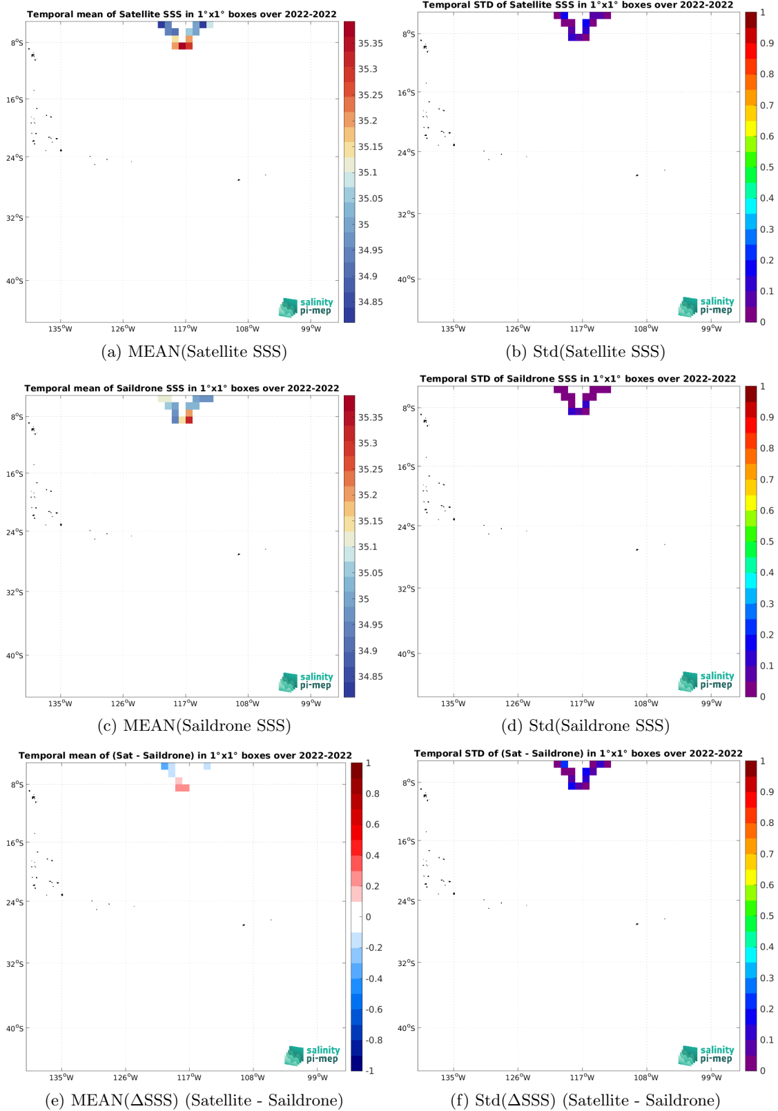
Figure 7: Temporal mean (left) and Std (right) of SSS from SMOS SSS L3 v332 - 9 Days (CATDS-CPDC) (top), Saildrone (middle), and of \Delta SSS (Satellite - Saildrone). Only match-up pairs are used to generate these maps.
