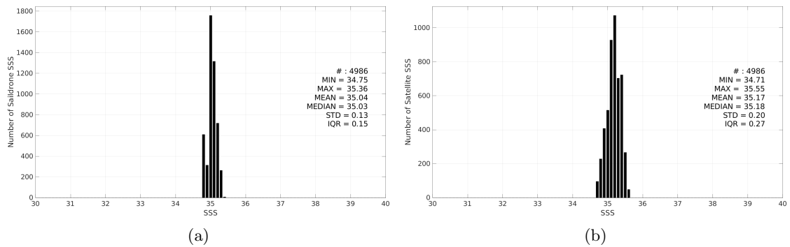
Figure 3: Histograms of SSS from Saildrone (a) and SMOS SSS L3 v332 - 9 Days (CATDS-CPDC) (b) considering all match-up pairs per bins of 0.1 over the OTT zone Pi-MEP region and for the full satellite product period.
