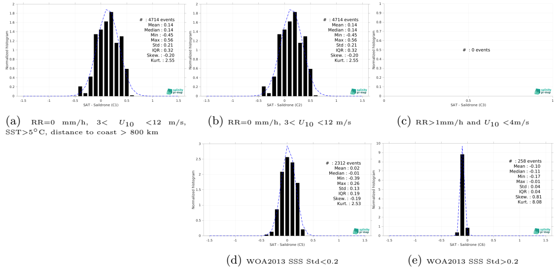
Figure 15: Normalized histogram of \Delta SSS (SMOS SSS L3 v332 - 9 Days (CATDS-CPDC) - Saildrone) for 5 different subdatasets corresponding to: RR=0 mm/h, 3 < U_{10} < 12 m/s, SST > 5°C, distance to coast > 800 km (a), RR=0 mm/h, 3 < U_{10} < 12 m/s (b), RR > 1mm/h and U_{10} < 4 m/s (c), WOA2013 SSS Std < 0.2 (d), WOA2013 SSS Std > 0.2 (e).
