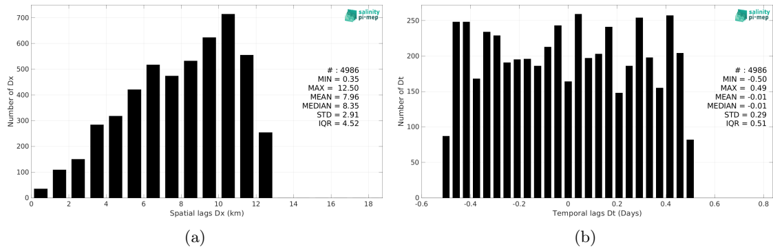
Figure 6: Histograms of the spatial (a) and temporal (b) lags between the location/time of the Saildrone measurement and the date of the corresponding SMOS SSS L3 v332 - 9 Days (CATDS-CPDC) SSS pixel.
