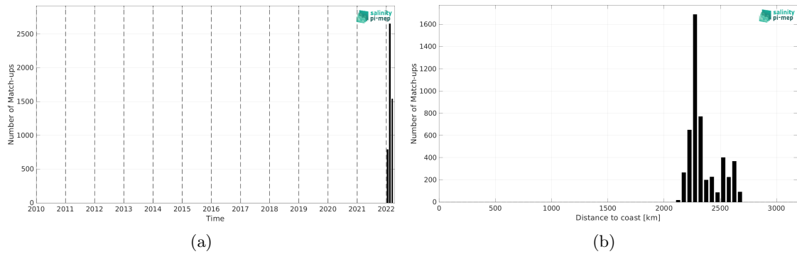
Figure 2: Number of match-ups between Saildrone and SMOS SSS L3 v332 - 9 Days (CATDS-CPDC) SSS as a function of time (a) and as function of the distance to coast (b) over the OTT zone Pi-MEP region and for the full satellite product period.
