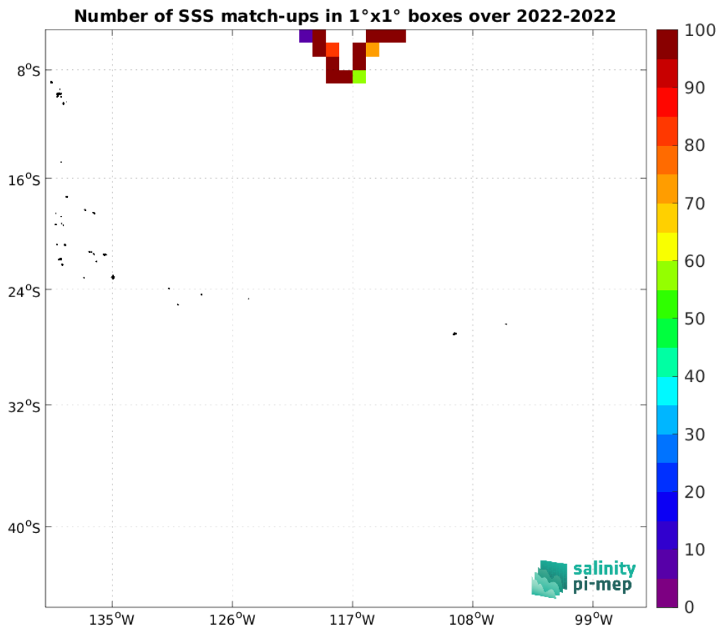
Figure 5: Number of SSS match-ups between Saildrone SSS and the SMOS SSS L3 v332 - 9 Days (CATDS-CPDC) SSS product for the OTT zone Pi-MEP region over 1°x1° boxes and for the full satellite product period.
