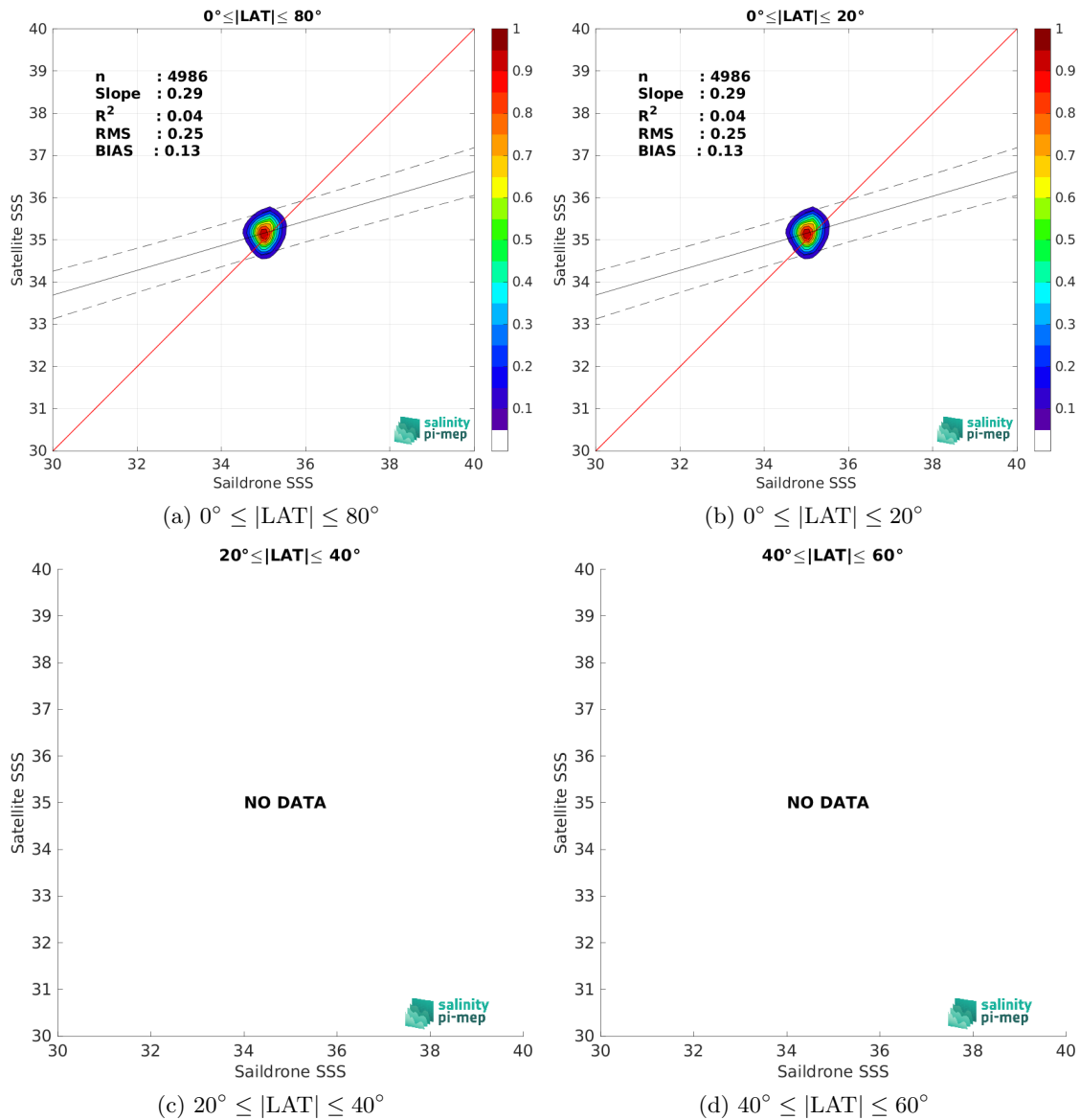
Figure 10: Contour maps of the concentration of SMOS SSS L3 v332 - 9 Days (CATDS-CPDC) SSS (y-axis) versus Saildrone SSS (x-axis) at match-up pairs for different latitude bands. For each plot, the red line shows x=y . The black thin and dashed lines indicate a linear fit through the data cloud and the \pm 95\% confidence levels, respectively. The number match-up pairs n , the slope and R^2 coefficient of the linear fit, the root mean square (RMS) and the mean bias between satellite and in situ data are indicated for each latitude band in each plots.
