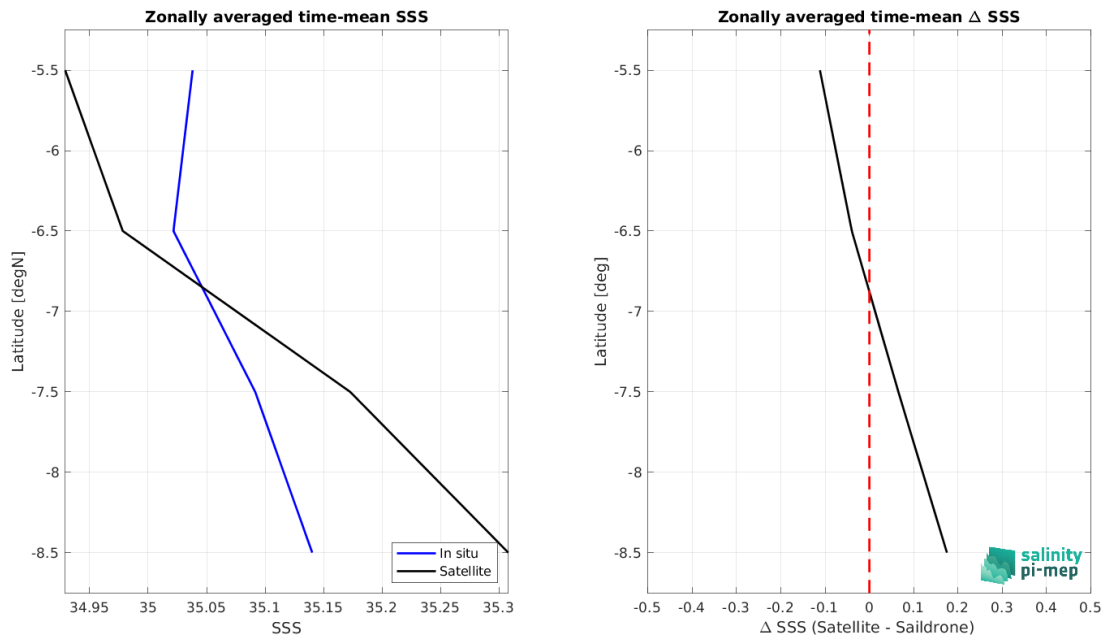
Figure 9: Left panel: Zonal mean SSS from SMOS SSS L3 v332 - 9 Days (CATDS-CPDC) satellite product (black) and from Sairdrone (blue). Right panel: Zonal mean of \Delta SSS (Satellite - Sairdrone) for all the collected Pi-MEP match-up pairs estimated over the full satellite product period.
