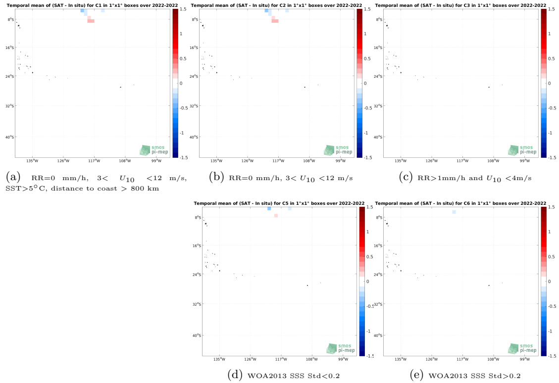
Figure 12: Temporal mean gridded over spatial boxes of size 1^\circ \times 1^\circ of \Delta SSS (SMOS SSS L3 v332 - 9 Days (CATDS-CPDC) - Sairdrone) for 5 different subdatasets corresponding to:RR=0 mm/h, 3 < U_{10} < 12 m/s, SST >5^\circ C, distance to coast > 800 km (a), RR=0 mm/h, 3 < U_{10} < 12 m/s (b), RR >1 mm/h and U_{10} < 4 m/s (c), WOA2013 SSS Std <0.2 (d), WOA2013 SSS Std >0.2 (e).
