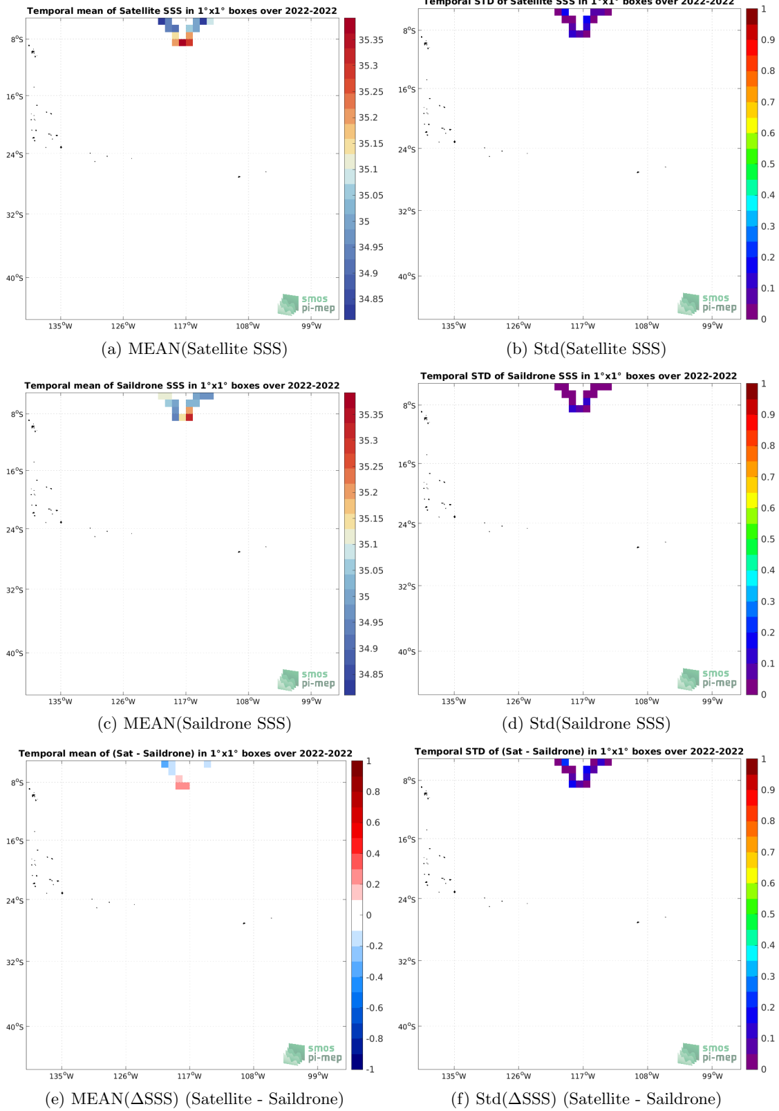
Figure 6: Temporal mean (left) and Std (right) of SSS from SMOS SSS L3 v332 - 9 Days (CATDS-CPDC) (top), Saildrone (middle), and of \Delta SSS (Satellite - Saildrone). Only match-up pairs are used to generate these maps.
