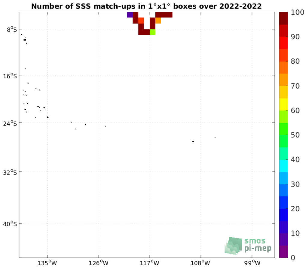
Figure 4: Number of SSS match-ups between Saildrone SSS and the SMOS SSS L3 v332 - 9 Days (CATDS-CPDC) SSS product for the OTT zone Pi-MEP region over 1°x1° boxes and for the full satellite product period.
