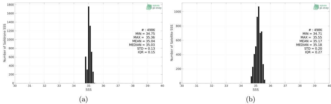
Figure 2: Histograms of SSS from Saildrone (a) and SMOS SSS L3 v332 - 9 Days (CATDS-CPDC) (b) considering all match-up pairs per bins of 0.1 over the OTT zone Pi-MEP region and for the full satellite product period.
