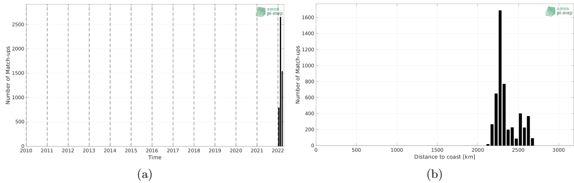
Figure 1: Number of match-ups between Saildrone and SMOS SSS L3 v332 - 9 Days (CATDS-CPDC) SSS as a function of time (a) and as function of the distance to coast (b) over the OTT zone Pi-MEP region and for the full satellite product period.
