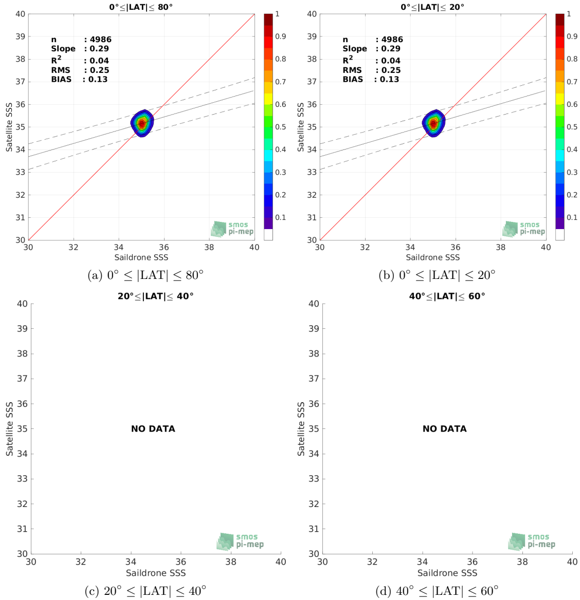
Figure 9: Contour maps of the concentration of SMOS SSS L3 v332 - 9 Days (CATDS-CPDC) SSS (y-axis) versus Saildrone SSS (x-axis) at match-up pairs for different latitude bands. For each plot, the red line shows x=y . The black thin and dashed lines indicate a linear fit through the data cloud and the \pm 95\% confidence levels, respectively. The number match-up pairs n , the slope and R^2 coefficient of the linear fit, the root mean square (RMS) and the mean bias between satellite and in situ data are indicated for each latitude band in each plots.
