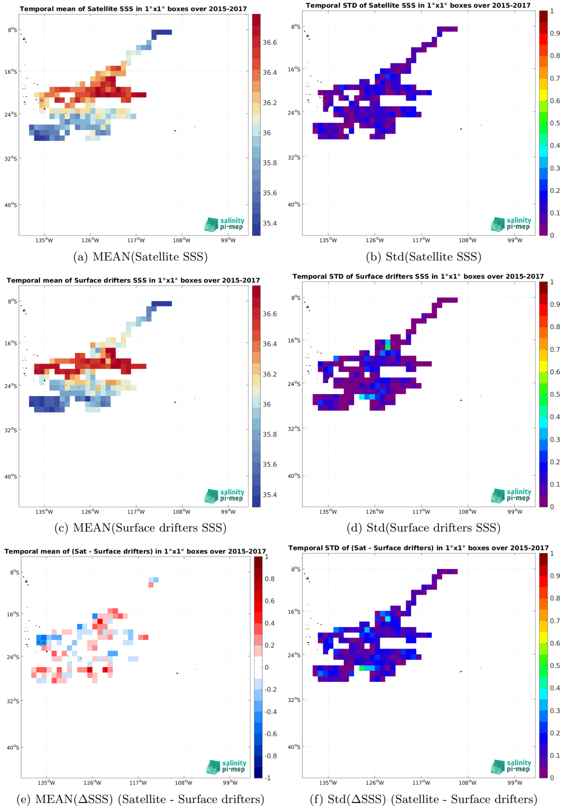
Figure 6: Temporal mean (left) and Std (right) of SSS from SMOS SSS L3 v332 - 9 Days (CATDS-CPDC) (top), Surface drifters (middle), and of \Delta SSS (Satellite - Surface drifters). Only match-up pairs are used to generate these maps.
