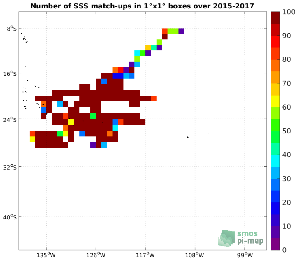
Figure 3: Number of SSS match-ups between Surface drifters SSS and the SMOS SSS L3 v332 - 9 Days (CATDS-CPDC) SSS product for the OTT zone Pi-MEP region over 1°x1° boxes and for the full satellite product period.
