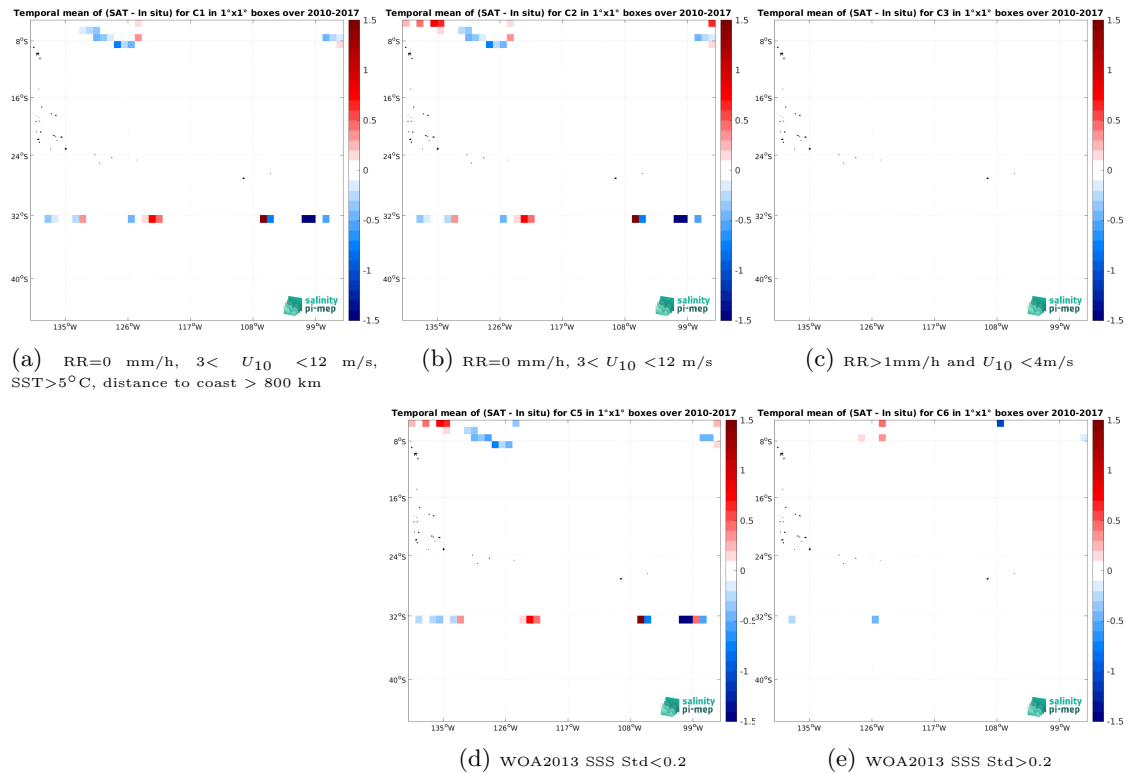
Figure 12: Temporal mean gridded over spatial boxes of size 1^\circ \times 1^\circ of \Delta\text{SSS} (SMOS SSS L2Q v331 - 0.25 Deg (CATDS-CPDC) - TSG (SAMOS)) for 5 different subdatasets corresponding to: \text{RR}=0 mm/h, 3 < U_{10} < 12 m/s, \text{SST} > 5^\circ\text{C} , distance to coast > 800 km (a), \text{RR}=0 mm/h, 3 < U_{10} < 12 m/s (b), \text{RR} > 1\text{mm/h} and U_{10} < 4\text{m/s} (c), WOA2013 SSS Std < 0.2 (d), WOA2013 SSS Std > 0.2 (e).
