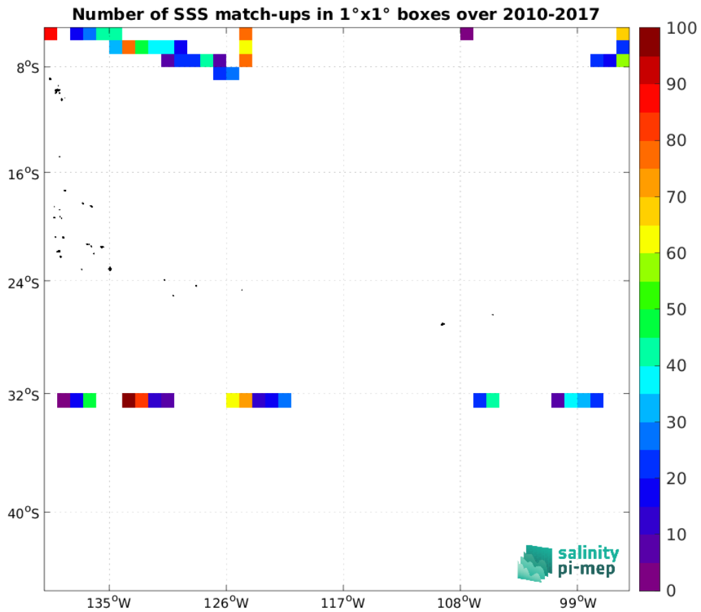
Figure 4: Number of SSS match-ups between TSG (SAMOS) SSS and the SMOS SSS L2Q v331 - 0.25 Deg (CATDS-CPDC) SSS product for the OTT zone Pi-MEP region over 1^\circ \times 1^\circ boxes and for the full satellite product period.
