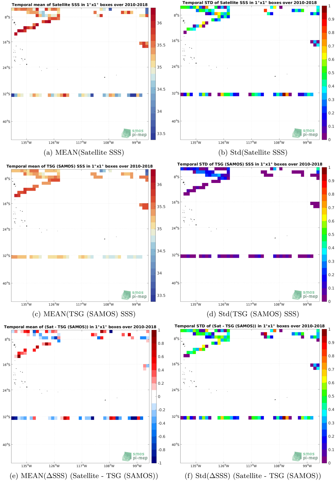
Figure 6: Temporal mean (left) and Std (right), of SSS from SMOS SSS L2Q v331 - 0.25 Deg (CATDS-CPDC) (top), TSG (SAMOS) (middle), and of \Delta SSS (Satellite - TSG (SAMOS)). Only match-up pairs are used to generate these maps.
