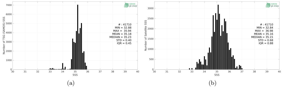
Figure 2: Histograms of SSS from TSG (SAMOS) (a) and SMOS SSS L2Q v331 - 0.25 Deg (CATDS-CPDC) (b) considering all match-up pairs per bins of 0.1 over the OTT zone Pi-MEP region and for the full satellite product period.
