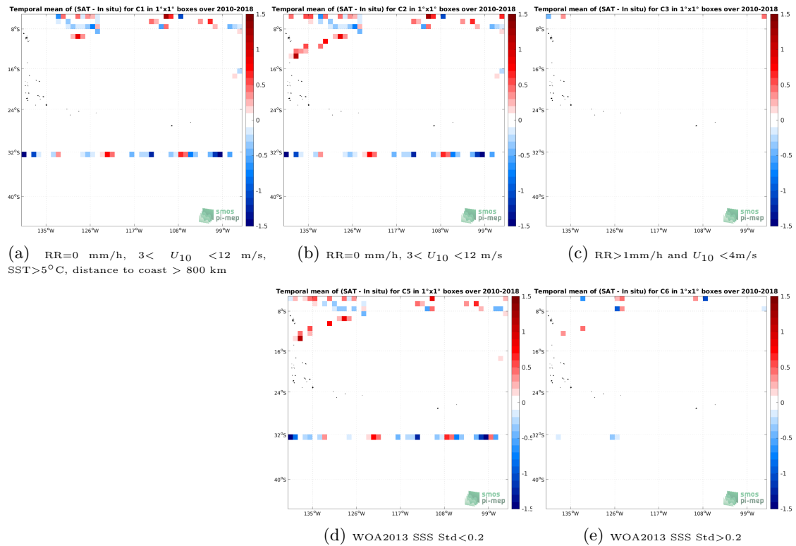
Figure 12: Temporal mean gridded over spatial boxes of size 1^\circ \times 1^\circ of \Delta SSS (SMOS SSS L2Q v331 - 0.25 Deg (CATDS-CPDC) - TSG (SAMOS)) for 5 different subdatasets corresponding to:RR=0 mm/h, 3 < U_{10} < 12 m/s, SST >5^\circ C, distance to coast > 800 km (a), RR=0 mm/h, 3 < U_{10} < 12 m/s (b), RR >1 mm/h and U_{10} < 4 m/s (c), WOA2013 SSS Std <0.2 (d), WOA2013 SSS Std >0.2 (e).
