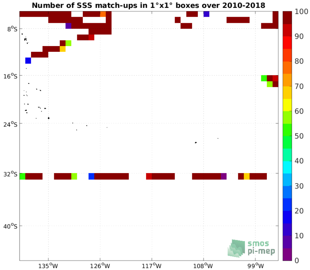
Figure 4: Number of SSS match-ups between TSG (SAMOS) SSS and the SMOS SSS L2Q v331 - 0.25 Deg (CATDS-CPDC) SSS product for the OTT zone Pi-MEP region over 1°x1° boxes and for the full satellite product period.
