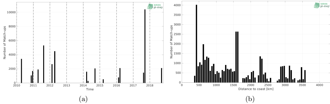
Figure 1: Number of match-ups between TSG (SAMOS) and SMOS SSS L2Q v331 - 0.25 Deg (CATDS-CPDC) SSS as a function of time (a) and as function of the distance to coast (b) over the OTT zone Pi-MEP region and for the full satellite product period.
