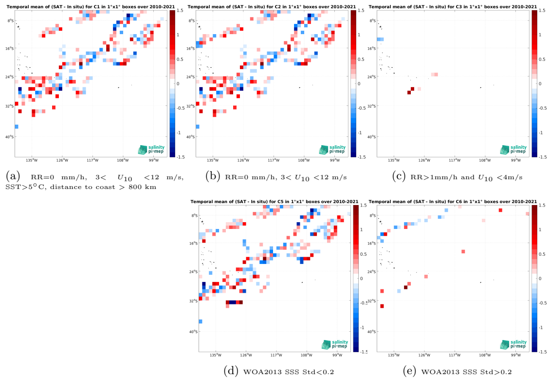
Figure 12: Temporal mean gridded over spatial boxes of size 1^{\circ}\times 1^{\circ} of \Delta\text{SSS} (SMOS SSS L2Q v331 - 0.25 Deg (CATDS-CPDC) - TSG (LEGOS-DM)) for 5 different subdatasets corresponding to:RR=0 mm/h, 3 < U_{10} < 12 m/s, SST >5^{\circ}\text{C} , distance to coast > 800 km (a), RR=0 mm/h, 3 < U_{10} < 12 m/s (b), RR >1\text{mm/h} and U_{10} < 4\text{m/s} (c), WOA2013 SSS Std <0.2 (d), WOA2013 SSS Std >0.2 (e).
