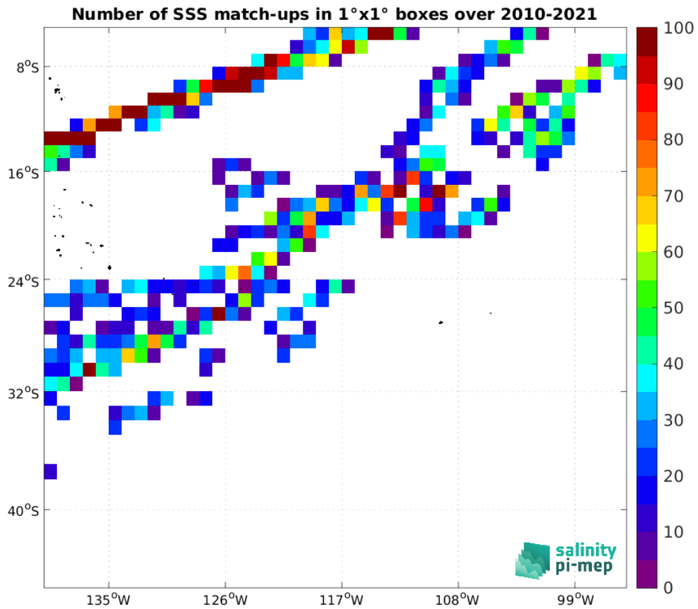
Figure 4: Number of SSS match-ups between TSG (LEGOS-DM) SSS and the SMOS SSS L2Q v331 - 0.25 Deg (CATDS-CPDC) SSS product for the OTT zone Pi-MEP region over 1^\circ \times 1^\circ boxes and for the full satellite product period.
