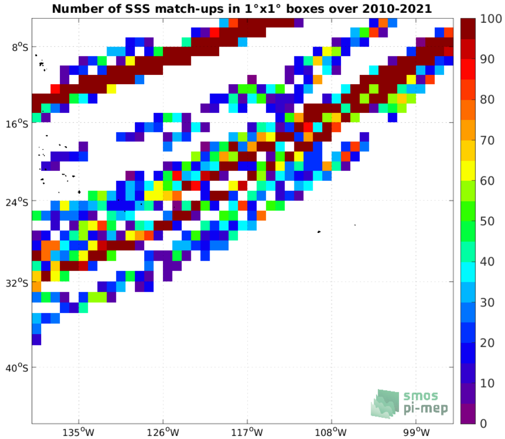
Figure 4: Number of SSS match-ups between TSG (LEGOS-DM) SSS and the SMOS SSS L2Q v331 - 0.25 Deg (CATDS-CPDC) SSS product for the OTT zone Pi-MEP region over 1°x1° boxes and for the full satellite product period.
