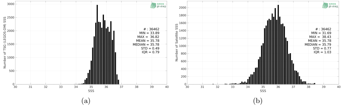
Figure 2: Histograms of SSS from TSG (LEGOS-DM) (a) and SMOS SSS L2Q v331 - 0.25 Deg (CATDS-CPDC) (b) considering all match-up pairs per bins of 0.1 over the OTT zone Pi-MEP region and for the full satellite product period.
