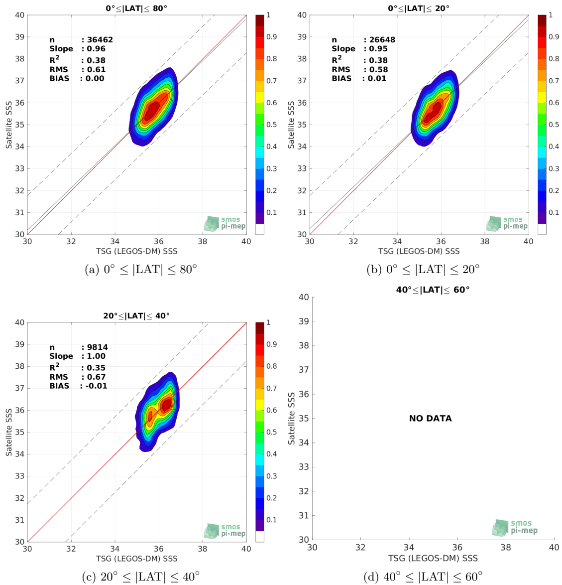
Figure 9: Contour maps of the concentration of SMOS SSS L2Q v331 - 0.25 Deg (CATDS-CPDC) SSS (y-axis) versus TSG (LEGOS-DM) SSS (x-axis) at match-up pairs for different latitude bands. For each plot, the red line shows x=y . The black thin and dashed lines indicate a linear fit through the data cloud and the \pm 95\% confidence levels, respectively. The number match-up pairs n , the slope and R^2 coefficient of the linear fit, the root mean square (RMS) and the mean bias between satellite and in situ data are indicated for each latitude band in each plots.
