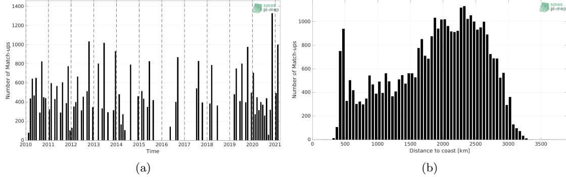
Figure 1: Number of match-ups between TSG (LEGOS-DM) and SMOS SSS L2Q v331 - 0.25 Deg (CATDS-CPDC) SSS as a function of time (a) and as function of the distance to coast (b) over the OTT zone Pi-MEP region and for the full satellite product period.
