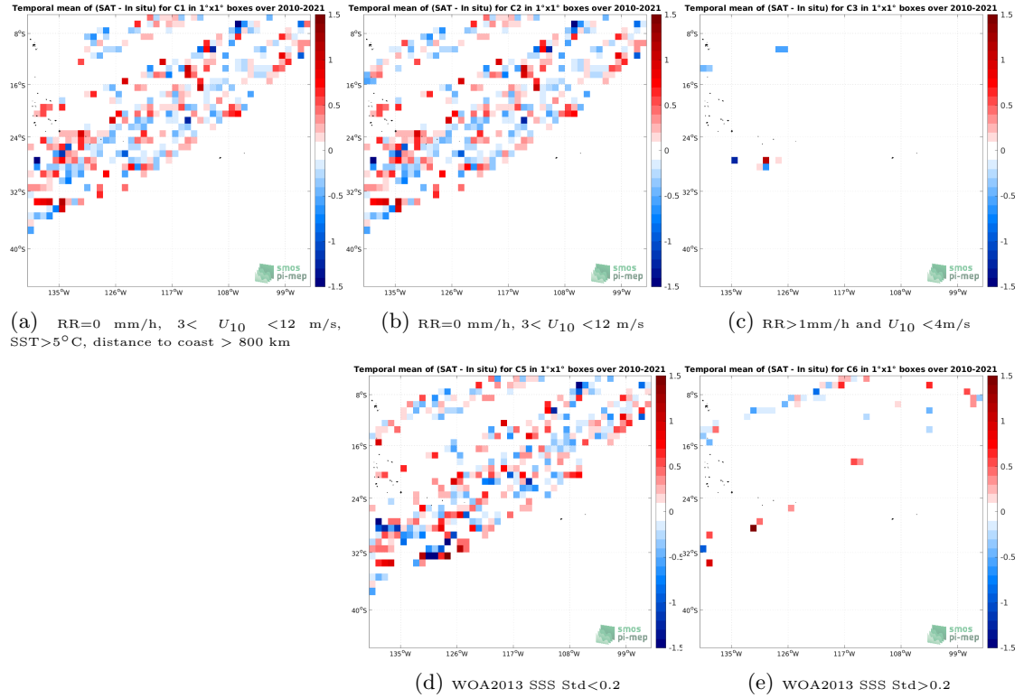
Figure 12: Temporal mean gridded over spatial boxes of size 1^{\circ}\times 1^{\circ} of \Delta\text{SSS} (SMOS SSS L2Q v331 - 0.25 Deg (CATDS-CPDC) - TSG (LEGOS-DM)) for 5 different subdatasets corresponding to:RR=0 mm/h, 3 < U_{10} < 12 m/s, SST >5^{\circ}\text{C} , distance to coast > 800 km (a), RR=0 mm/h, 3 < U_{10} < 12 m/s (b), RR >1\text{mm/h} and U_{10} < 4\text{m/s} (c), WOA2013 SSS Std <0.2 (d), WOA2013 SSS Std >0.2 (e).
