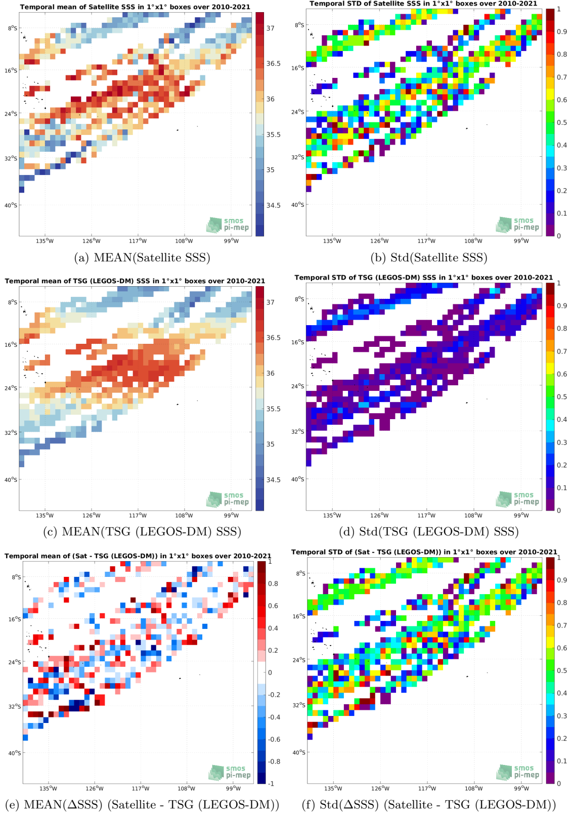
Figure 6: Temporal mean (left) and Std (right) of SSS from SMOS SSS L2Q v331 - 0.25 Deg (CATDS-CPDC) (top), TSG (LEGOS-DM) (middle), and of \Delta SSS (Satellite - TSG (LEGOS-DM)). Only match-up pairs are used to generate these maps.
