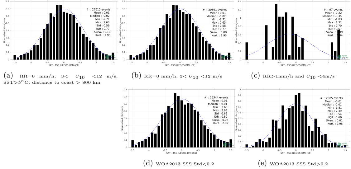
Figure 13: Normalized histogram of \Delta\text{SSS} (SMOS SSS L2Q v331 - 0.25 Deg (CATDS-CPDC) - TSG (LEGOS-DM)) for 5 different subdatasets corresponding to: RR=0 mm/h, 3 < U_{10} < 12 m/s, SST>5°C, distance to coast > 800 km (a), RR=0 mm/h, 3 < U_{10} < 12 m/s (b), RR>1mm/h and U_{10} < 4 m/s (c), WOA2013 SSS Std<0.2 (d), WOA2013 SSS Std>0.2 (e).
