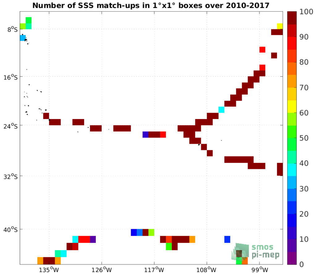
Figure 4: Number of SSS match-ups between TSG (GOSUD-Sailing-ship) SSS and the SMOS SSS L2Q v331 - 0.25 Deg (CATDS-CPDC) SSS product for the OTT zone Pi-MEP region over 1°x1° boxes and for the full satellite product period.
