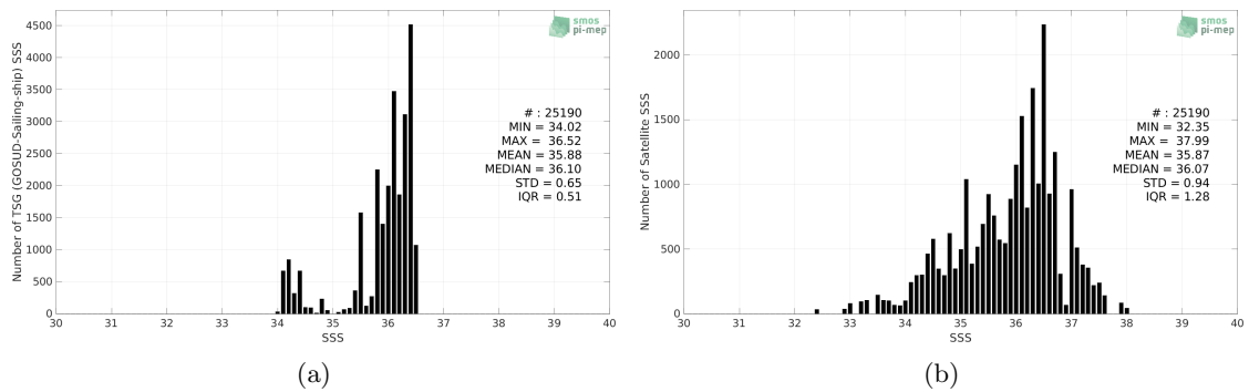
Figure 2: Histograms of SSS from TSG (GOSUD-Sailing-ship) (a) and SMOS SSS L2Q v331 - 0.25 Deg (CATDS-CPDC) (b) considering all match-up pairs per bins of 0.1 over the OTT zone Pi-MEP region and for the full satellite product period.
