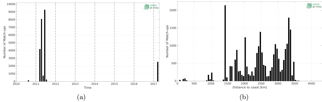
Figure 1: Number of match-ups between TSG (GOSUD-Sailing-ship) and SMOS SSS L2Q v331 - 0.25 Deg (CATDS-CPDC) SSS as a function of time (a) and as function of the distance to coast (b) over the OTT zone Pi-MEP region and for the full satellite product period.
