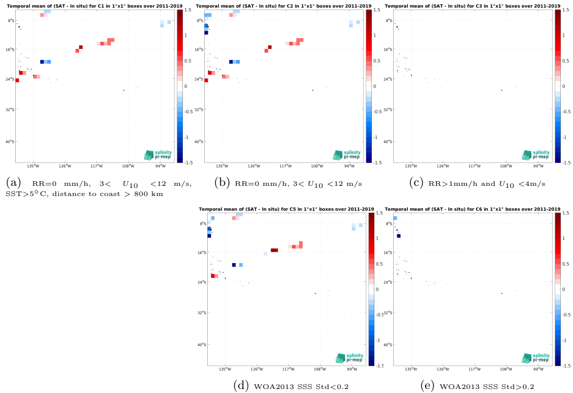
Figure 12: Temporal mean gridded over spatial boxes of size 1^\circ \times 1^\circ of \Delta SSS (SMOS SSS L2Q v331 - 0.25 Deg (CATDS-CPDC) - TSG (GOSUD-Research-vessel)) for 5 different subdatasets corresponding to:RR=0 mm/h, 3 < U_{10} < 12 m/s, SST >5^\circ\text{C} , distance to coast > 800 km (a), RR=0 mm/h, 3 < U_{10} < 12 m/s (b), RR >1 mm/h and U_{10} < 4 m/s (c), WOA2013 SSS Std <0.2 (d), WOA2013 SSS Std >0.2 (e).
