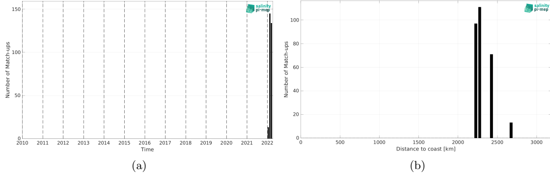
Figure 1: Number of match-ups between Saildrone and SMOS SSS L2Q v331 - 0.25 Deg (CATDS-CPDC) SSS as a function of time (a) and as function of the distance to coast (b) over the OTT zone Pi-MEP region and for the full satellite product period.
