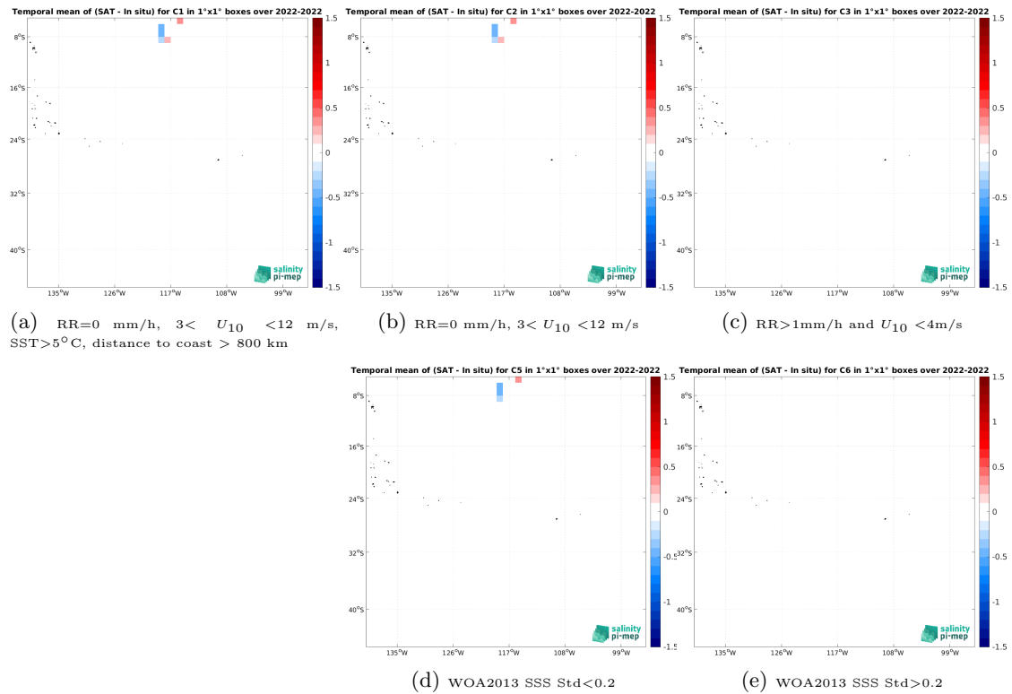
Figure 12: Temporal mean gridded over spatial boxes of size 1^\circ \times 1^\circ of \Delta SSS (SMOS SSS L2Q v331 - 0.25 Deg (CATDS-CPDC) - Saildrone) for 5 different subdatasets corresponding to:RR=0 mm/h, 3 < U_{10} < 12 m/s, SST >5^\circ C, distance to coast > 800 km (a), RR=0 mm/h, 3 < U_{10} < 12 m/s (b), RR >1 mm/h and U_{10} < 4 m/s (c), WOA2013 SSS Std <0.2 (d), WOA2013 SSS Std >0.2 (e).
