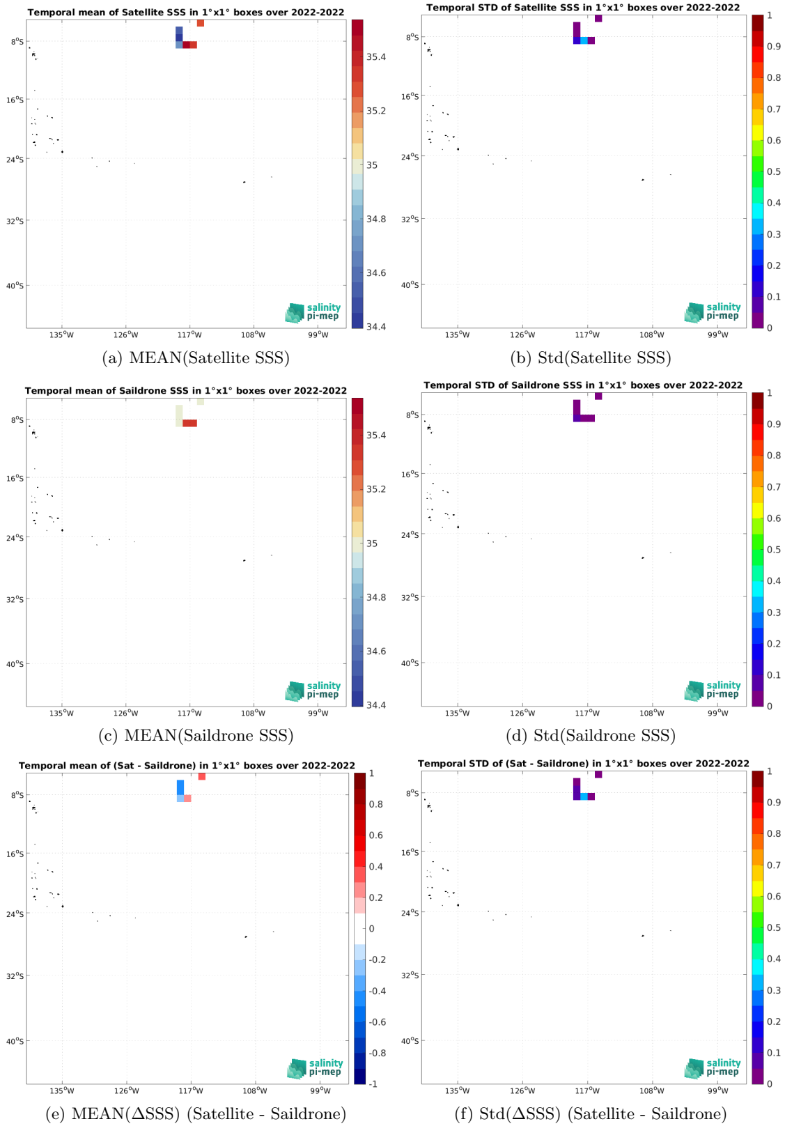
Figure 6: Temporal mean (left) and Std (right) of SSS from SMOS SSS L2Q v331 - 0.25 Deg (CATDS-CPDC) (top), Saildrone (middle), and of \Delta SSS (Satellite - Saildrone). Only match-up pairs are used to generate these maps.
