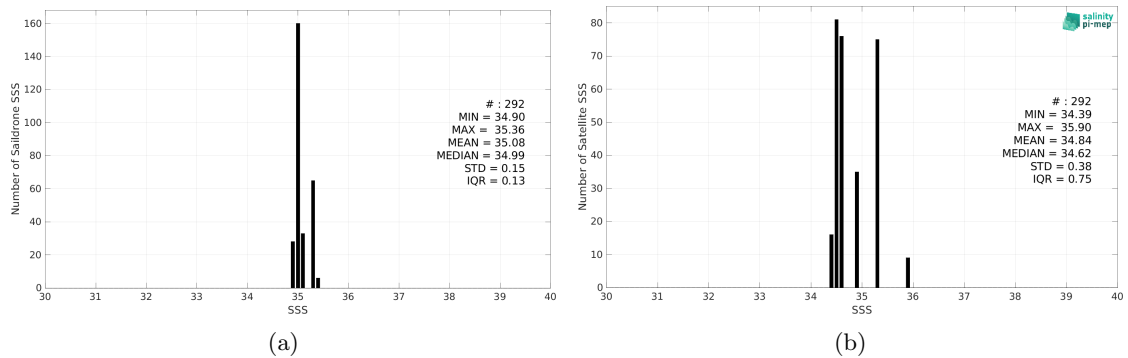
Figure 2: Histograms of SSS from Saildrone (a) and SMOS SSS L2Q v331 - 0.25 Deg (CATDS-CPDC) (b) considering all match-up pairs per bins of 0.1 over the OTT zone Pi-MEP region and for the full satellite product period.
