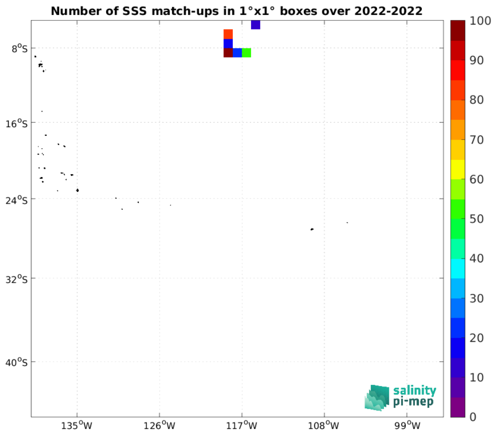
Figure 4: Number of SSS match-ups between Saildrone SSS and the SMOS SSS L2Q v331 - 0.25 Deg (CATDS-CPDC) SSS product for the OTT zone Pi-MEP region over 1^\circ \times 1^\circ boxes and for the full satellite product period.
