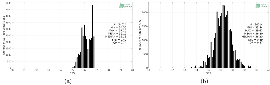
Figure 2: Histograms of SSS from Surface drifters (a) and SMOS SSS L2Q v331 - 0.25 Deg (CATDS-CPDC) (b) considering all match-up pairs per bins of 0.1 over the OTT zone Pi-MEP region and for the full satellite product period.
