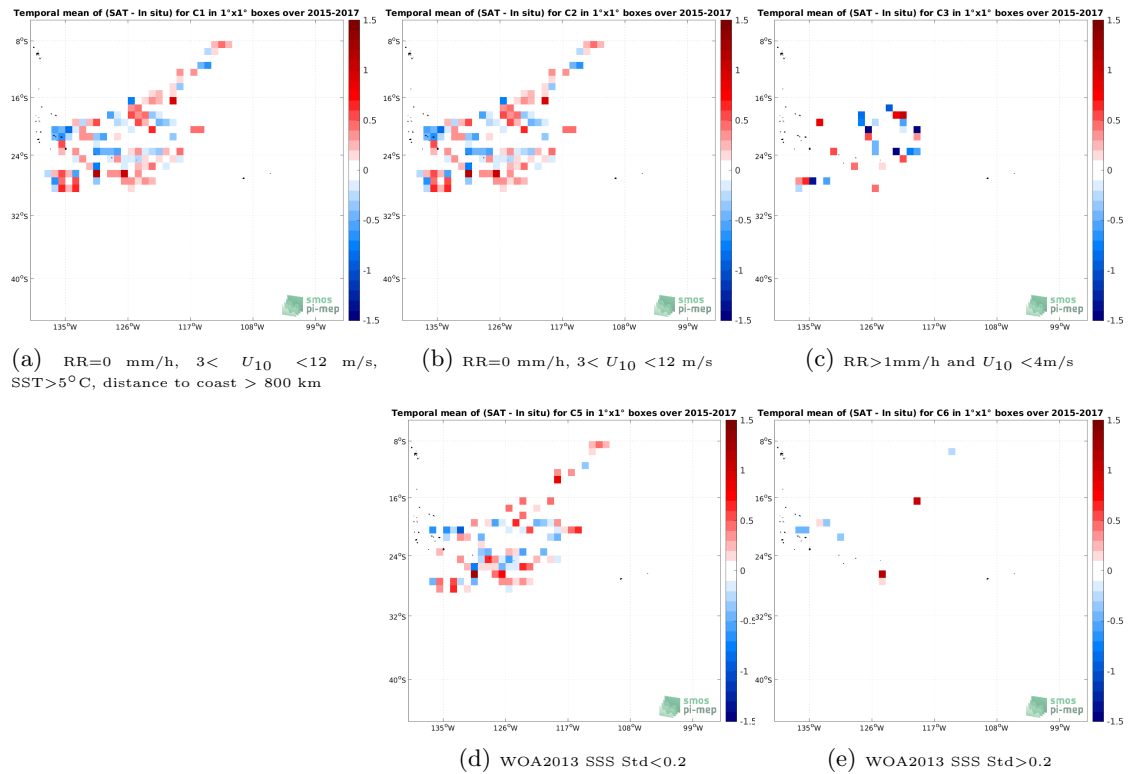
Figure 11: Temporal mean gridded over spatial boxes of size 1^\circ \times 1^\circ of \Delta SSS (SMOS SSS L2Q v331 - 0.25 Deg (CATDS-CPDC) - Surface drifters) for 5 different subdatasets corresponding to: RR=0 mm/h, 3 < U_{10} < 12 m/s, SST > 5^\circ C, distance to coast > 800 km (a), RR=0 mm/h, 3 < U_{10} < 12 m/s (b), RR > 1 mm/h and U_{10} < 4 m/s (c), WOA2013 SSS Std < 0.2 (d), WOA2013 SSS Std > 0.2 (e).
