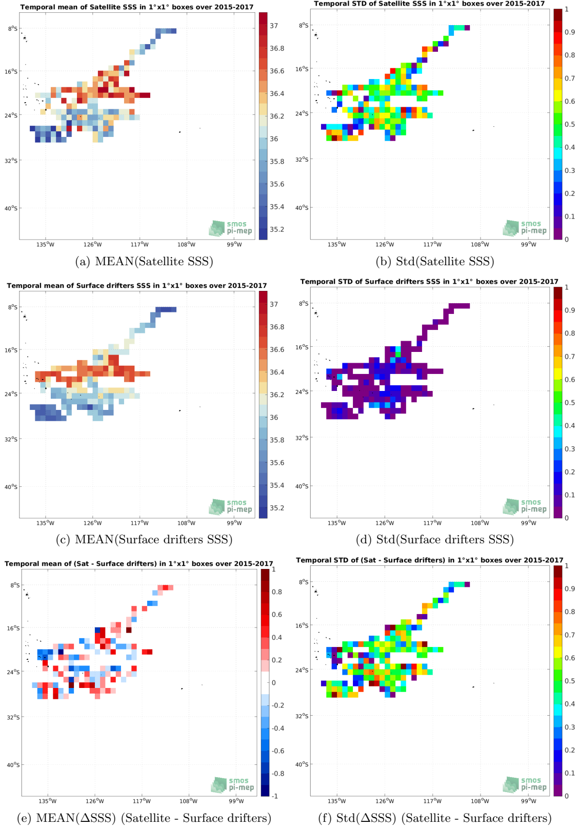
Figure 5: Temporal mean (left) and Std (right) of SSS from SMOS SSS L2Q v331 - 0.25 Deg (CATDS-CPDC) (top), Surface drifters (middle), and of \Delta SSS (Satellite - Surface drifters). Only match-up pairs are used to generate these maps.
