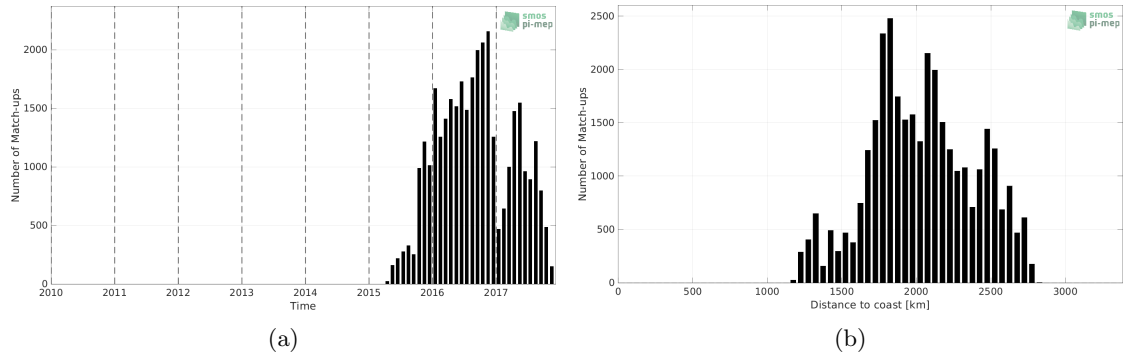
Figure 1: Number of match-ups between Surface drifters and SMOS SSS L2Q v331 - 0.25 Deg (CATDS-CPDC) SSS as a function of time (a) and as function of the distance to coast (b) over the OTT zone Pi-MEP region and for the full satellite product period.
