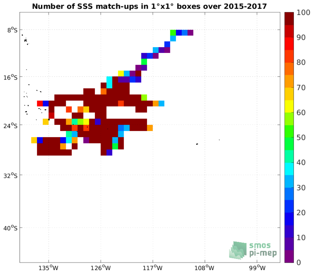
Figure 3: Number of SSS match-ups between Surface drifters SSS and the SMOS SSS L2Q v331 - 0.25 Deg (CATDS-CPDC) SSS product for the OTT zone Pi-MEP region over 1°x1° boxes and for the full satellite product period.
