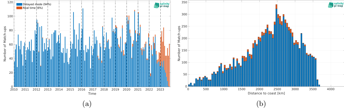
Figure 1: Number of match-ups between Argo and SMOS SSS L2Q v331 - 0.25 Deg (CATDS-CPDC) SSS as a function of time (a) and as function of the distance to coast (b) over the OTT zone Pi-MEP region and for the full satellite product period.
