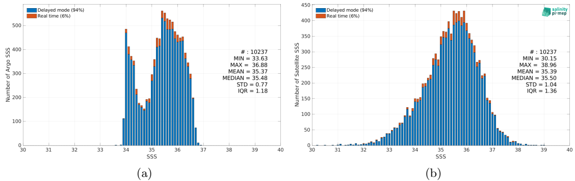
Figure 2: Histograms of SSS from Argo (a) and SMOS SSS L2Q v331 - 0.25 Deg (CATDS-CPDC) (b) considering all match-up pairs per bins of 0.1 over the OTT zone Pi-MEP region and for the full satellite product period.
