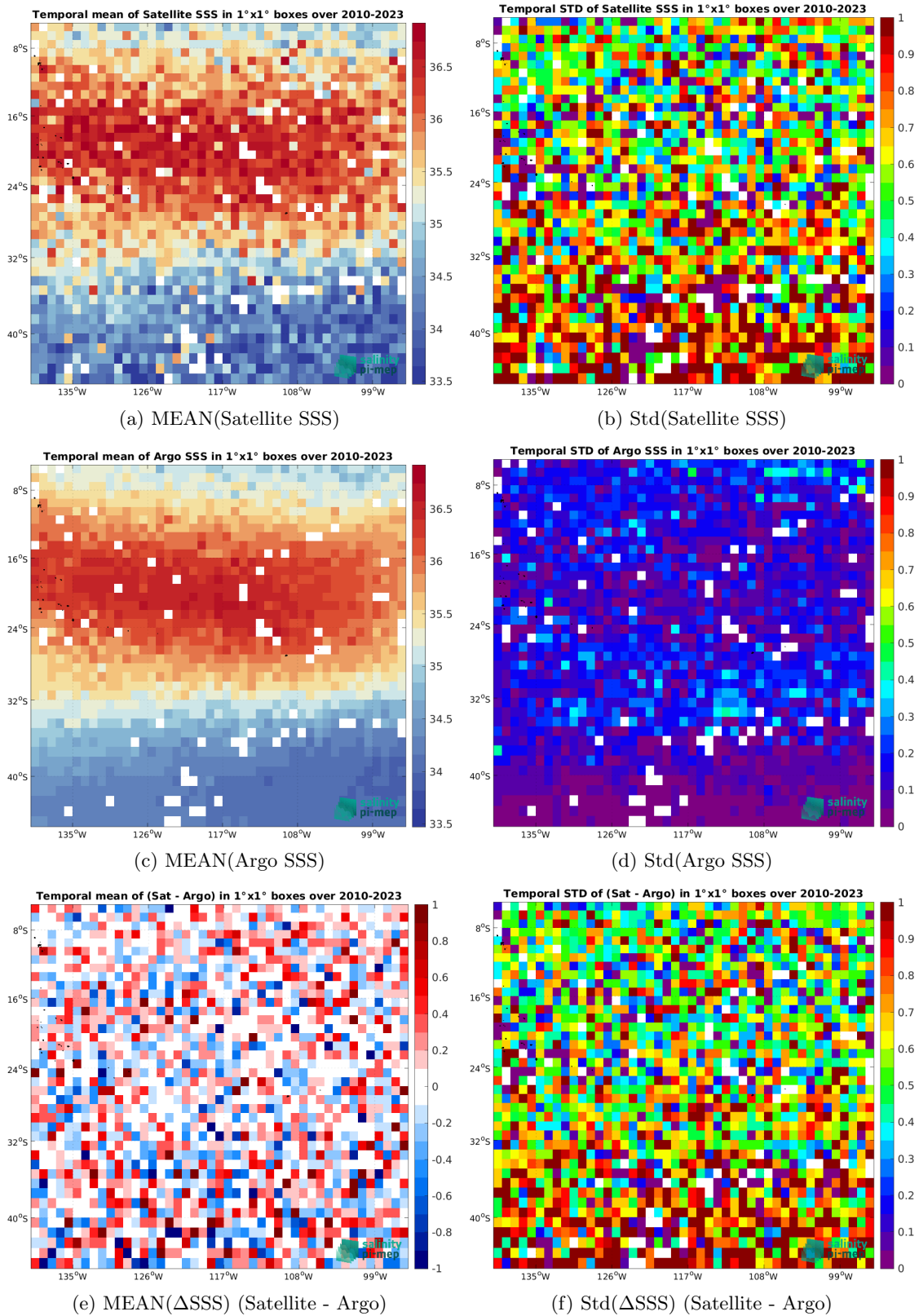
Figure 6: Temporal mean (left) and Std (right) of SSS from SMOS SSS L2Q v331 - 0.25 Deg (CATDS-CPDC) (top), Argo (middle), and of \Delta SSS (Satellite - Argo). Only match-up pairs are used to generate these maps.
