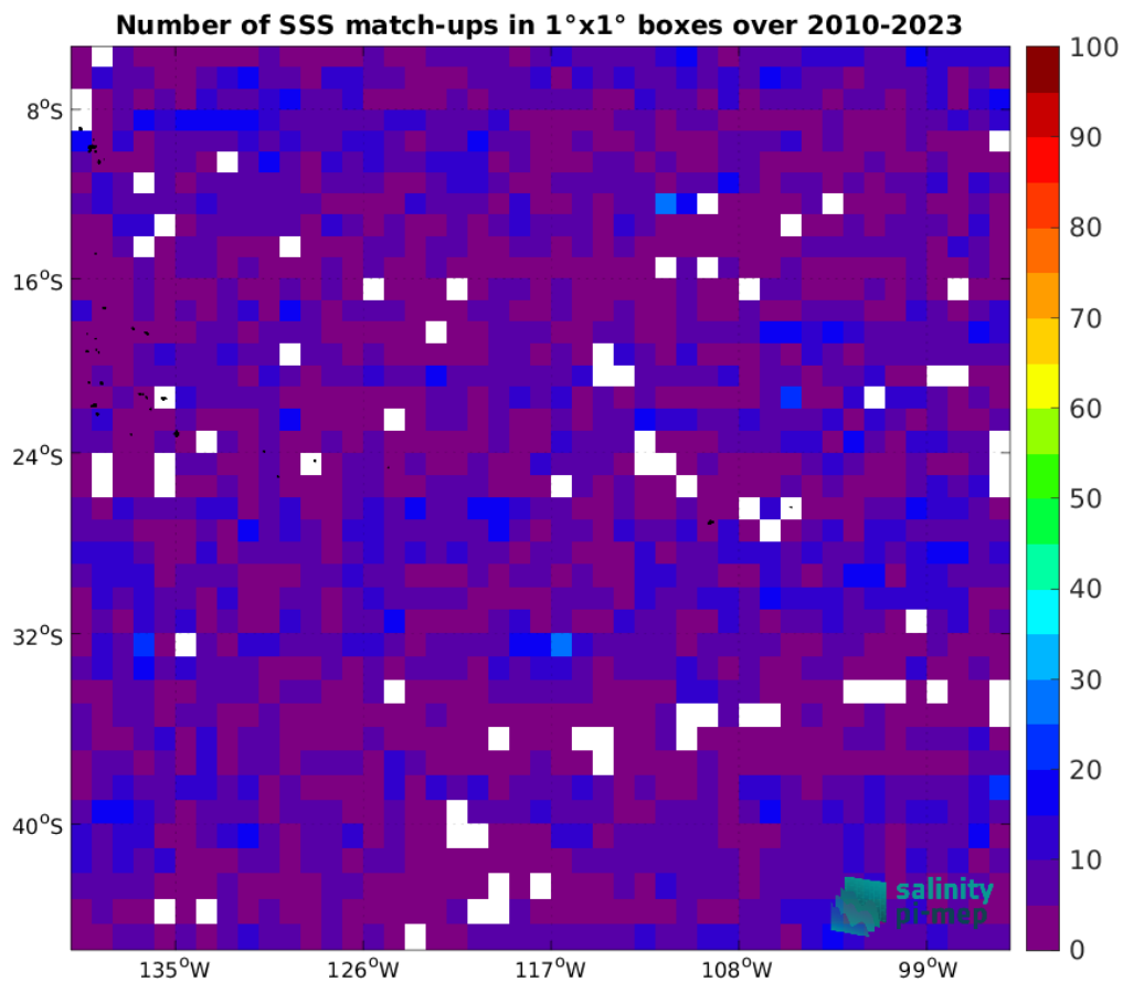
Figure 4: Number of SSS match-ups between Argo SSS and the SMOS SSS L2Q v331 - 0.25 Deg (CATDS-CPDC) SSS product for the OTT zone Pi-MEP region over 1°x1° boxes and for the full satellite product period.
