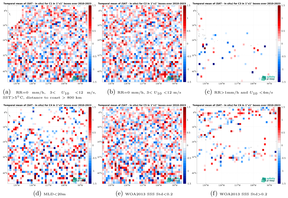
Figure 12: Temporal mean gridded over spatial boxes of size 1^\circ \times 1^\circ of \Delta SSS (SMOS SSS L2Q v331 - 0.25 Deg (CATDS-CPDC) - Argo) for 6 different subdatasets corresponding to:RR=0 mm/h, 3 < U_{10} < 12 m/s, SST >5^\circ C, distance to coast > 800 km (a), RR=0 mm/h, 3 < U_{10} < 12 m/s (b), RR >1 mm/h and U_{10} < 4 m/s (c),MLD <20 m (d),WOA2013 SSS Std <0.2 (e),WOA2013 SSS Std >0.2 (f).
