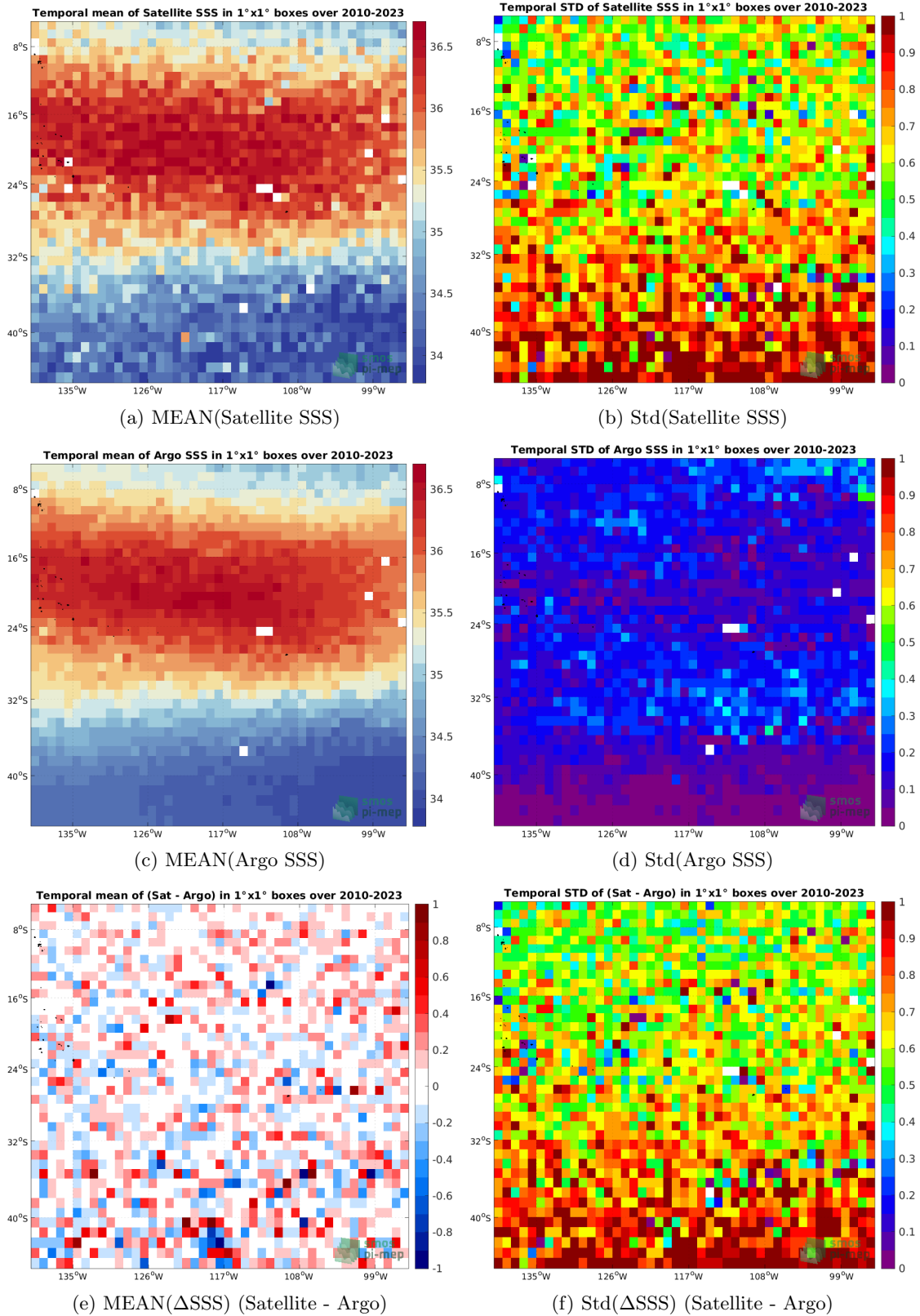
Figure 6: Temporal mean (left) and Std (right), of SSS from SMOS SSS L2Q v331 - 0.25 Deg (CATDS-CPDC) (top), Argo (middle), and of \Delta SSS (Satellite - Argo). Only match-up pairs are used to generate these maps.
