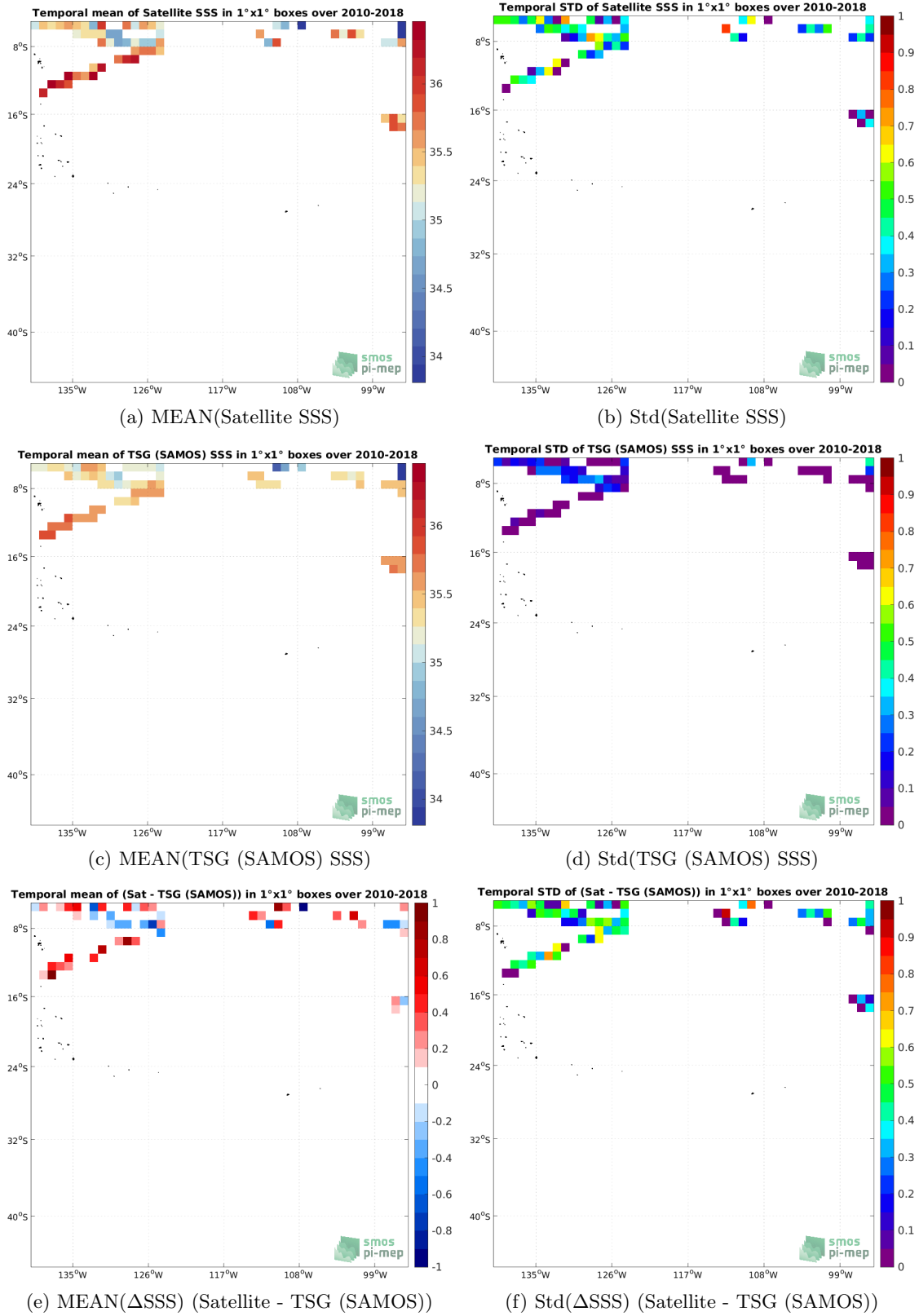
Figure 6: Temporal mean (left) and Std (right), of SSS from SMOS SSS L2Q v330 - 0.25 Deg (CATDS-CPDC) (top), TSG (SAMOS) (middle), and of \Delta SSS (Satellite - TSG (SAMOS)). Only match-up pairs are used to generate these maps.
