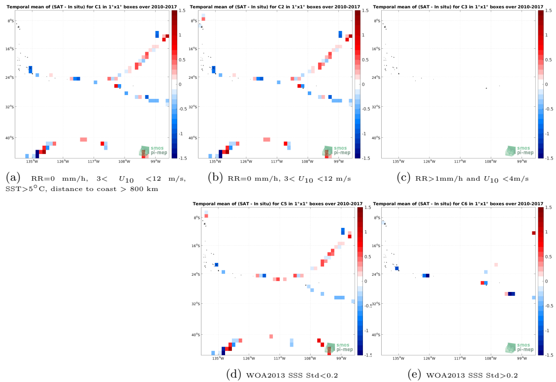
Figure 12: Temporal mean gridded over spatial boxes of size 1^\circ \times 1^\circ of \Delta\text{SSS} (SMOS SSS L2Q v330 - 0.25 Deg (CATDS-CPDC) - TSG (GOSUD-Sailing-ship)) for 5 different subdatasets corresponding to:RR=0 mm/h, 3 < U_{10} < 12 m/s, SST >5^\circ\text{C} , distance to coast > 800 km (a), RR=0 mm/h, 3 < U_{10} < 12 m/s (b), RR >1 mm/h and U_{10} < 4 m/s (c), WOA2013 SSS Std <0.2 (d), WOA2013 SSS Std >0.2 (e).
