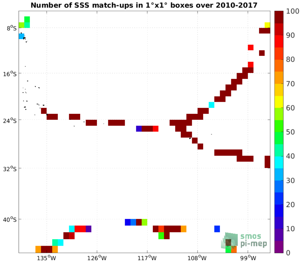
Figure 4: Number of SSS match-ups between TSG (GOSUD-Sailing-ship) SSS and the SMOS SSS L2Q v330 - 0.25 Deg (CATDS-CPDC) SSS product for the OTT zone Pi-MEP region over 1°x1° boxes and for the full satellite product period.
