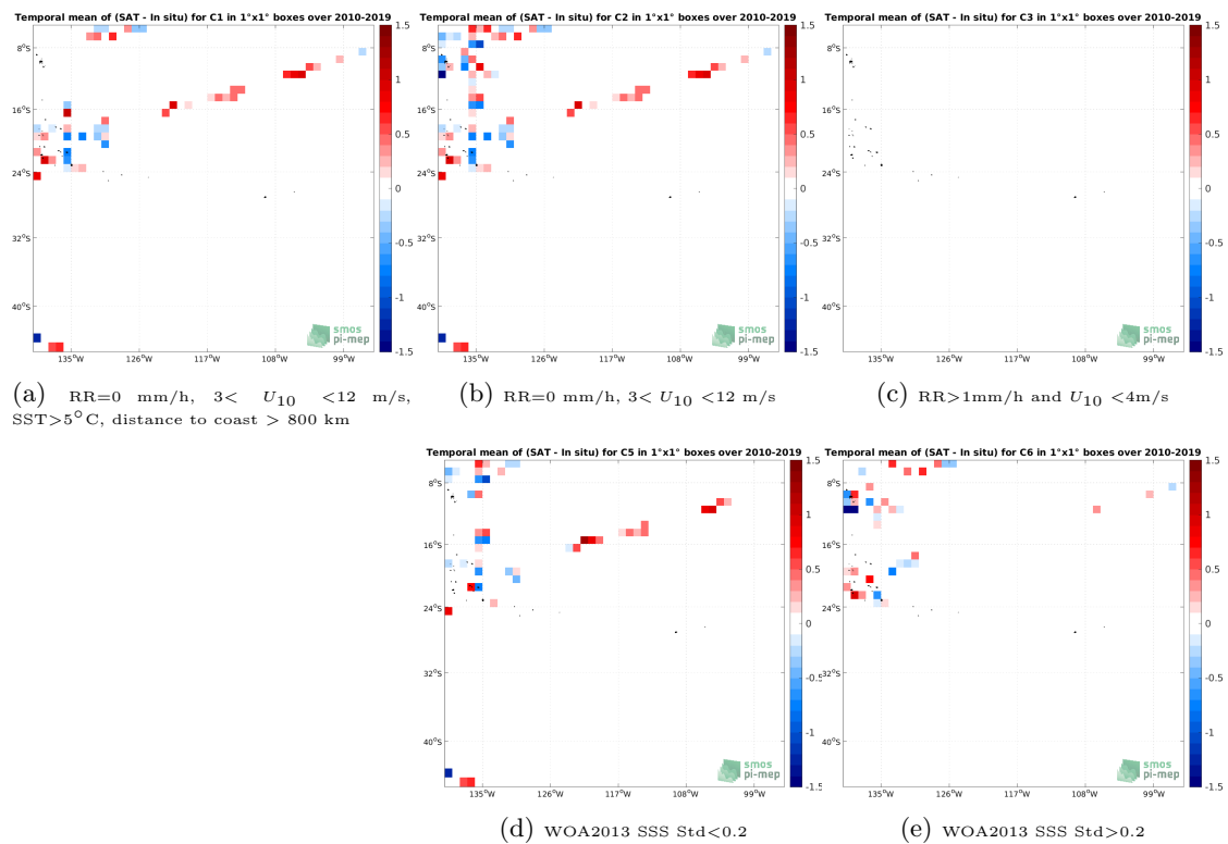
Figure 12: Temporal mean gridded over spatial boxes of size 1^\circ \times 1^\circ of \Delta SSS (SMOS SSS L2Q v330 - 0.25 Deg (CATDS-CPDC) - TSG (GOSUD-Research-vessel)) for 5 different subdatasets corresponding to:RR=0 mm/h, 3 < U_{10} < 12 m/s, SST >5^\circ C, distance to coast > 800 km (a), RR=0 mm/h, 3 < U_{10} < 12 m/s (b), RR >1 mm/h and U_{10} < 4 m/s (c), WOA2013 SSS Std <0.2 (d), WOA2013 SSS Std >0.2 (e).
