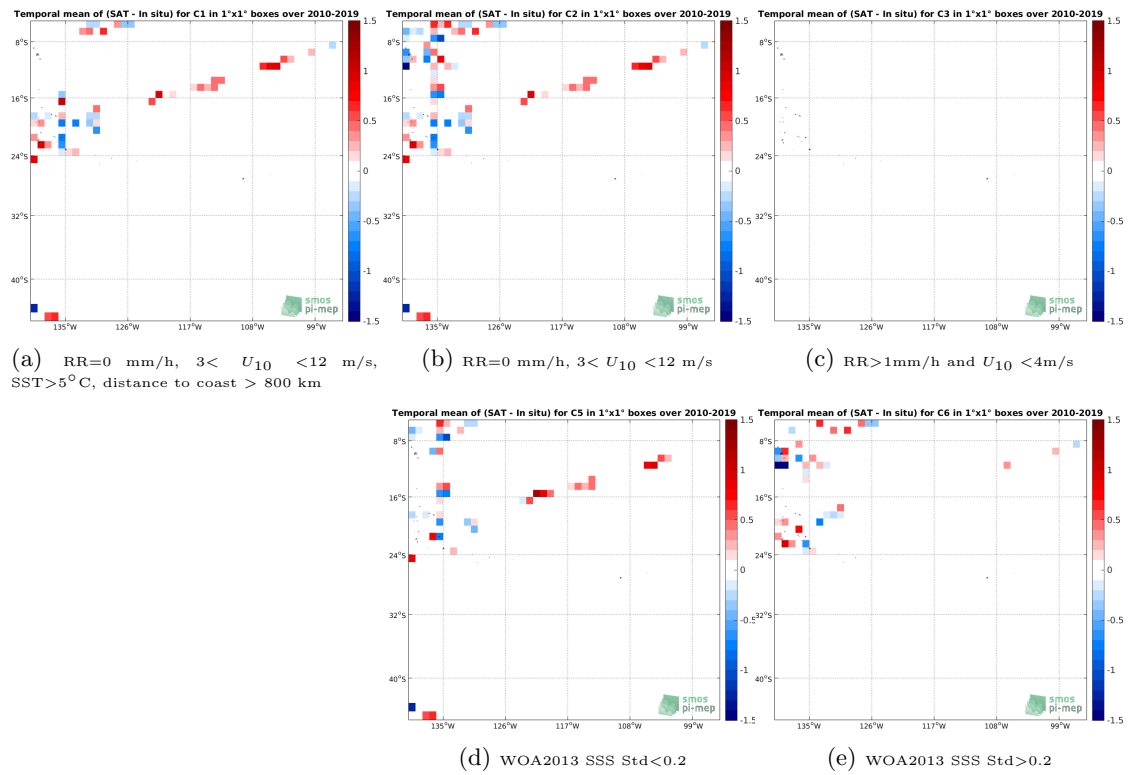
Figure 12: Temporal mean gridded over spatial boxes of size 1^\circ \times 1^\circ of \Delta\text{SSS} (SMOS SSS L2Q v330 - 0.25 Deg (CATDS-CPDC) - TSG (GOSUD-Research-vessel)) for 5 different subdatasets corresponding to:RR=0 mm/h, 3 < U_{10} < 12 m/s, SST>5°C, distance to coast > 800 km (a), RR=0 mm/h, 3 < U_{10} < 12 m/s (b), RR>1mm/h and U_{10} < 4 m/s (c), WOA2013 SSS Std<0.2 (d), WOA2013 SSS Std>0.2 (e).
