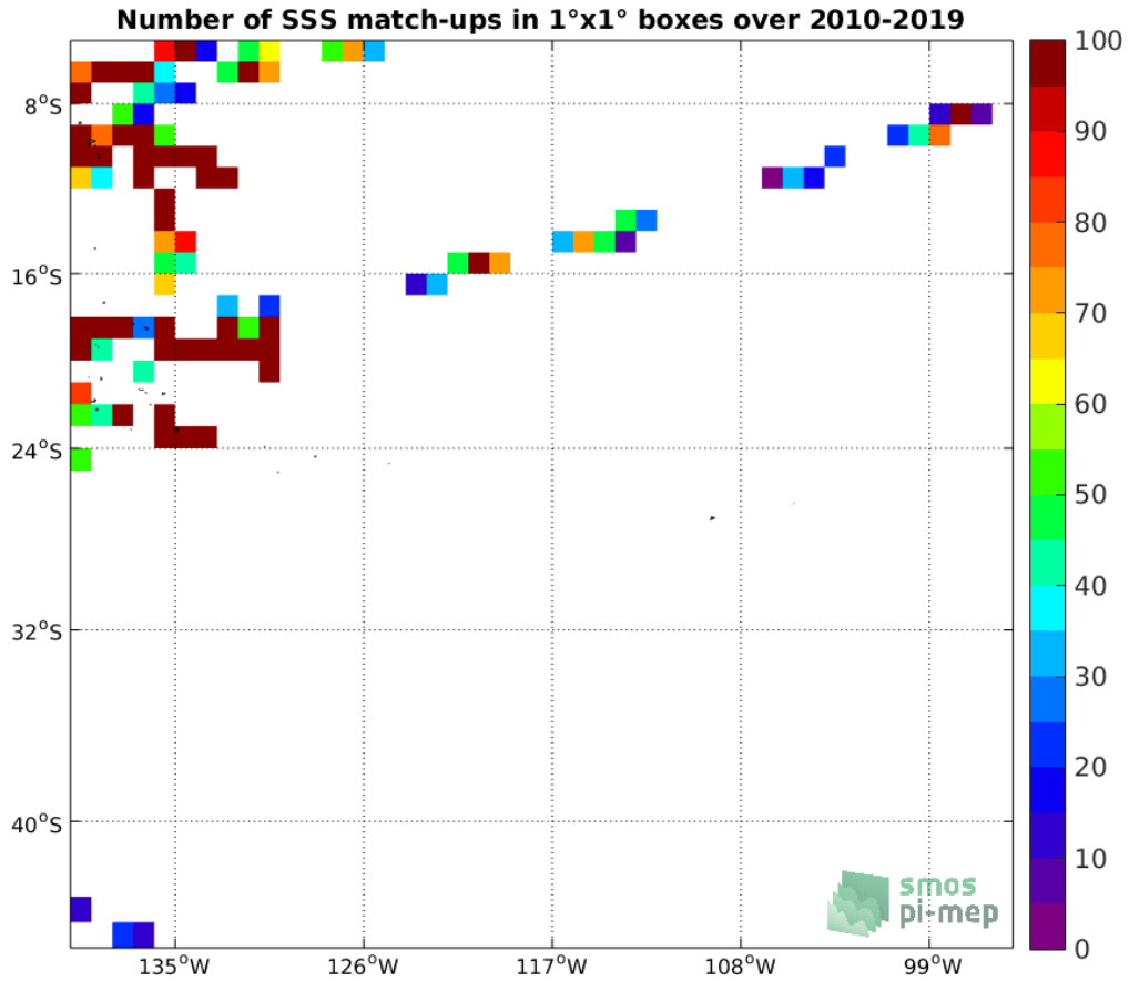
Figure 4: Number of SSS match-ups between TSG (GOSUD-Research-vessel) SSS and the SMOS SSS L2Q v330 - 0.25 Deg (CATDS-CPDC) SSS product for the OTT zone Pi-MEP region over 1^\circ \times 1^\circ boxes and for the full satellite product period.
