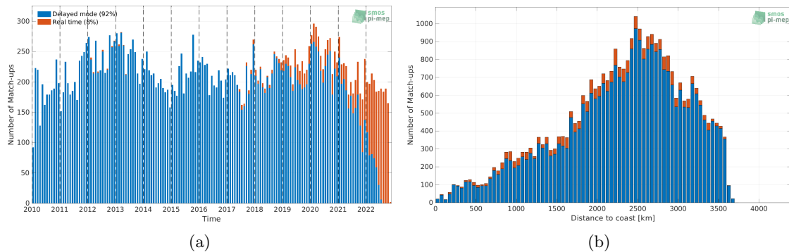
Figure 1: Number of match-ups between Argo and SMOS SSS L2Q v330 - 0.25 Deg (CATDS-CPDC) SSS as a function of time (a) and as function of the distance to coast (b) over the OTT zone Pi-MEP region and for the full satellite product period.
