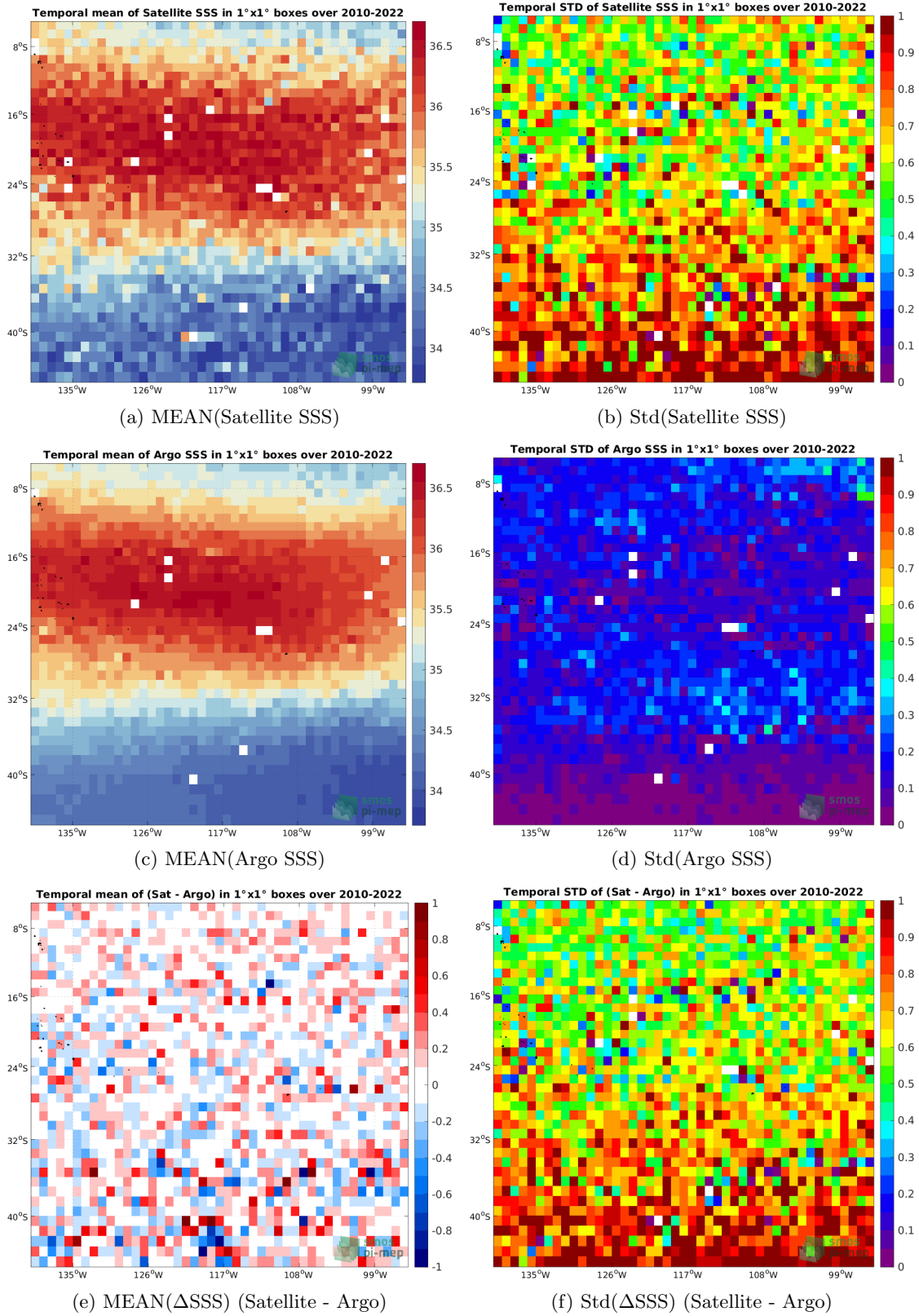
Figure 6: Temporal mean (left) and Std (right), of SSS from SMOS SSS L2Q v330 - 0.25 Deg (CATDS-CPDC) (top), Argo (middle), and of \Delta SSS (Satellite - Argo). Only match-up pairs are used to generate these maps.
