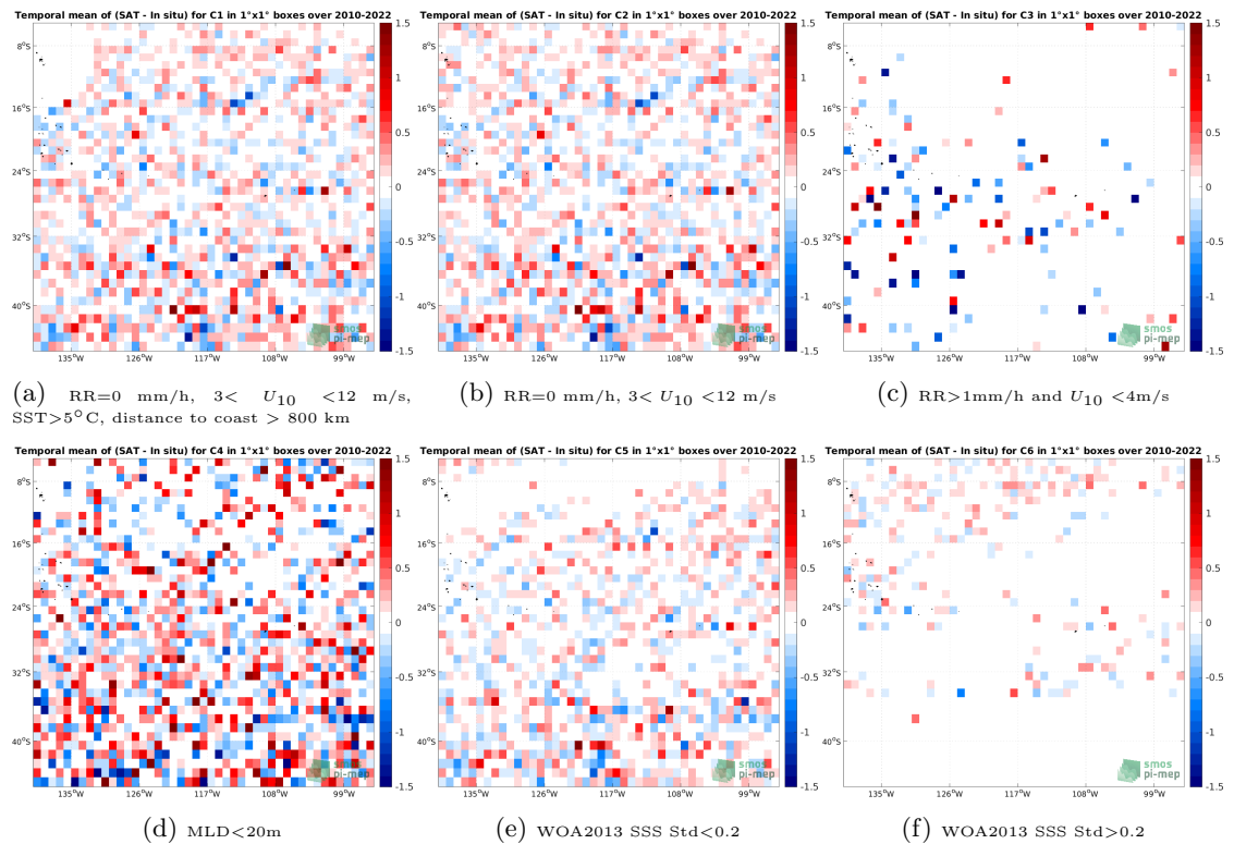
Figure 12: Temporal mean gridded over spatial boxes of size 1^\circ \times 1^\circ of \Delta SSS (SMOS SSS L2Q v330 - 0.25 Deg (CATDS-CPDC) - Argo) for 6 different subdatasets corresponding to:RR=0 mm/h, 3 < U_{10} < 12 m/s, SST >5^\circ C, distance to coast > 800 km (a), RR=0 mm/h, 3 < U_{10} < 12 m/s (b), RR >1 mm/h and U_{10} < 4 m/s (c),MLD <20 m (d),WOA2013 SSS Std <0.2 (e),WOA2013 SSS Std >0.2 (f).
