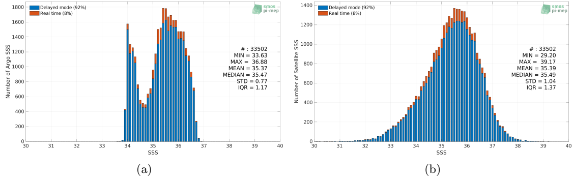
Figure 2: Histograms of SSS from Argo (a) and SMOS SSS L2Q v330 - 0.25 Deg (CATDS-CPDC) (b) considering all match-up pairs per bins of 0.1 over the OTT zone Pi-MEP region and for the full satellite product period.
