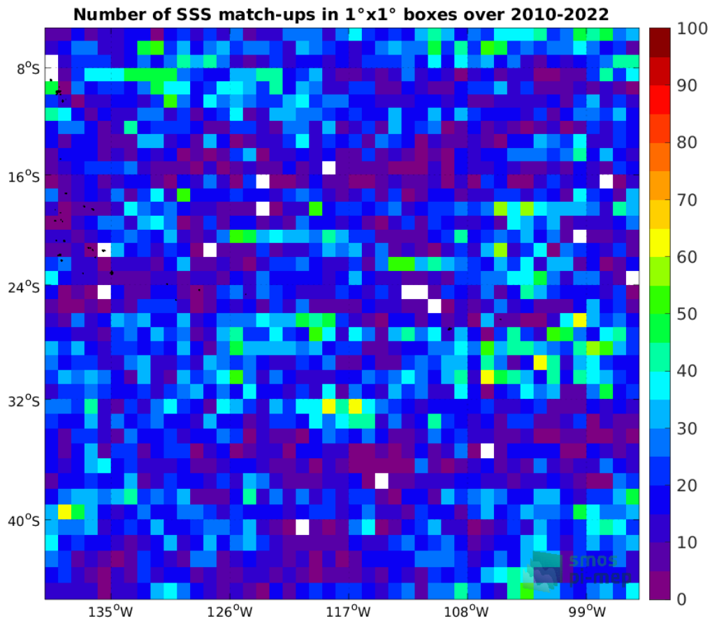
Figure 4: Number of SSS match-ups between Argo SSS and the SMOS SSS L2Q v330 - 0.25 Deg (CATDS-CPDC) SSS product for the OTT zone Pi-MEP region over 1°x1° boxes and for the full satellite product period.
