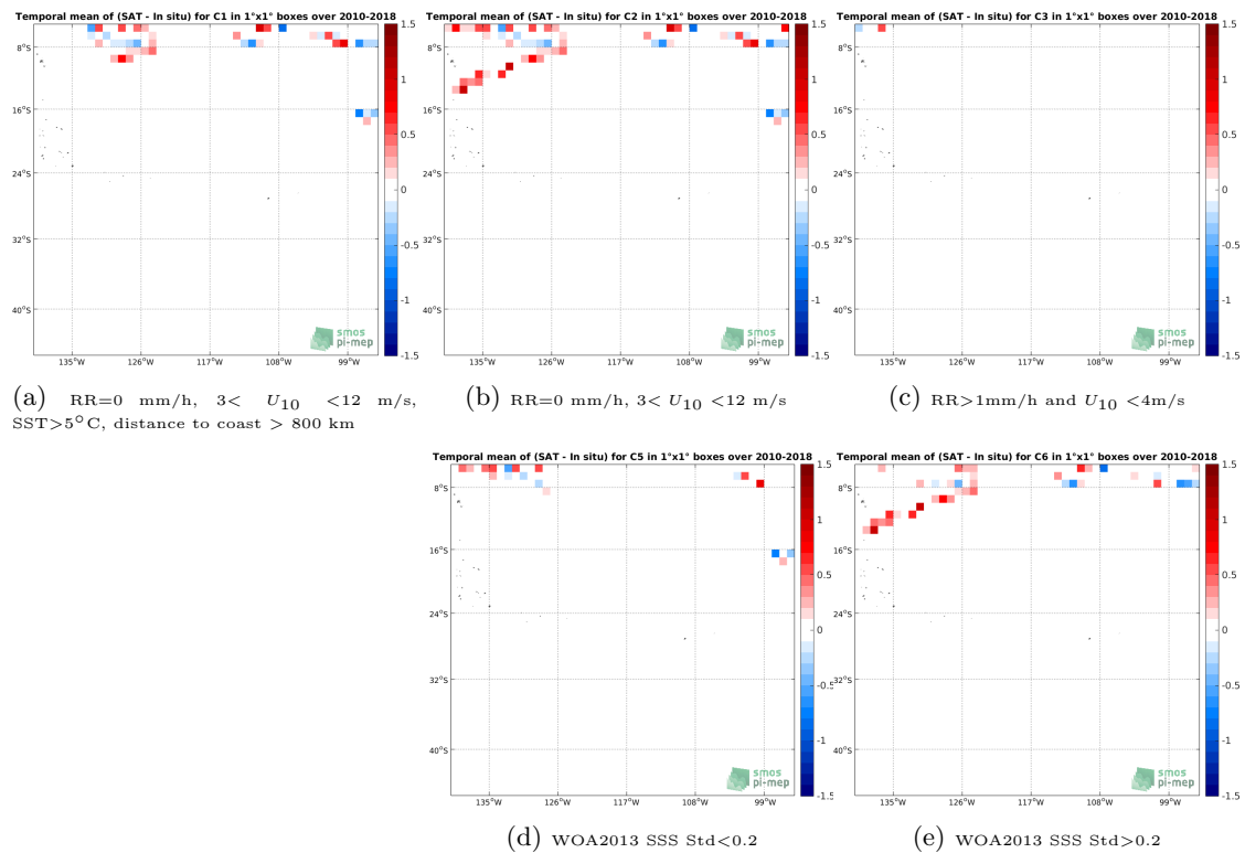
Figure 12: Temporal mean gridded over spatial boxes of size 1^\circ \times 1^\circ of \Delta\text{SSS} (SMOS SSS L2Q v321 - 0.25 Deg (CATDS-CPDC) - TSG (SAMOS)) for 5 different subdatasets corresponding to:RR=0 mm/h, 3 < U_{10} < 12 m/s, SST >5^\circ\text{C} , distance to coast > 800 km (a), RR=0 mm/h, 3 < U_{10} < 12 m/s (b), RR >1 mm/h and U_{10} < 4 m/s (c), WOA2013 SSS Std <0.2 (d), WOA2013 SSS Std >0.2 (e).
