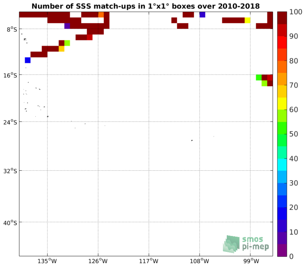
Figure 4: Number of SSS match-ups between TSG (SAMOS) SSS and the SMOS SSS L2Q v321 - 0.25 Deg (CATDS-CPDC) SSS product for the OTT zone Pi-MEP region over 1^{\circ} \times 1^{\circ} boxes and for the full satellite product period.
