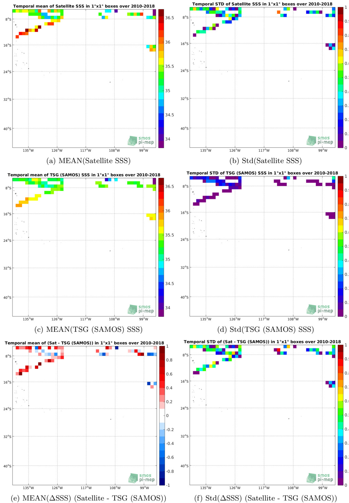
Figure 6: Temporal mean (left) and Std (right) of SSS from SMOS SSS L2Q v321 - 0.25 Deg (CATDS-CPDC) (top), TSG (SAMOS) (middle), and of \Delta SSS (Satellite - TSG (SAMOS)). Only match-up pairs are used to generate these maps.
