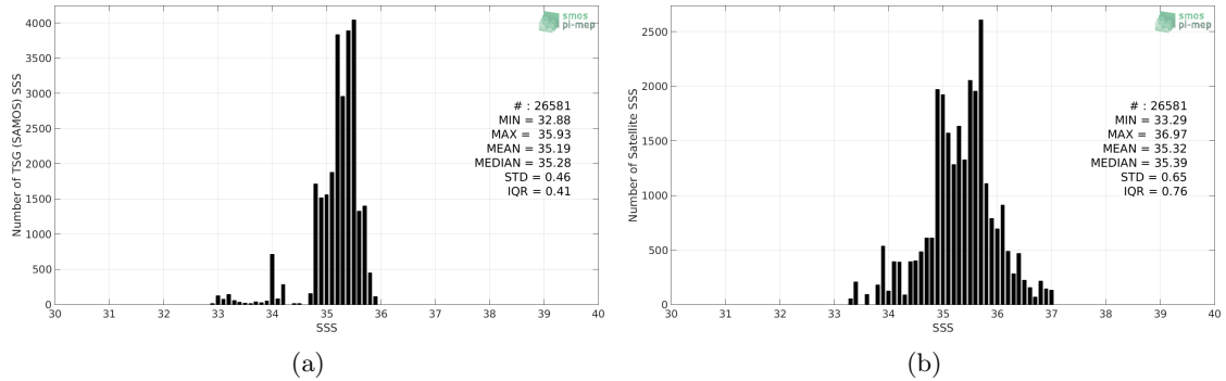
Figure 2: Histograms of SSS from TSG (SAMOS) (a) and SMOS SSS L2Q v321 - 0.25 Deg (CATDS-CPDC) (b) considering all match-up pairs per bins of 0.1 over the OTT zone Pi-MEP region and for the full satellite product period.
