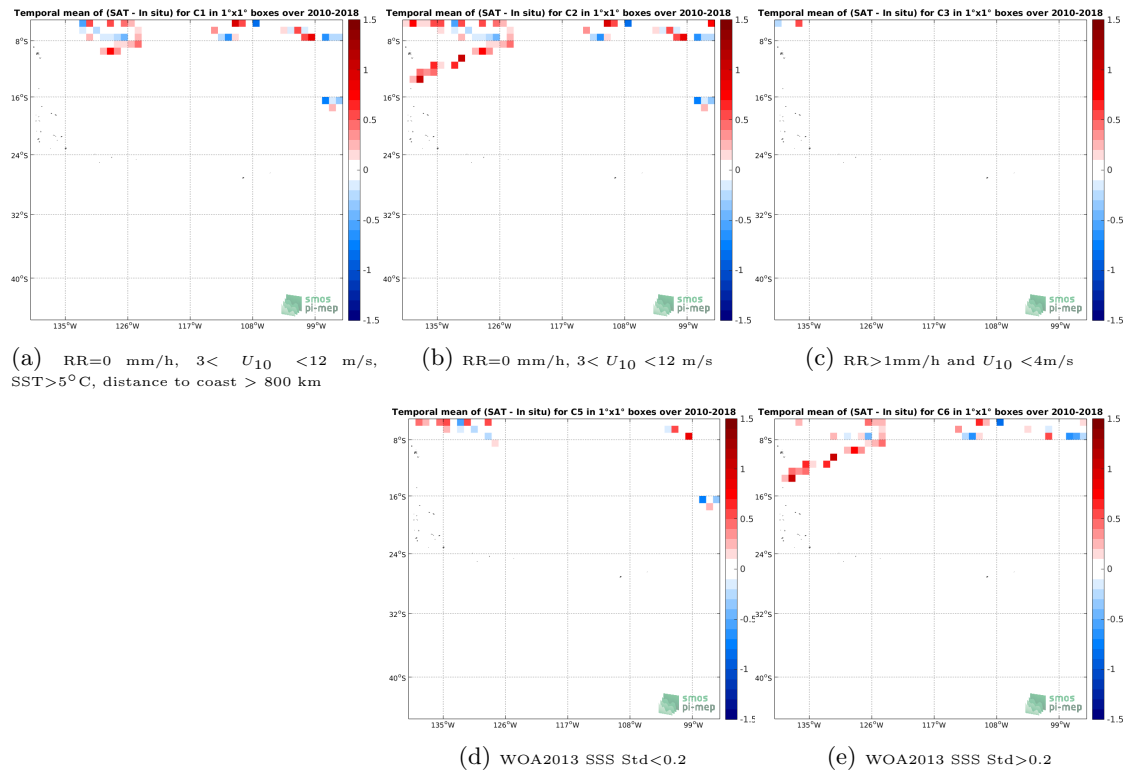
Figure 12: Temporal mean gridded over spatial boxes of size 1^\circ \times 1^\circ of \Delta SSS (SMOS SSS L2Q v321 - 0.25 Deg (CATDS-CPDC) - TSG (SAMOS)) for 5 different subdatasets corresponding to:RR=0 mm/h, 3 < U_{10} < 12 m/s, SST >5^\circ\text{C} , distance to coast > 800 km (a), RR=0 mm/h, 3 < U_{10} < 12 m/s (b), RR >1 mm/h and U_{10} < 4 m/s (c), WOA2013 SSS Std <0.2 (d), WOA2013 SSS Std >0.2 (e).
