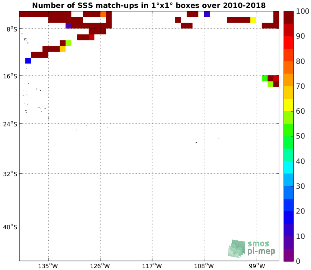
Figure 4: Number of SSS match-ups between TSG (SAMOS) SSS and the SMOS SSS L2Q v321 - 0.25 Deg (CATDS-CPDC) SSS product for the OTT zone Pi-MEP region over 1^\circ \times 1^\circ boxes and for the full satellite product period.
