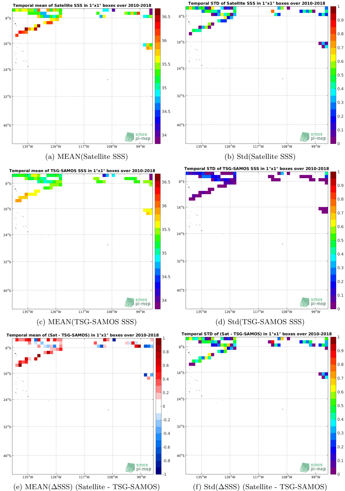
Figure 6: Temporal mean (left) and Std (right) of SSS from SMOS L2Q v321 - 0.25 Deg (CATDS-CPDC) (top), TSG-SAMOS (middle), and of \Delta SSS (Satellite - TSG-SAMOS). Only match-up pairs are used to generate these maps.
