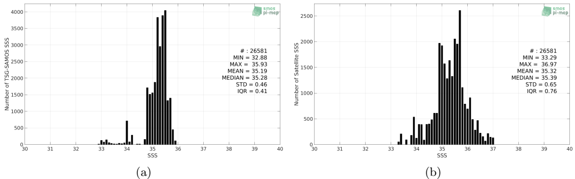
Figure 2: Histograms of SSS from TSG-SAMOS (a) and SMOS L2Q v321 - 0.25 Deg (CATDS-CPDC) (b) considering all match-up pairs per bins of 0.1 over the OTT zone Pi-MEP region and for the full satellite product period.
