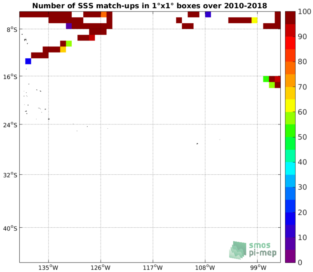
Figure 4: Number of SSS match-ups between TSG-SAMOS SSS and the SMOS L2Q v321 - 0.25 Deg (CATDS-CPDC) SSS product for the OTT zone Pi-MEP region over 1°x1° boxes and for the full satellite product period.
