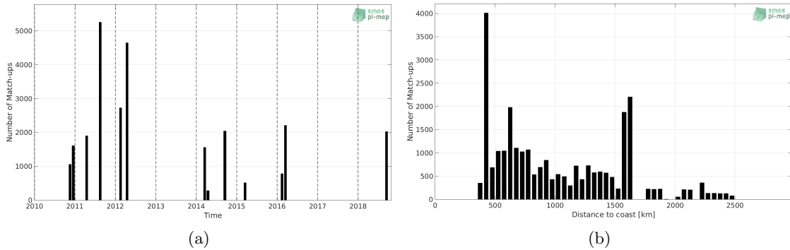
Figure 1: Number of match-ups between TSG-SAMOS and SMOS L2Q v321 - 0.25 Deg (CATDS-CPDC) SSS as a function of time (a) and as function of the distance to coast (b) over the OTT zone Pi-MEP region and for the full satellite product period.
