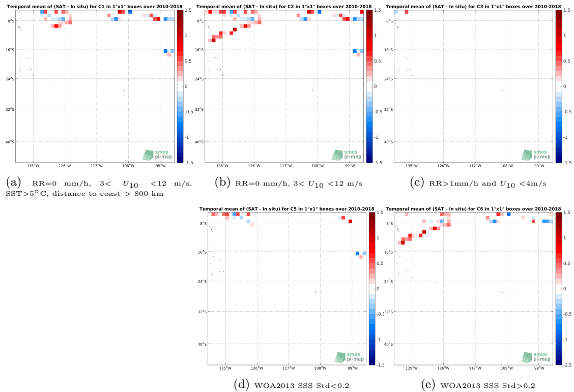
Figure 12: Temporal mean gridded over spatial boxes of size 1^\circ \times 1^\circ of \Delta SSS (SMOS L2Q v321 - 0.25 Deg (CATDS-CPDC) - TSG-SAMOS) for 5 different subdatasets corresponding to:RR=0 mm/h, 3 < U_{10} < 12 m/s, SST >5^\circ\text{C} , distance to coast > 800 km (a), RR=0 mm/h, 3 < U_{10} < 12 m/s (b), RR >1 mm/h and U_{10} < 4 m/s (c), WOA2013 SSS Std <0.2 (d), WOA2013 SSS Std >0.2 (e).
