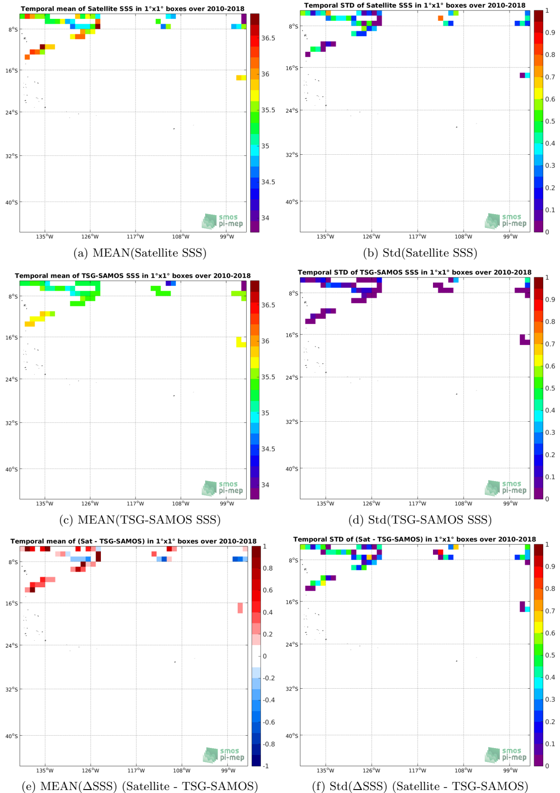
Figure 6: Temporal mean (left) and Std (right) of SSS from SMOS-L3-CATDS-CPDC-V321-L2Q (top), TSG-SAMOS (middle), and of \Delta SSS (Satellite - TSG-SAMOS). Only match-up pairs are used to generate these maps.
