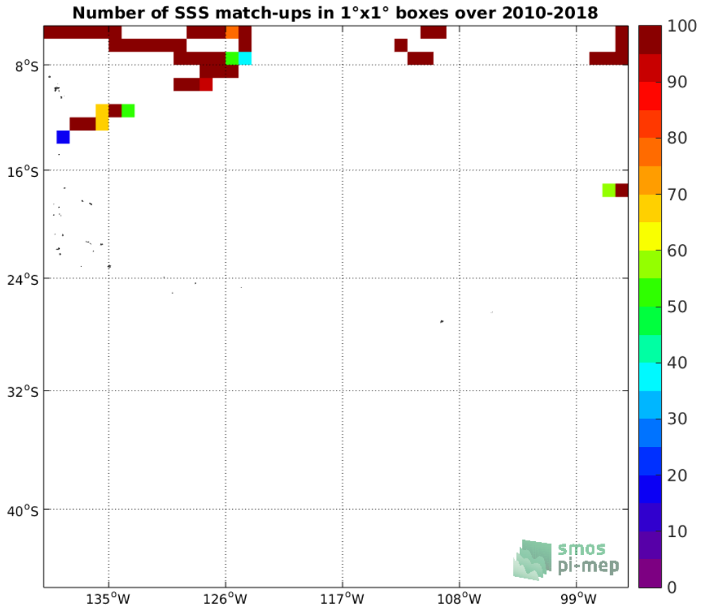
Figure 4: Number of SSS match-ups between TSG-SAMOS SSS and the SMOS-L3-CATDS-CPDC-V321-L2Q SSS product for the OTT zone Pi-MEP region over 1°x1° boxes and for the full satellite product period.
