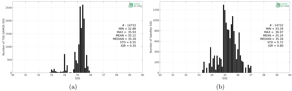
Figure 2: Histograms of SSS from TSG-SAMOS (a) and SMOS-L3-CATDS-CPDC-V321-L2Q (b) considering all match-up pairs per bins of 0.1 over the OTT zone Pi-MEP region and for the full satellite product period.
