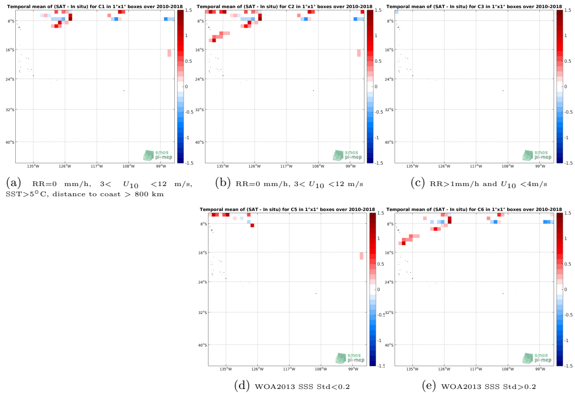
Figure 12: Temporal mean gridded over spatial boxes of size 1^\circ \times 1^\circ of \Delta SSS (SMOS-L3-CATDS-CPDC-V321-L2Q - TSG-SAMOS) for 5 different subdatasets corresponding to:RR=0 mm/h, 3 < U_{10} < 12 m/s, SST >5^\circ C, distance to coast > 800 km (a), RR=0 mm/h, 3 < U_{10} < 12 m/s (b), RR >1 mm/h and U_{10} < 4 m/s (c), WOA2013 SSS Std <0.2 (d), WOA2013 SSS Std >0.2 (e).
