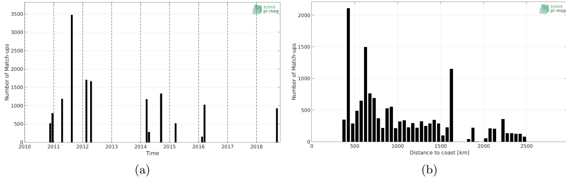
Figure 1: Number of match-ups between TSG-SAMOS and SMOS-L3-CATDS-CPDC-V321-L2Q SSS as a function of time (a) and as function of the distance to coast (b) over the OTT zone Pi-MEP region and for the full satellite product period.
