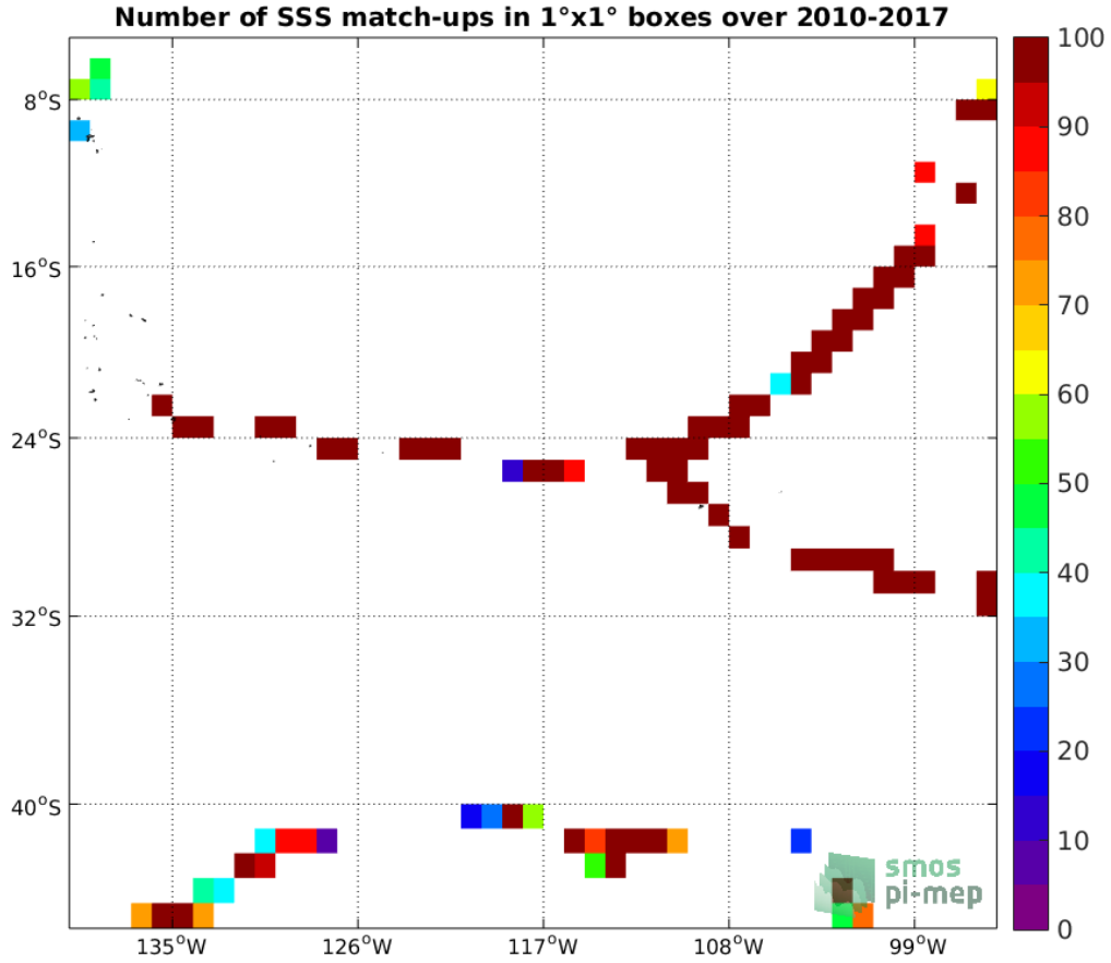
Figure 4: Number of SSS match-ups between TSG (GOSUD-Sailing-ship) SSS and the SMOS SSS L2Q v321 - 0.25 Deg (CATDS-CPDC) SSS product for the OTT zone Pi-MEP region over 1°x1° boxes and for the full satellite product period.
