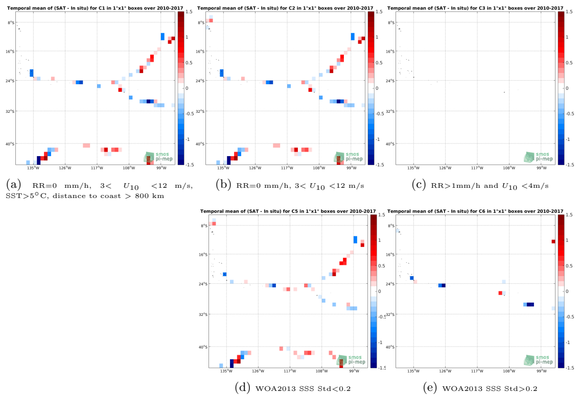
Figure 12: Temporal mean gridded over spatial boxes of size 1^\circ \times 1^\circ of \Delta SSS (SMOS L2Q v321 - 0.25 Deg (CATDS-CPDC) - TSG-GOSUD-Sailing-ship) for 5 different subdatasets corresponding to: RR=0 mm/h, 3 < U_{10} < 12 m/s, SST > 5^\circ C , distance to coast > 800 km (a), RR=0 mm/h, 3 < U_{10} < 12 m/s (b), RR > 1 mm/h and U_{10} < 4 m/s (c), WOA2013 SSS Std < 0.2 (d), WOA2013 SSS Std > 0.2 (e).
