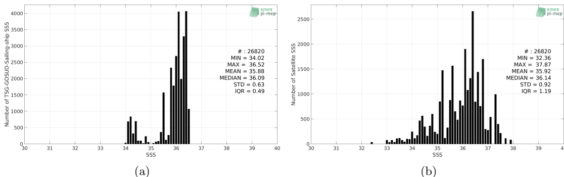
Figure 2: Histograms of SSS from TSG-GOSUD-Sailing-ship (a) and SMOS L2Q v321 - 0.25 Deg (CATDS-CPDC) (b) considering all match-up pairs per bins of 0.1 over the OTT zone Pi-MEP region and for the full satellite product period.
