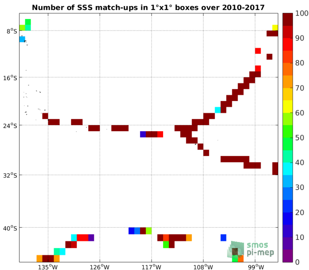
Figure 4: Number of SSS match-ups between TSG-GOSUD-Sailing-ship SSS and the SMOS L2Q v321 - 0.25 Deg (CATDS-CPDC) SSS product for the OTT zone Pi-MEP region over 1°x1° boxes and for the full satellite product period.
