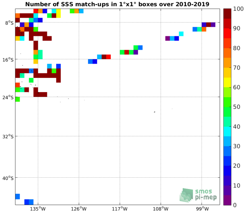
Figure 4: Number of SSS match-ups between TSG (GOSUD-Research-vessel) SSS and the SMOS SSS L2Q v321 - 0.25 Deg (CATDS-CPDC) SSS product for the OTT zone Pi-MEP region over 1^\circ \times 1^\circ boxes and for the full satellite product period.
